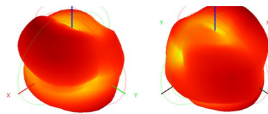
2500.0MHz Total, Eff: 9.3%
