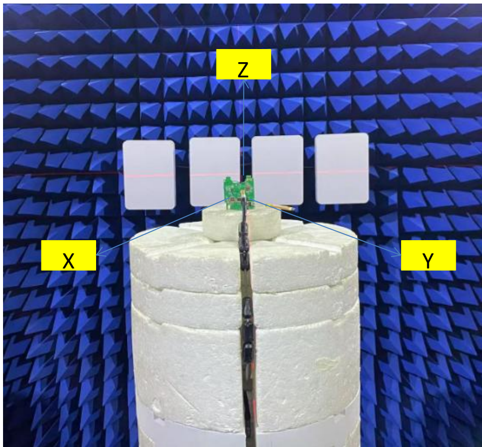
Testing environment
