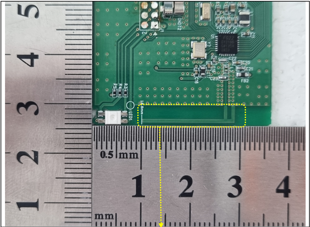
Zigbee Antenna
