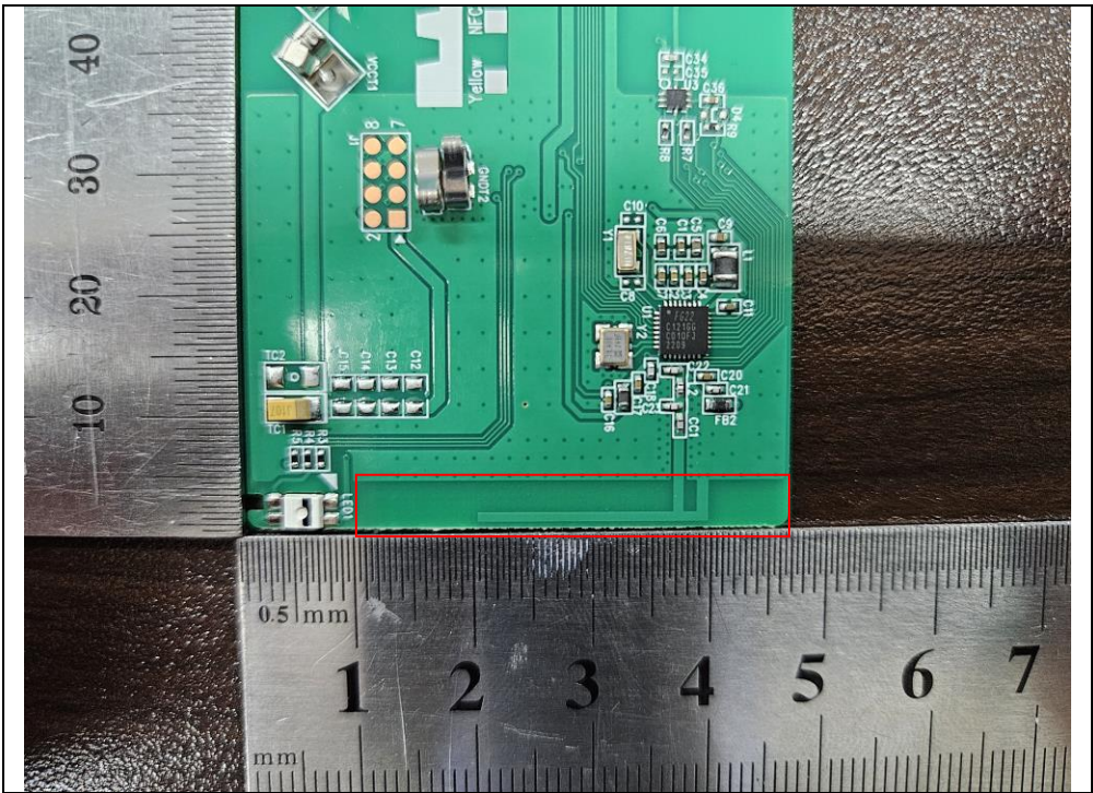
Zigbee Antenna
