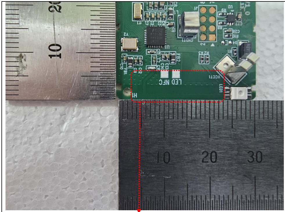
Zigbee Antenna
