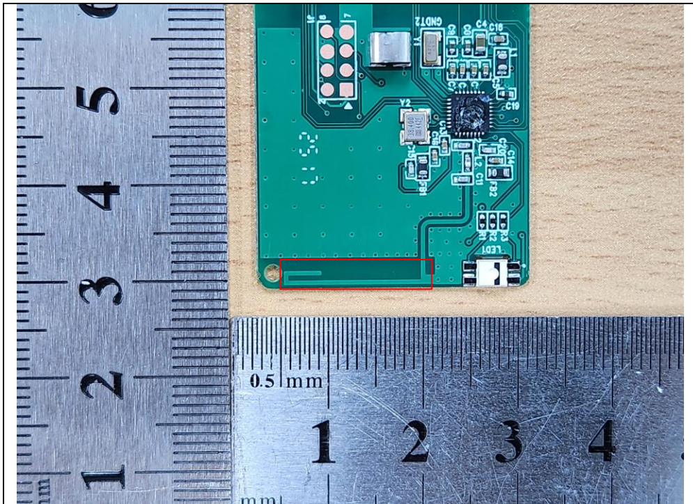
Zigbee Antenna
