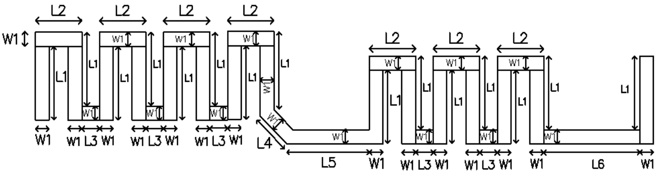
Figure 3:Antenna Dimensions
