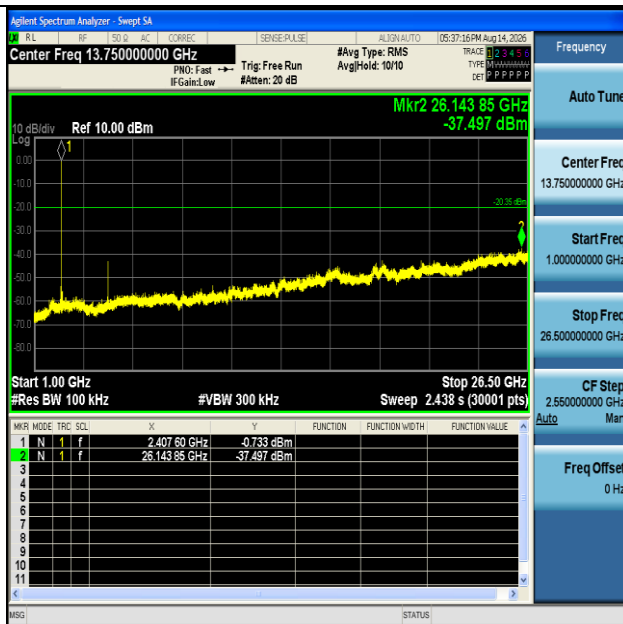
SRD-Ant1-2408-1000~26500-PASS
