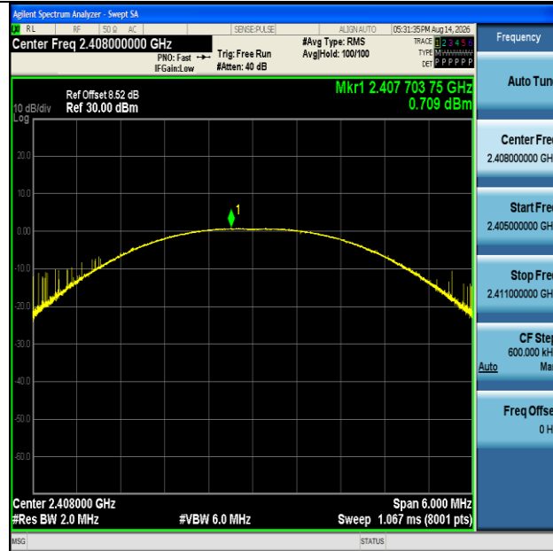
SRD-Ant1-2408-PASS
