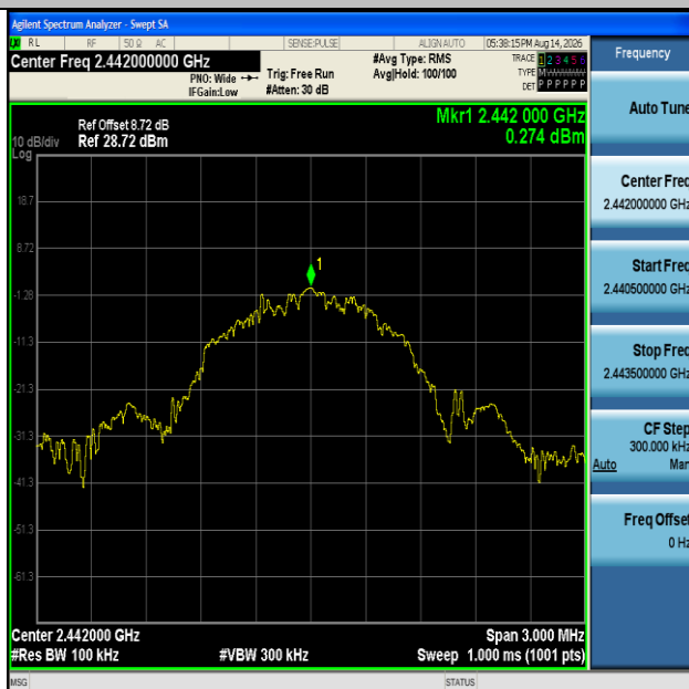
SRD-Ant1-2442-0~Reference-PASS
