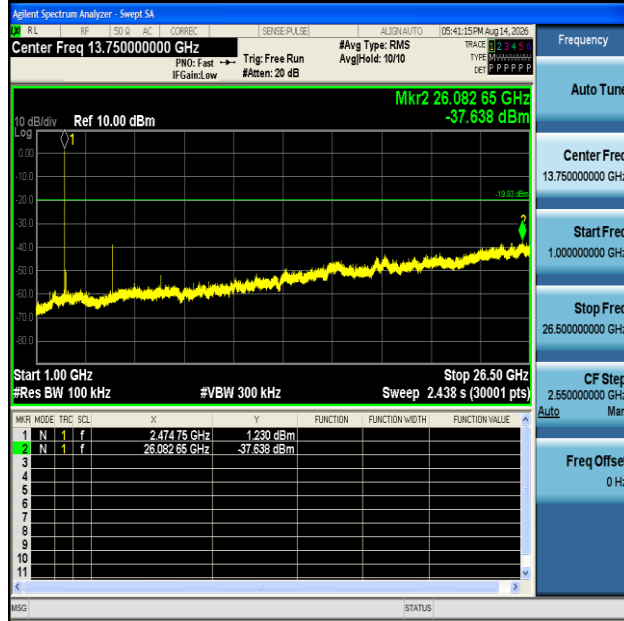
SRD-Ant1-2475-1000~26500-PASS
