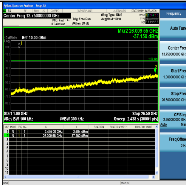
SRD-Ant1-2445-1000~26500-PASS
