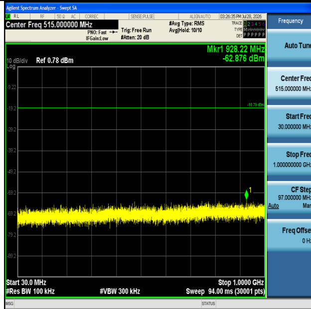
SRD-Ant1-2445-30~1000-PASS
