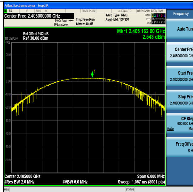
SRD-Ant1-2405-PASS
