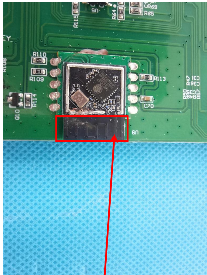
PCB Antenna
