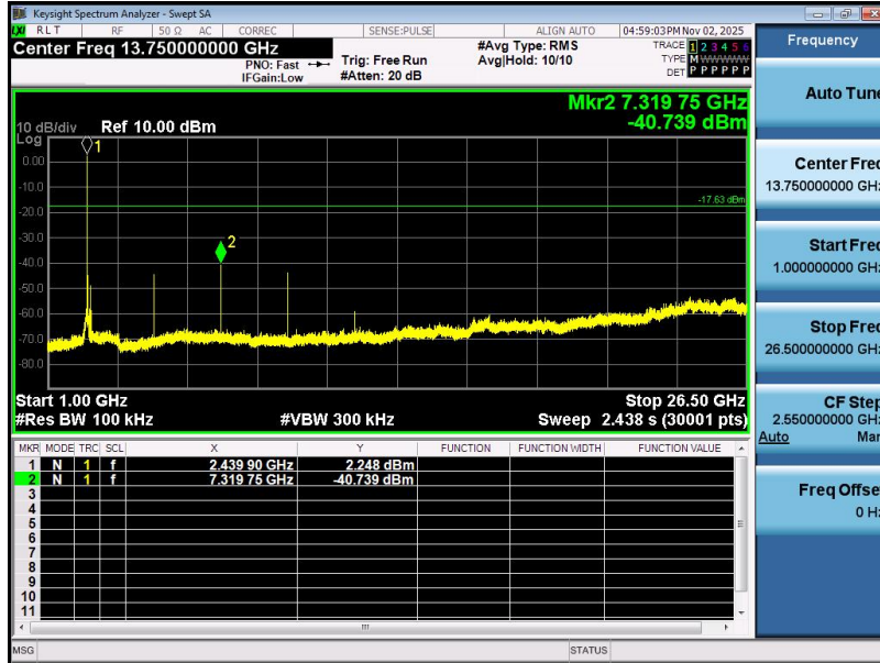
BLE_2M-Ant1-2440-1000~26500-PASS
