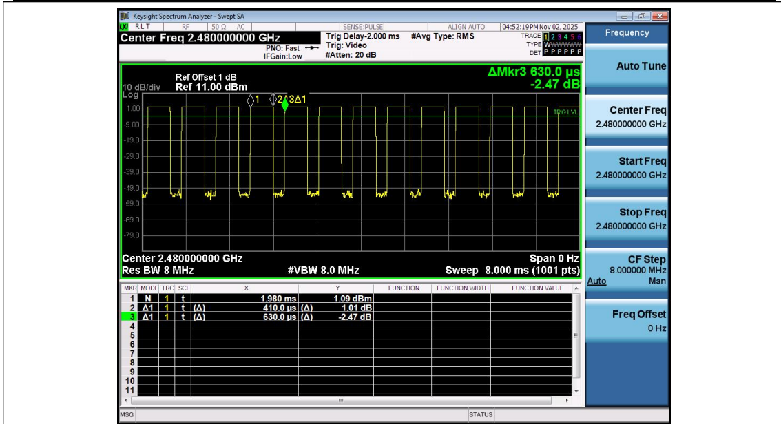
NTNV-BLE_1M-Ant1-2480
