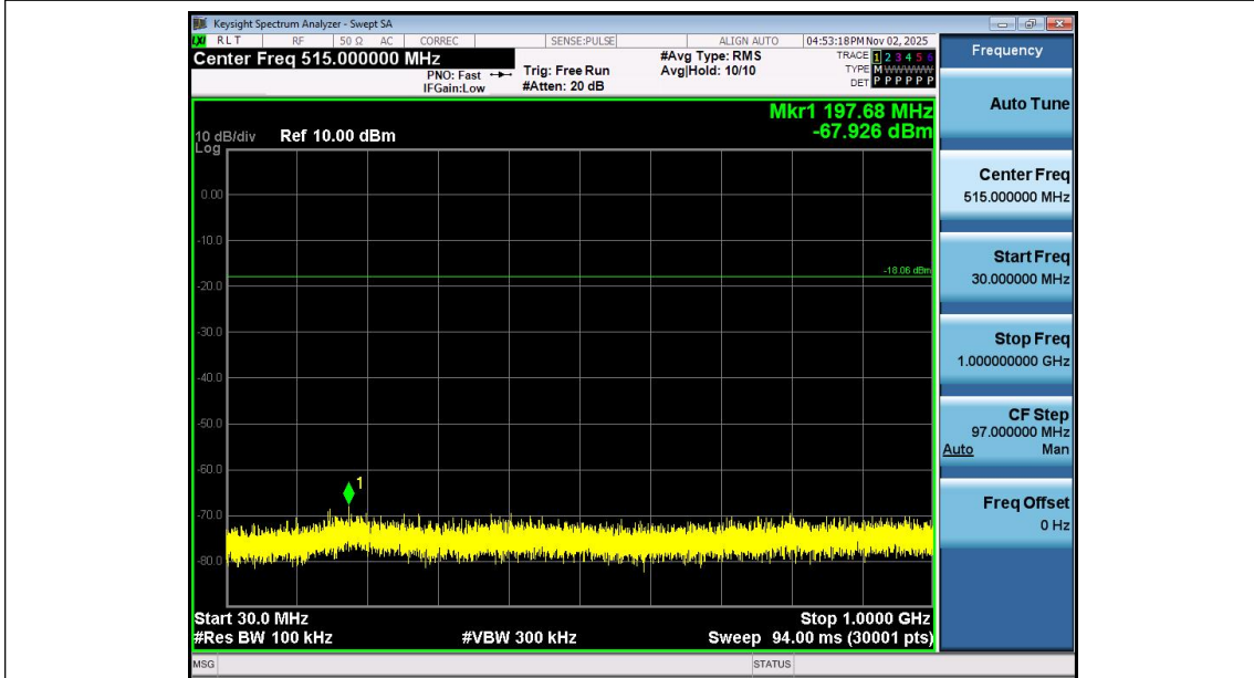
BLE_1M-Ant1-2480-30~1000-PASS
