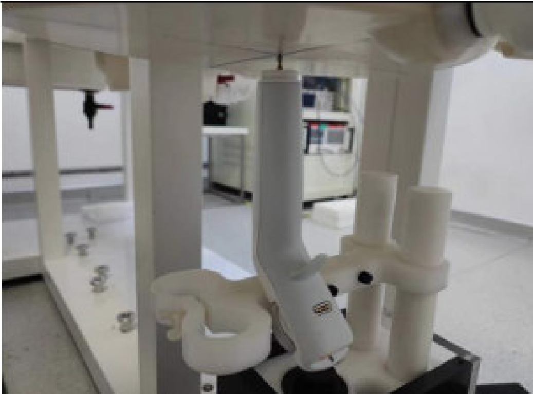
Picture 9: Bottom Edge2, the distance from EUT to the bottom of the Phantom is 0mm
