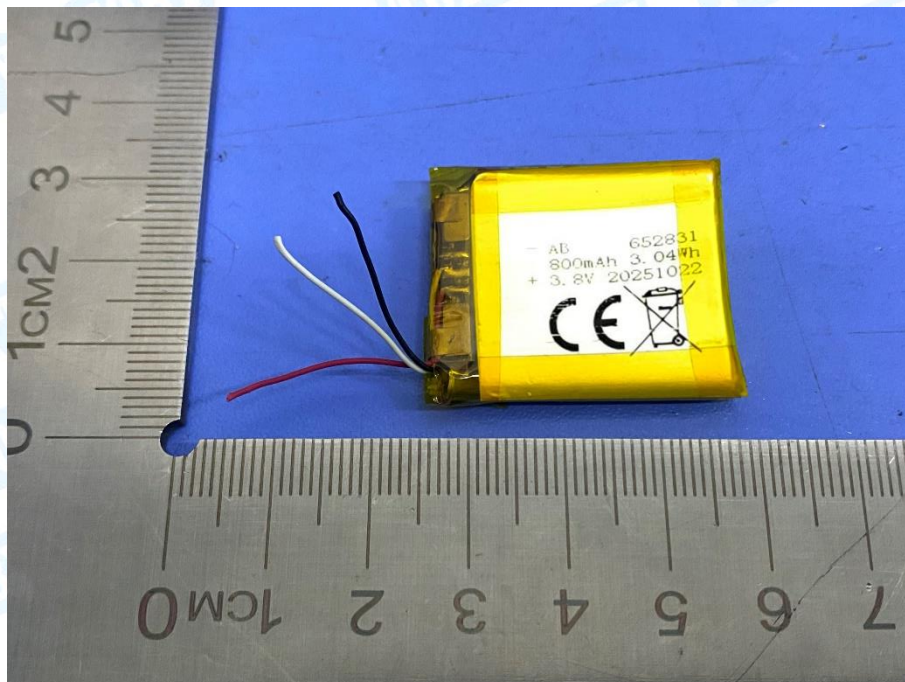
Photo 13 Internal of Battery
