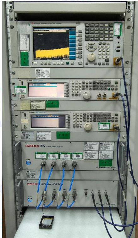
Photo of Setup for RF Conducted
