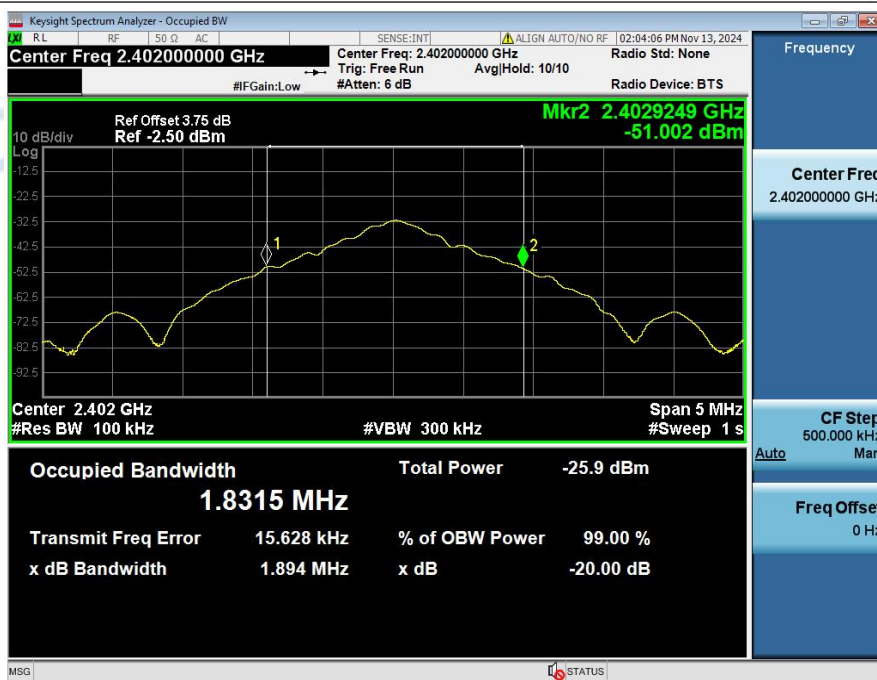
Occupied Channel Bandwidth NVNT ANT1 1-DH5 2402
