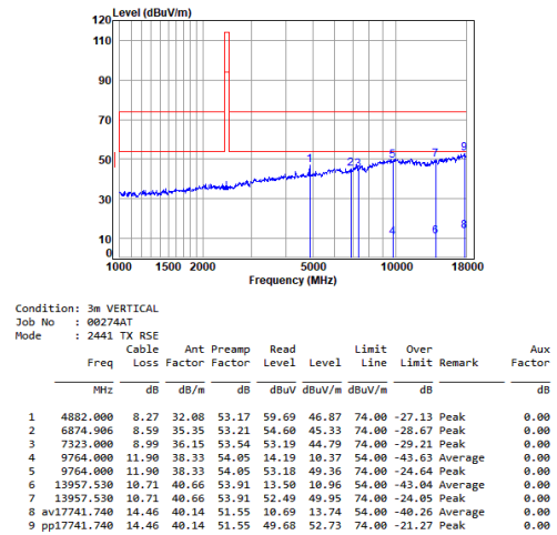
2.4G SRD_TX_CH_M_Vertical
