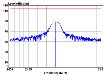
2.4G SRD_TX_CH_M_Horizontal
