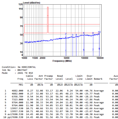
2.4G SRD_TX_CH_M_Horizontal
