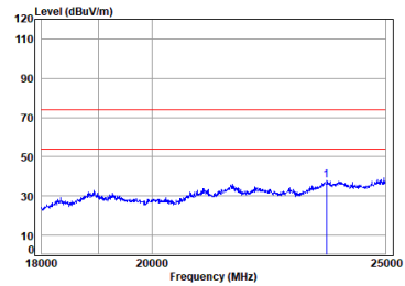
2.4G SRD_TX_CH_M_Vertical
