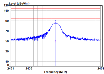
2.4G SRD_TX_CH_M_Vertical
