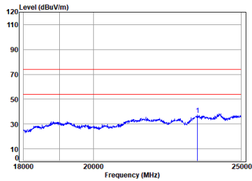
2.4G SRD_TX_CH_M_Horizontal
