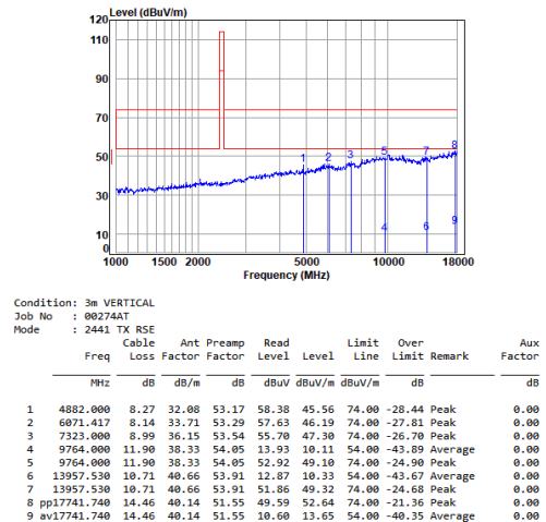
2.4G SRD_TX_CH_M_Vertical
