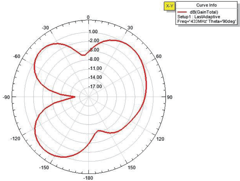
Radiation Pattern 2
