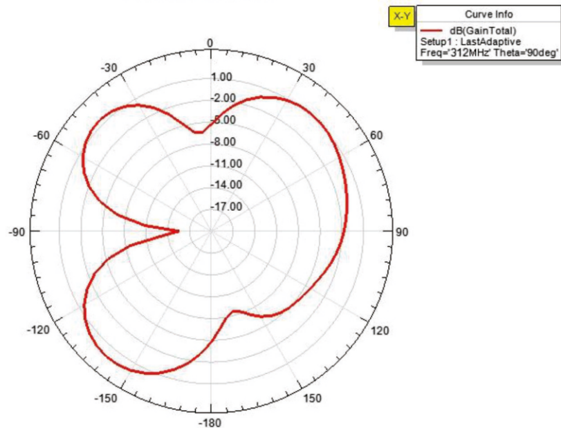
Radiation Pattern 2
