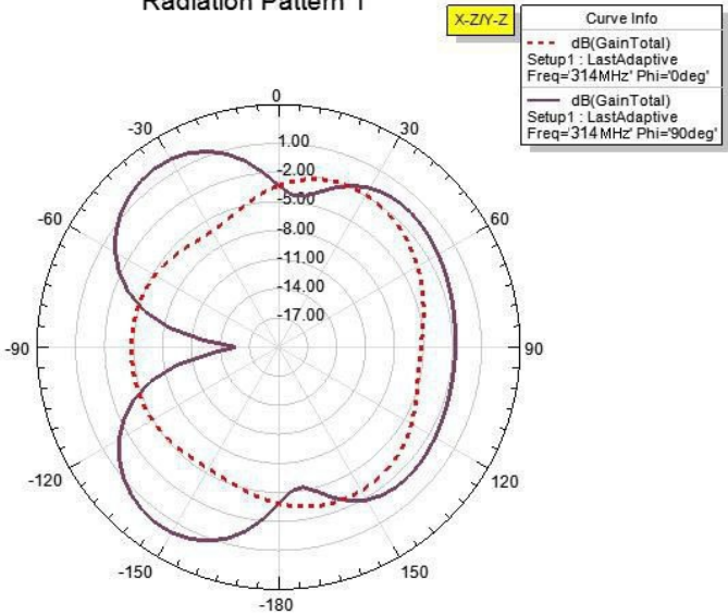
Radiation Pattern 1
