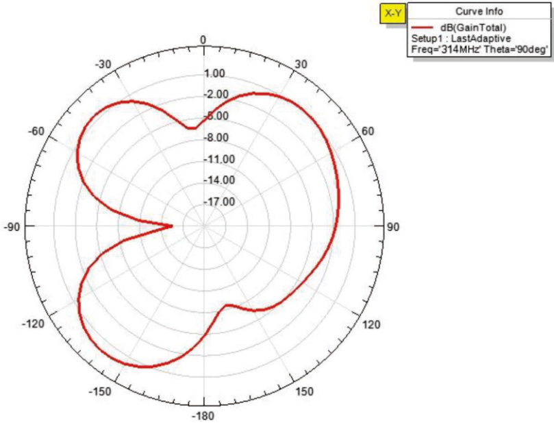
Radiation Pattern 2
