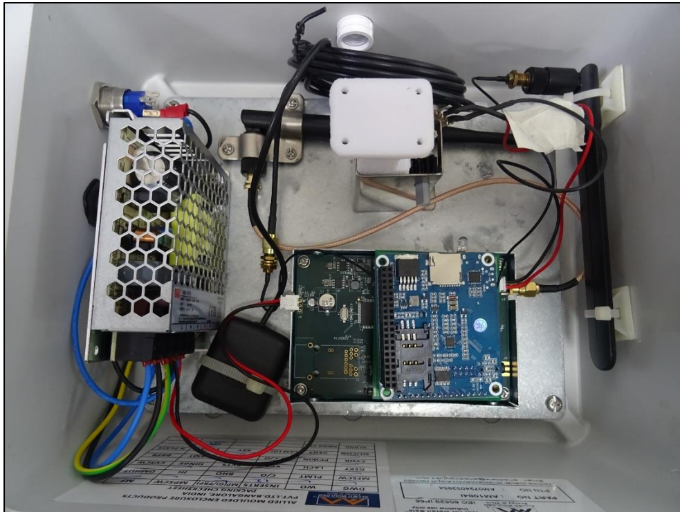
EUT Without enclosure
