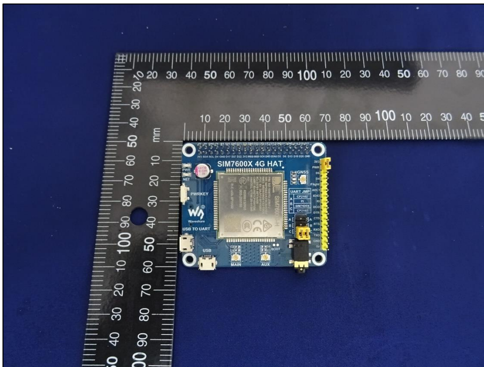
Dimensional view of the EUT PCB
