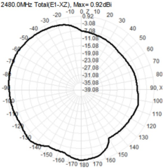
2480MHz Phi 0 2D
