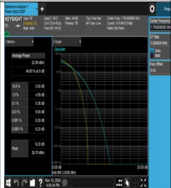
Band4-1.4MHz-16QAM-20393-6RB#0-PASS
