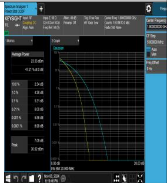
Band2-20MHz-16QAM-19100-100RB#0-PASS
