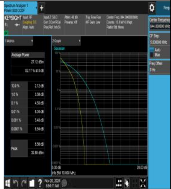
26(824-849)-10MHz-16QAM-26990-50RB#0-PAS
