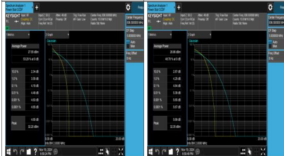
26(824-849)-1.4MHz-QPSK-26915-6RB#0-PASS
