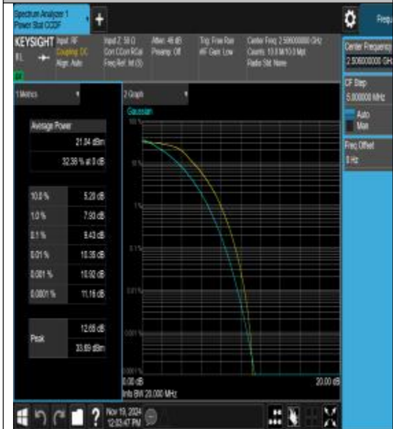
Band41-20MHz-QPSK-39750-100RB#0-PASS
