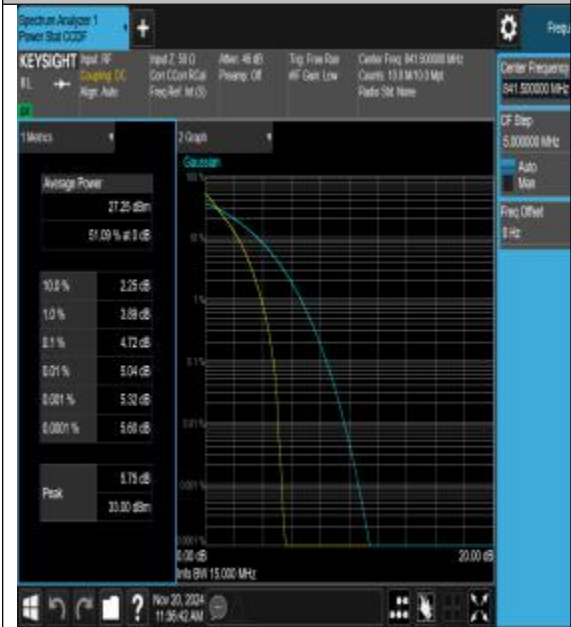
26(824-849)-15MHz-QPSK-26965-75RB#0-PASS
