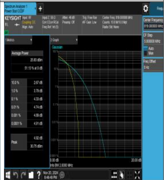
26(814-824)-1.4MHz-16QAM-26740-6RB#0-PASS
