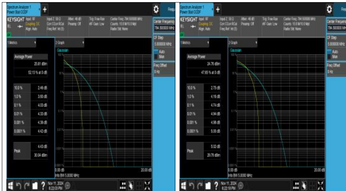
Band13-5MHz-QPSK-23255-1RB#0-PASS
