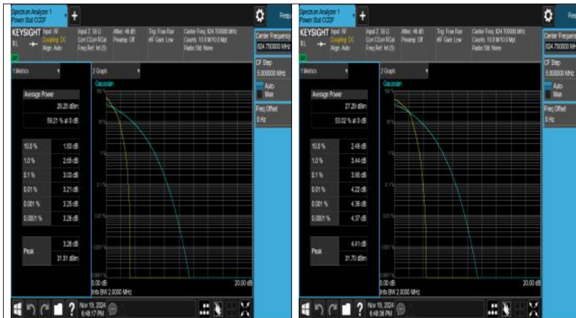
26(824-849)-1.4MHz-QPSK-26797-1RB#0-PASS
