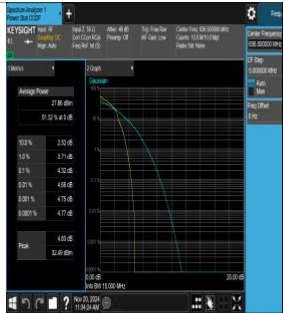
26(824-849)-15MHz-16QAM-26915-1RB#0-PASS
