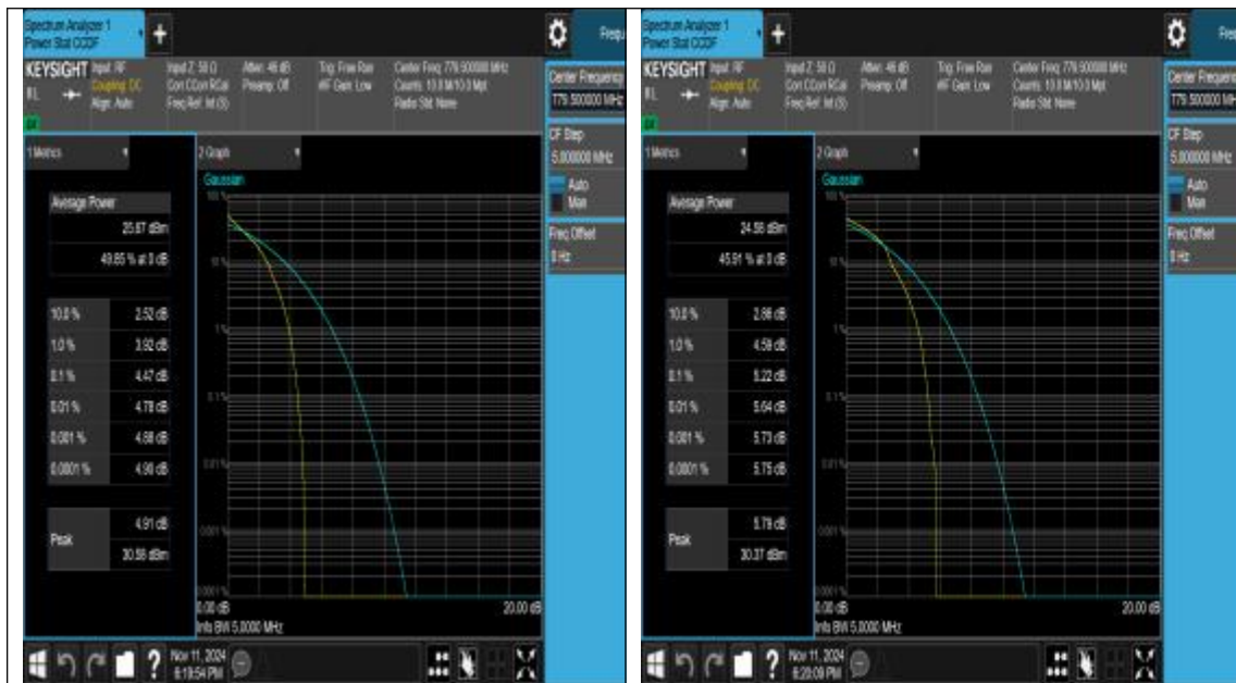
Band13-5MHz-QPSK-23205-1RB#0-PASS
