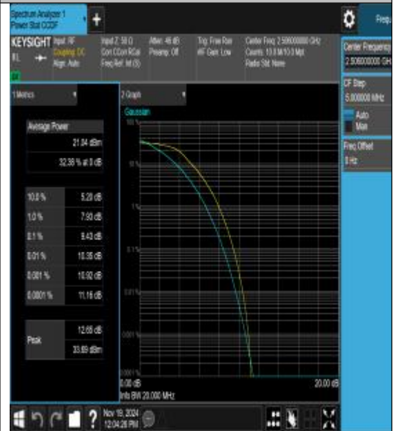
Band41-20MHz-16QAM-39750-100RB#0-PASS
