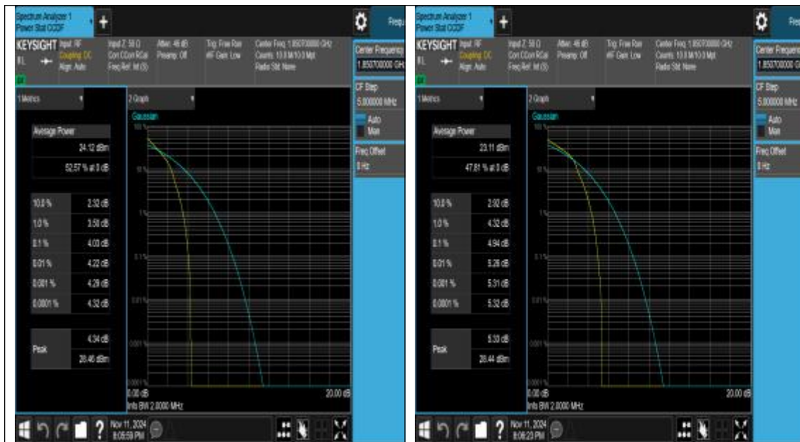
Band25-1.4MHz-QPSK-26047-1RB#0-PASS
