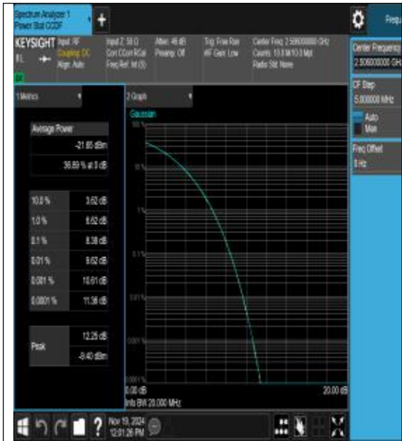
Band41-20MHz-QPSK-39750-1RB#0-PASS
