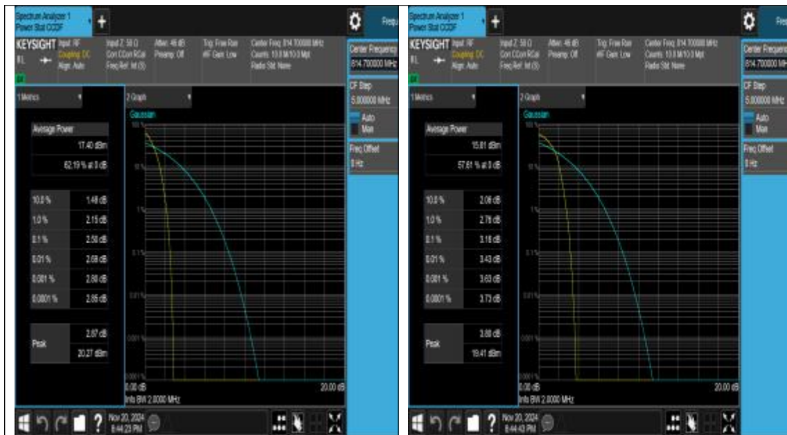
26(814-824)-1.4MHz-QPSK-26697-1RB#0-PASS
