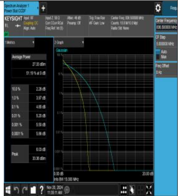
26(824-849)-15MHz-16QAM-26915-75RB#0-PAS
