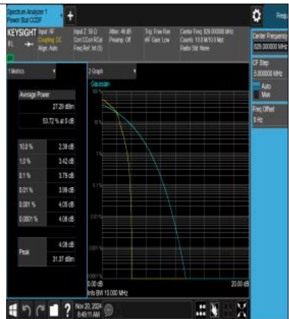
26(824-849)-10MHz-16QAM-26840-1RB#0-PASS
