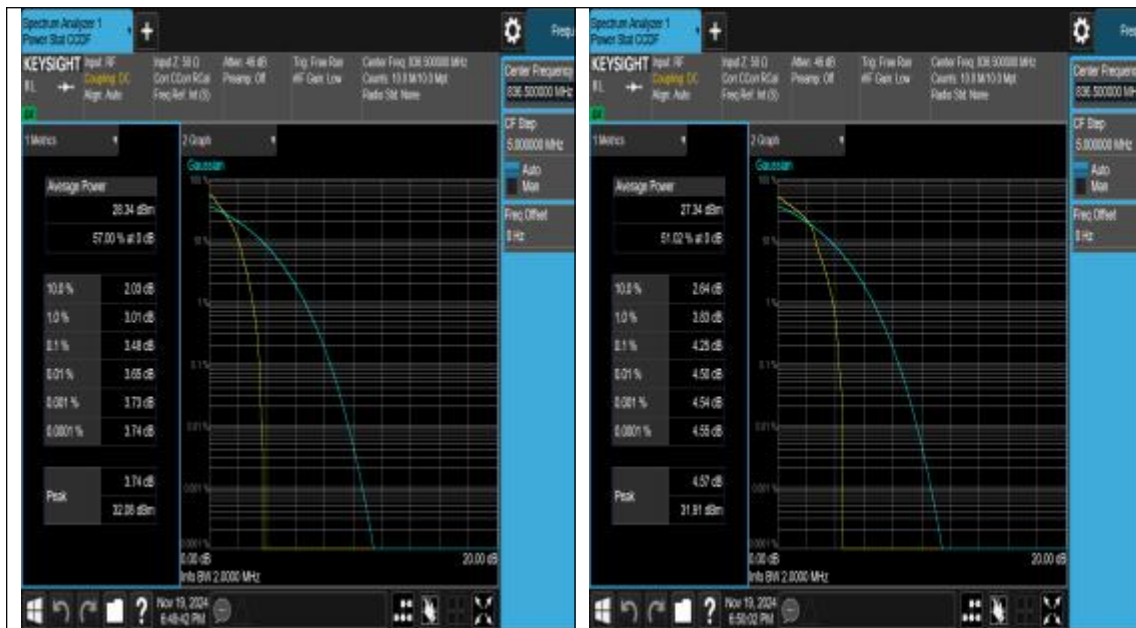
26(824-849)-1.4MHz-QPSK-26915-1RB#0-PASS
