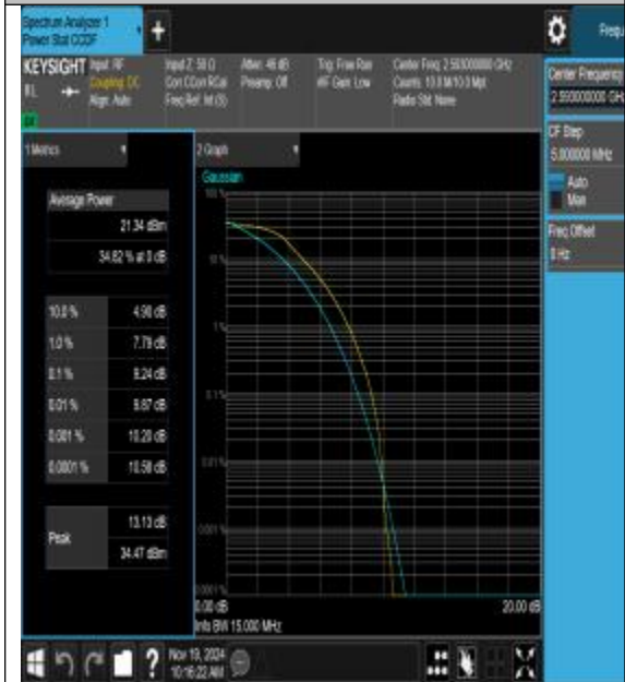
Band41-15MHz-QPSK-40620-75RB#0-PASS
