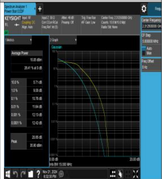
40(2305-2320)-15MHz-16QAM-38775-75RB#0-PA
