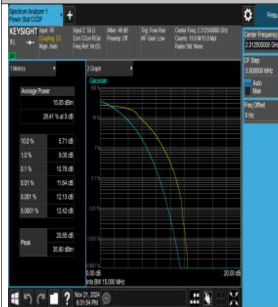
40(2305-2320)-15MHz-QPSK-38775-75RB#0-PA
