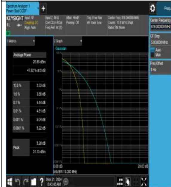
26(814-824)-10MHz-QPSK-26740-50RB#0-PASS
