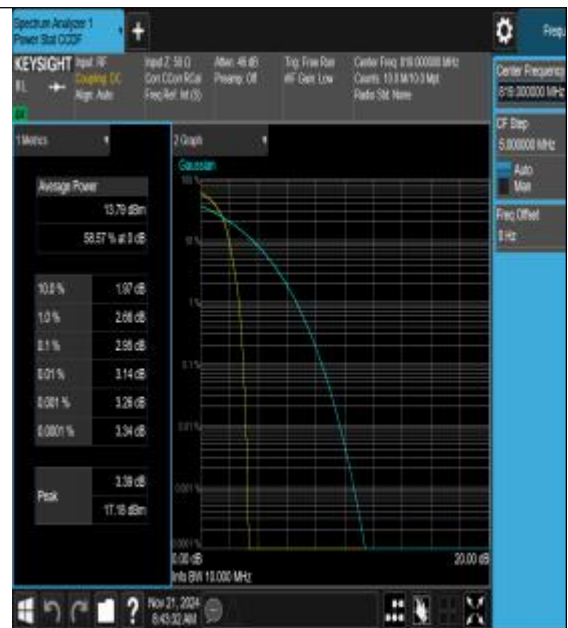
26(814-824)-10MHz-16QAM-26740-1RB#0-PASS
