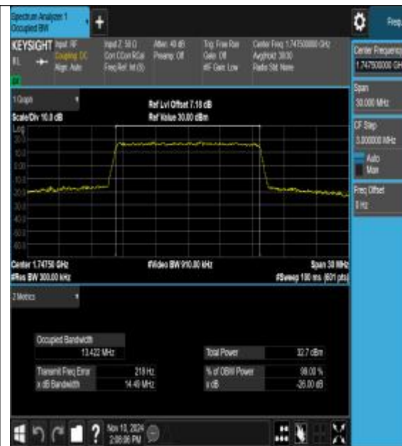
Band4-15MHz-16QAM-20325-75RB#0-PASS
