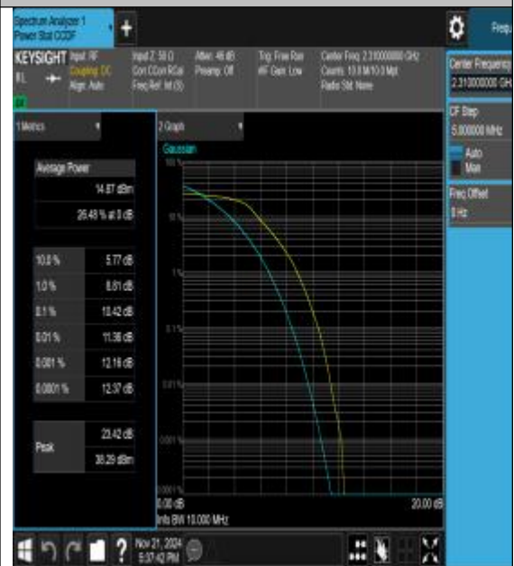
40(2305-2320)-10MHz-16QAM-38750-50RB#0-PA
