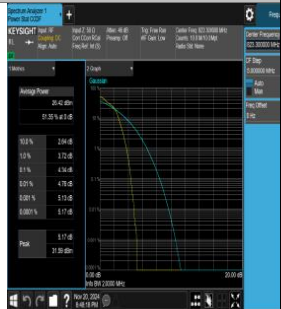
26(814-824)-1.4MHz-16QAM-26783-6RB#0-PASS
