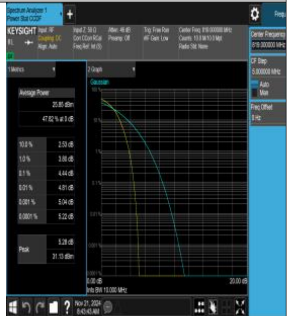
26(814-824)-10MHz-16QAM-26740-50RB#0-PAS
