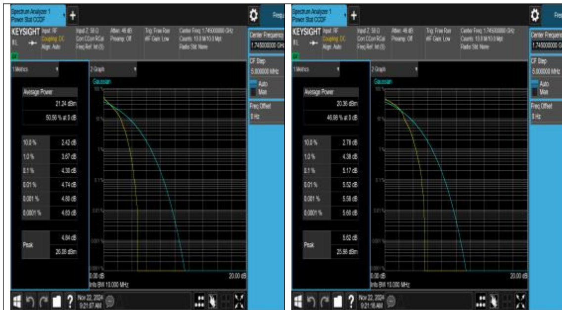
Band66-10MHz-QPSK-132322-1RB#0-PASS
