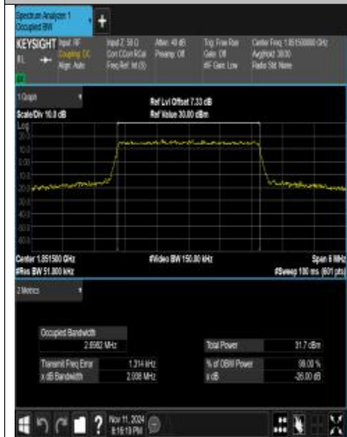
Band25-3MHz-QPSK-26055-15RB#0-PASS
