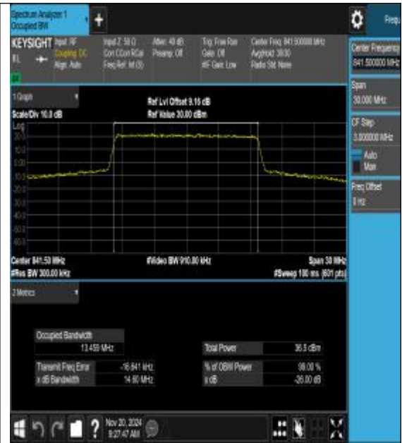
26(824-849)-15MHz-16QAM-26965-75RB#0-PAS
