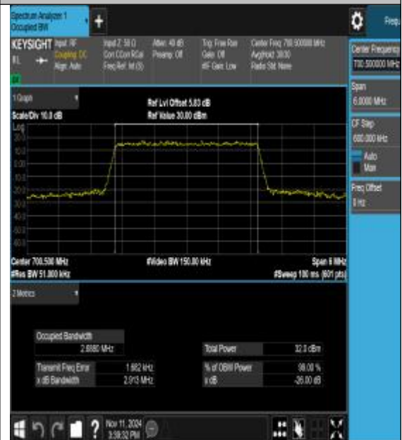
Band12-3MHz-16QAM-23025-15RB#0-PASS
