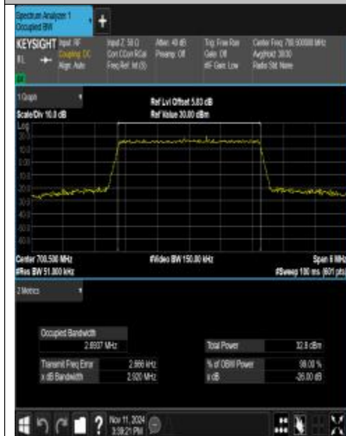
Band12-3MHz-QPSK-23025-15RB#0-PASS
