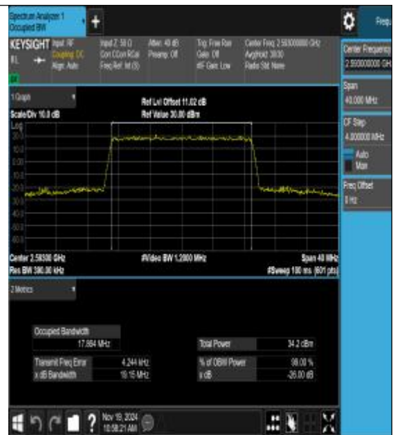
Band41-20MHz-16QAM-40620-100RB#0-PASS
