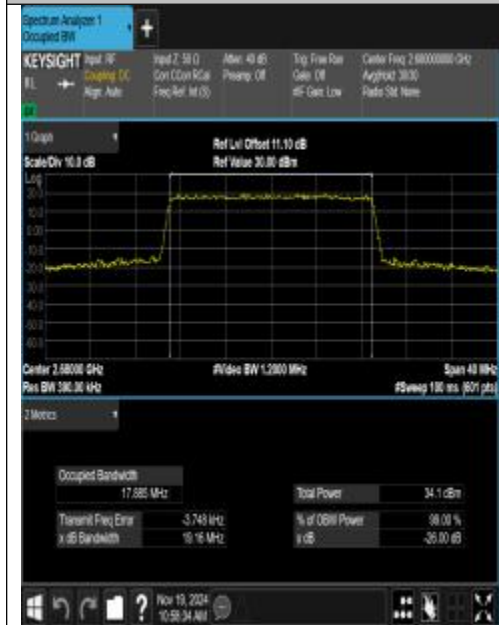
Band41-20MHz-QPSK-41490-100RB#0-PASS
