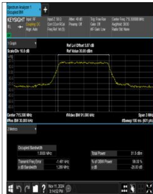
Band12-1.4MHz-QPSK-23173-6RB#0-PASS
