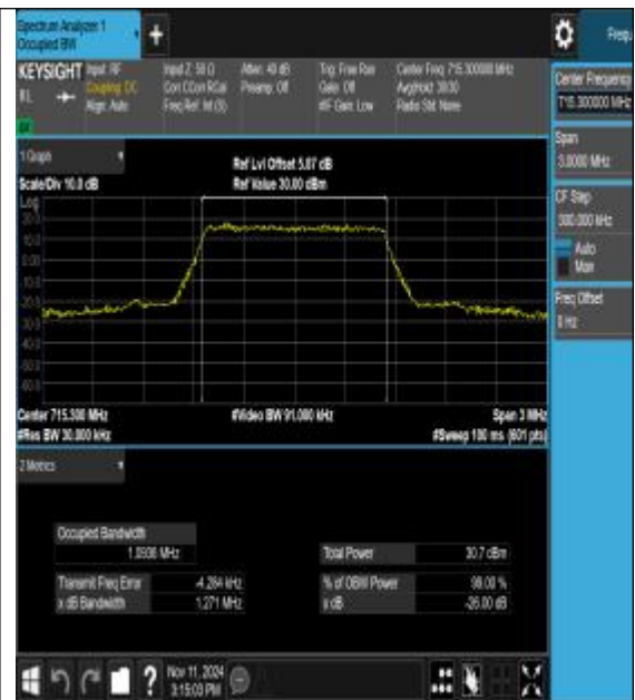
Band12-1.4MHz-16QAM-23173-6RB#0-PASS
