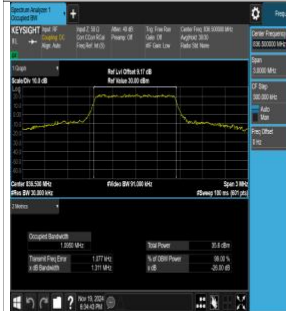
26(824-849)-1.4MHz-QPSK-26915-6RB#0-PASS
