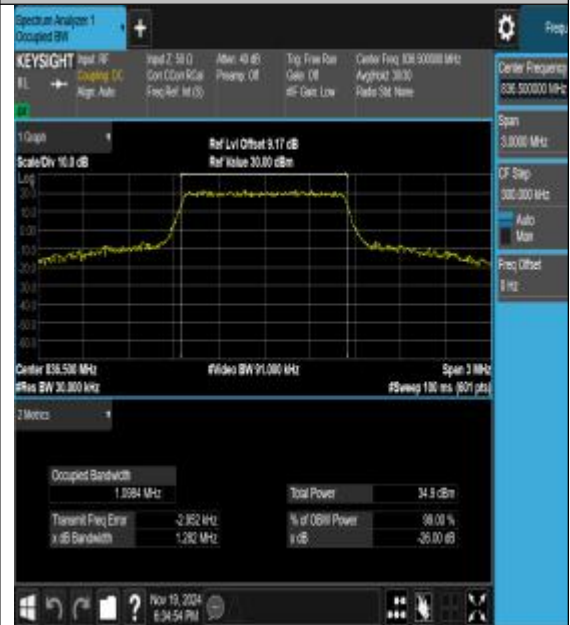
26(824-849)-1.4MHz-16QAM-26915-6RB#0-PASS
