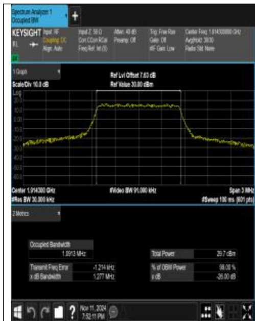
Band25-1.4MHz-QPSK-26683-6RB#0-PASS
