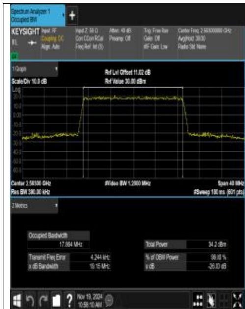
Band41-20MHz-QPSK-40620-100RB#0-PASS
