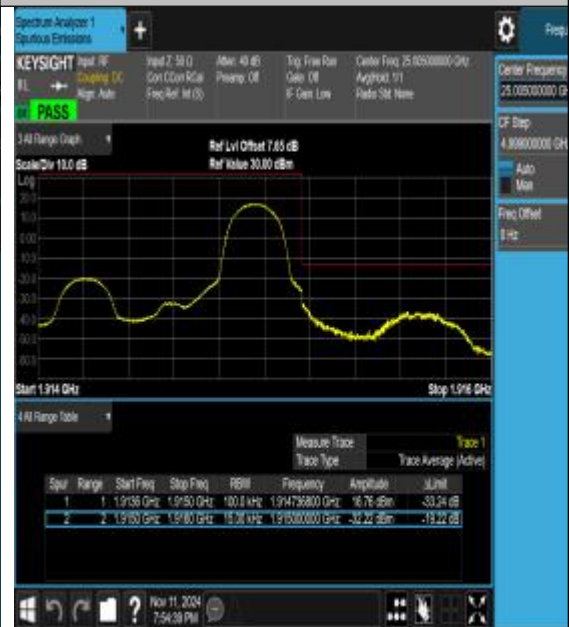
Band25_1.4MHz_16QAM_26683_1RB#5
