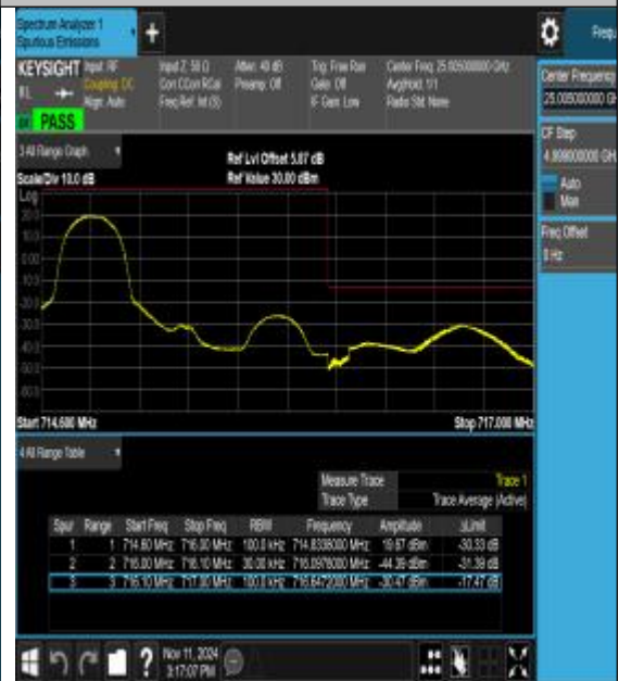
Band12_1.4MHz_16QAM_23173_1RB#0
