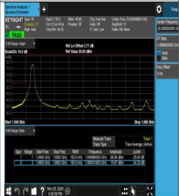
Band25_10MHz_16QAM_26090_1RB#0
