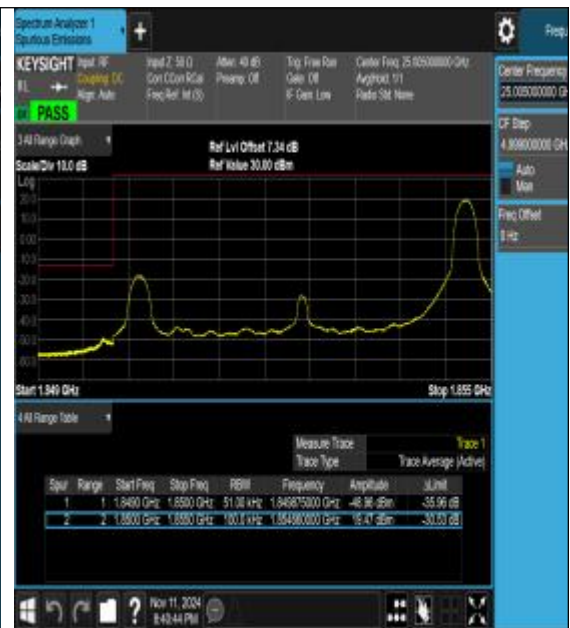
Band25_5MHz_16QAM_26065_1RB#24
