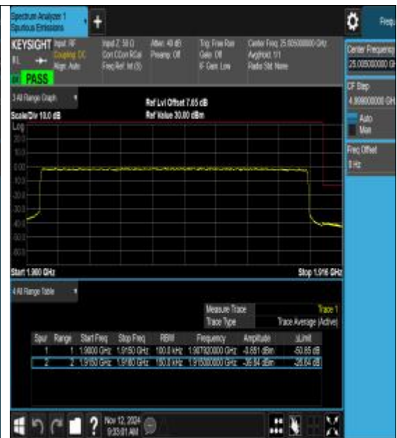
Band25_15MHz_16QAM_26615_75RB#0
