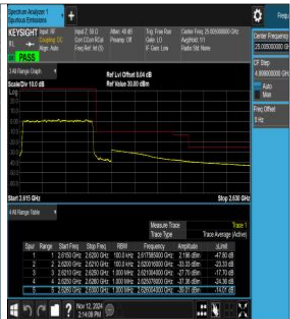
Band38_5MHz_16QAM_38225_25RB#0
