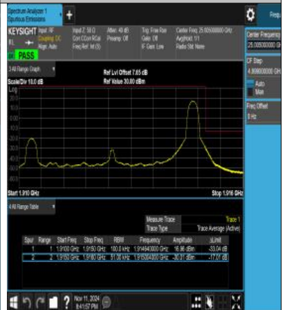
Band25_5MHz_16QAM_26665_1RB#24
