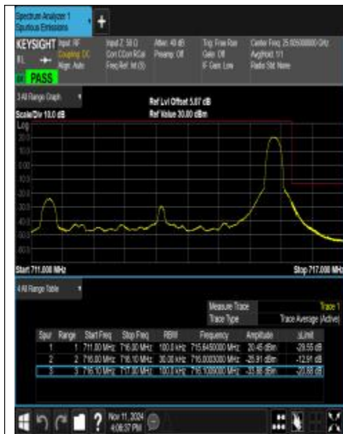
Band12_5MHz_QPSK_23155_1RB#24
