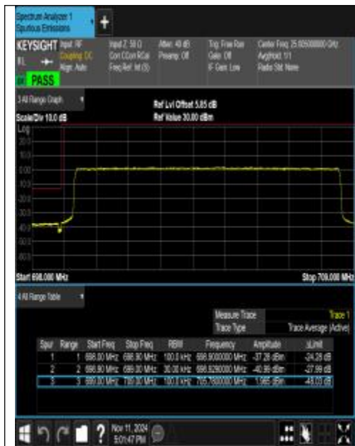
Band12_10MHz_QPSK_23060_50RB#0
