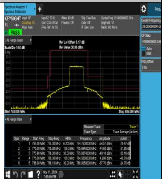
Band13_5MHz_16QAM_23255_25RB#0
