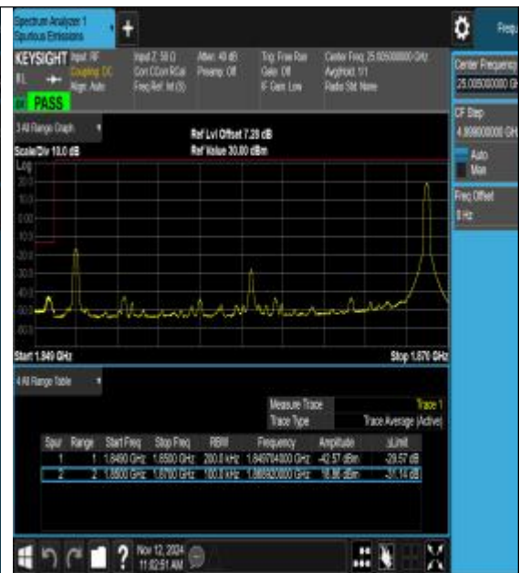
Band25_20MHz_16QAM_26140_1RB#99
