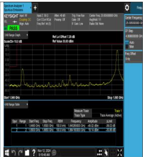
Band25_15MHz_16QAM_26115_1RB#74
