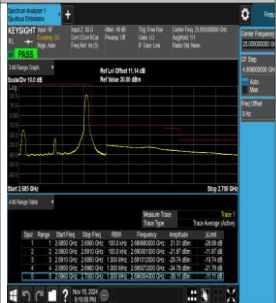
Band41_5MHz_16QAM_41565_1RB#24
