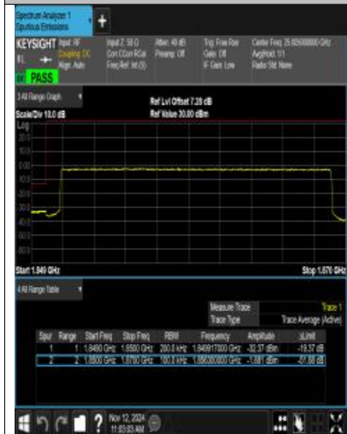
Band25_20MHz_QPSK_26140_100RB#0
