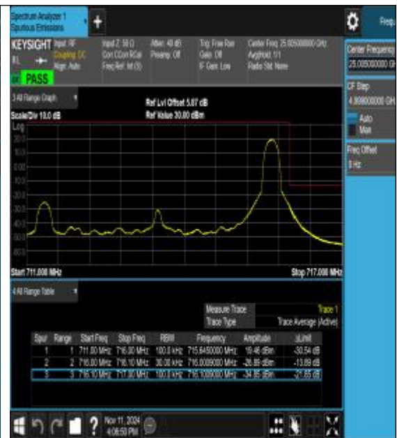
Band12_5MHz_16QAM_23155_1RB#24
