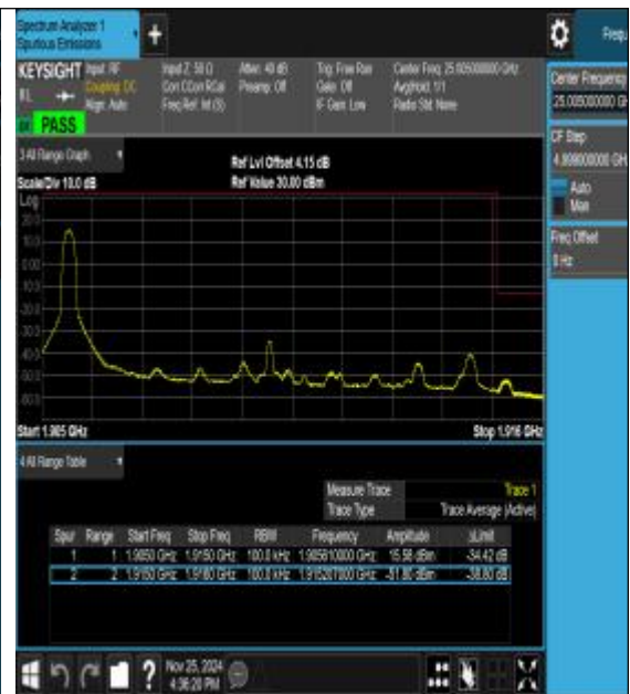
Band25_10MHz_16QAM_26640_1RB#0
