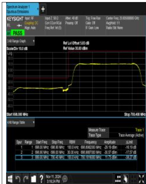
Band12_1.4MHz_QPSK_23017_6RB#0
