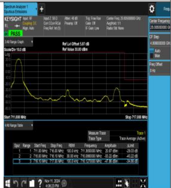
Band12_5MHz_16QAM_23155_1RB#0
