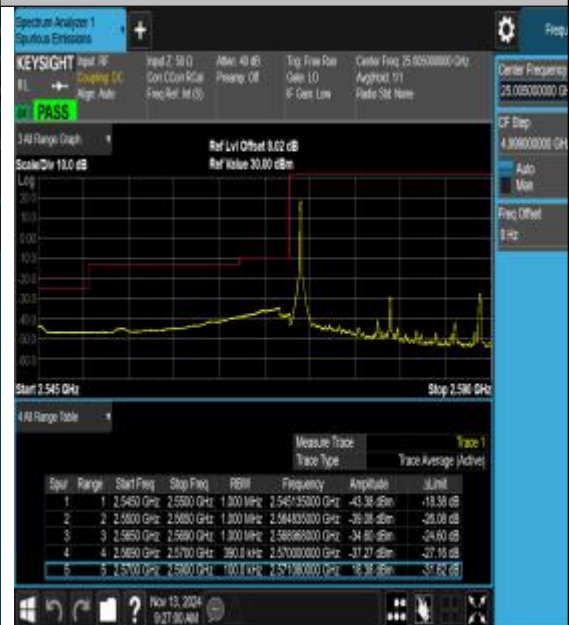
Band38_20MHz_16QAM_37850_1RB#0
