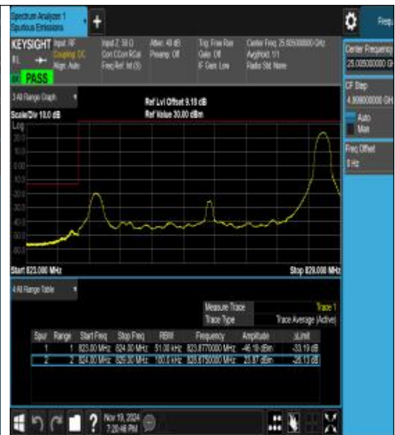
Band26_5MHz_16QAM_26815_1RB#24
