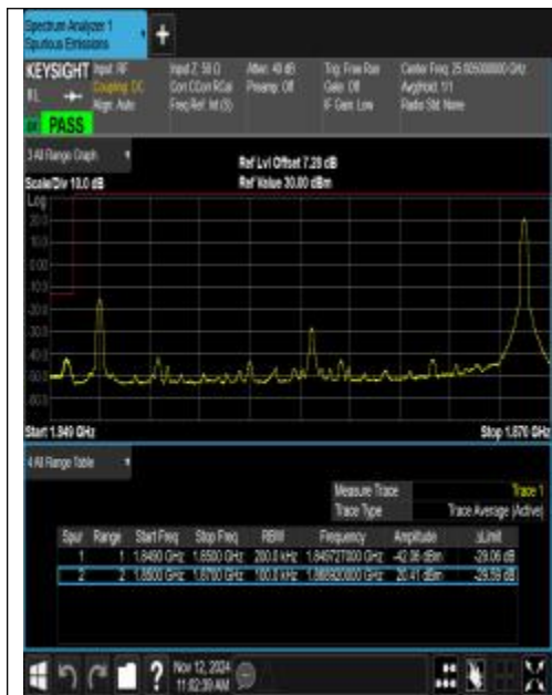
Band25_20MHz_QPSK_26140_1RB#99
