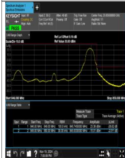
Band26_3MHz_QPSK_27025_1RB#14
