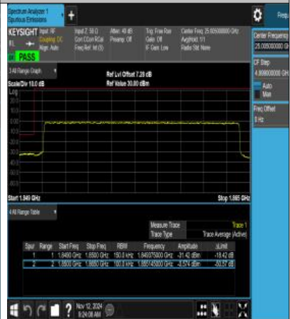
Band25_15MHz_16QAM_26115_75RB#0
