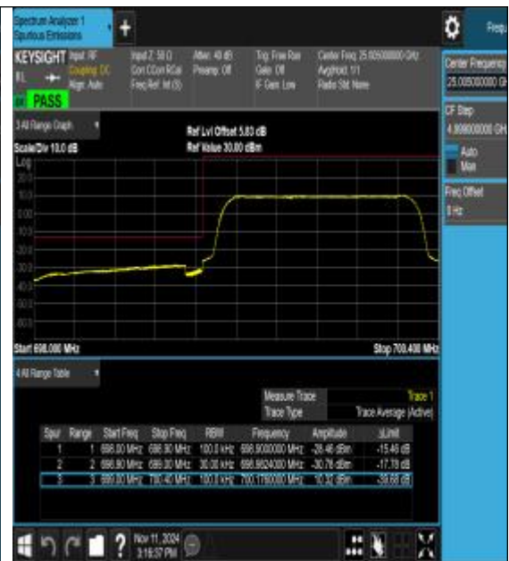
Band12_1.4MHz_16QAM_23017_6RB#0
