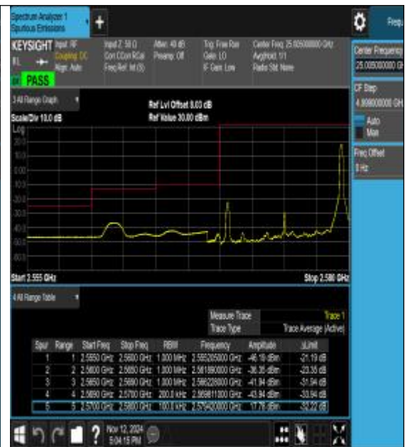
Band38_10MHz_16QAM_37800_1RB#49
