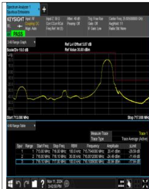
Band12_3MHz_QPSK_23165_1RB#14
