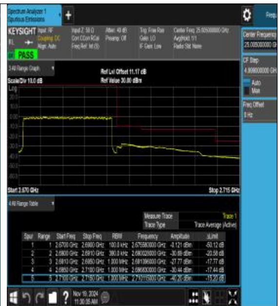
Band41_20MHz_16QAM_41490_100RB#0
