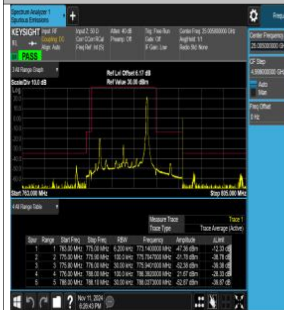
Band13_10MHz_QPSK_23230_1RB#49
