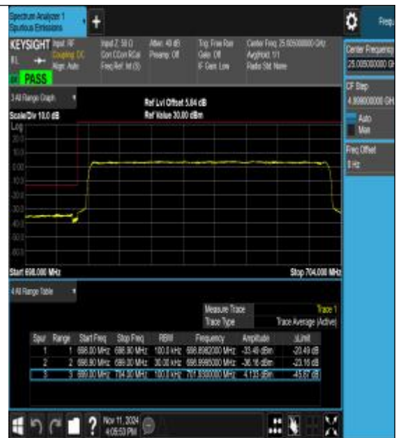
Band12_5MHz_16QAM_23035_25RB#0
