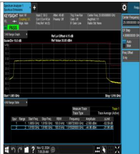
Band25_10MHz_16QAM_26640_50RB#0
