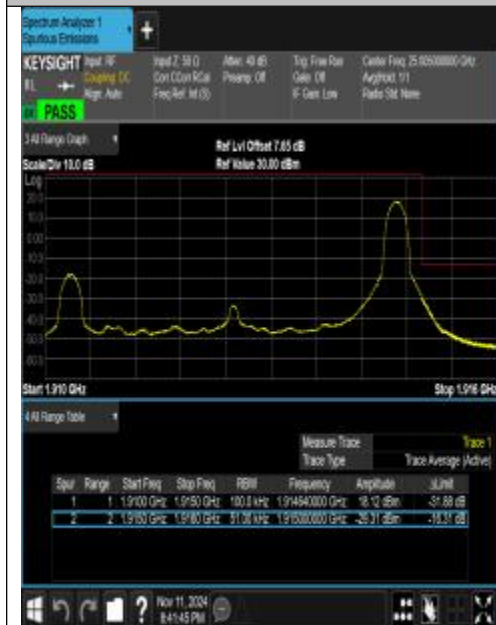
Band25_5MHz_QPSK_26665_1RB#24
