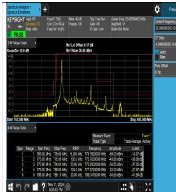
Band13_10MHz_QPSK_23230_1RB#0
