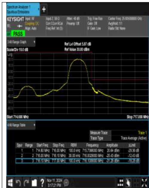
Band12_1.4MHz_QPSK_23173_1RB#5
