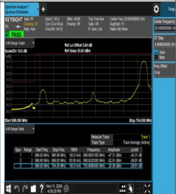
Band12_5MHz_16QAM_23035_1RB#24
