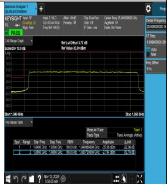
Band25_10MHz_16QAM_26090_50RB#0
