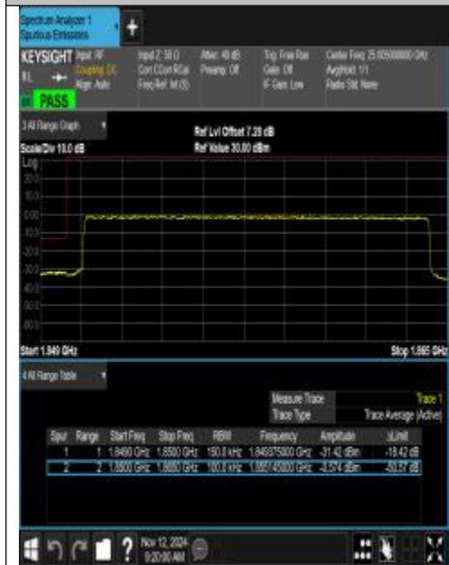
Band25_15MHz_QPSK_26115_75RB#0
