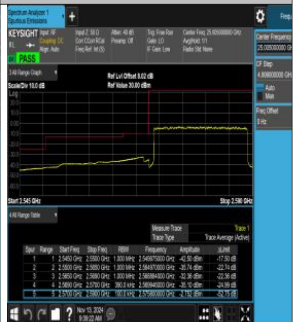
Band38_20MHz_16QAM_37850_100RB#0
