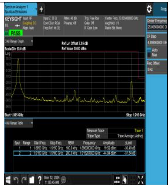
Band25_20MHz_16QAM_26590_1RB#0
