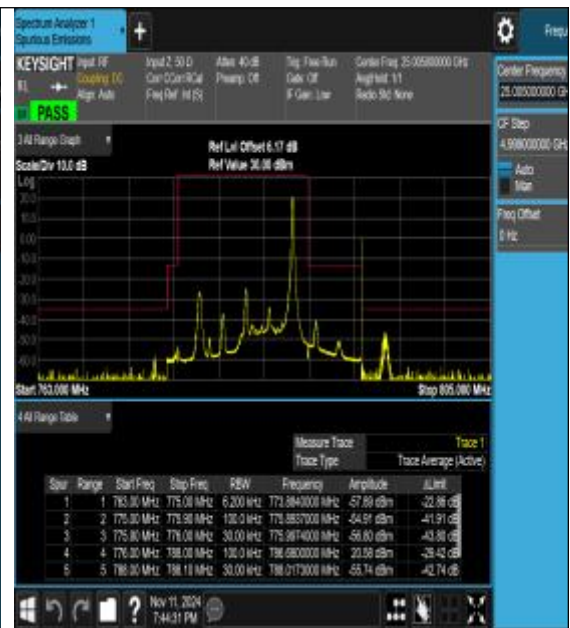
Band13_5MHz_16QAM_23255_1RB#24
