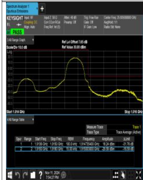
Band25_1.4MHz_QPSK_26683_1RB#5
