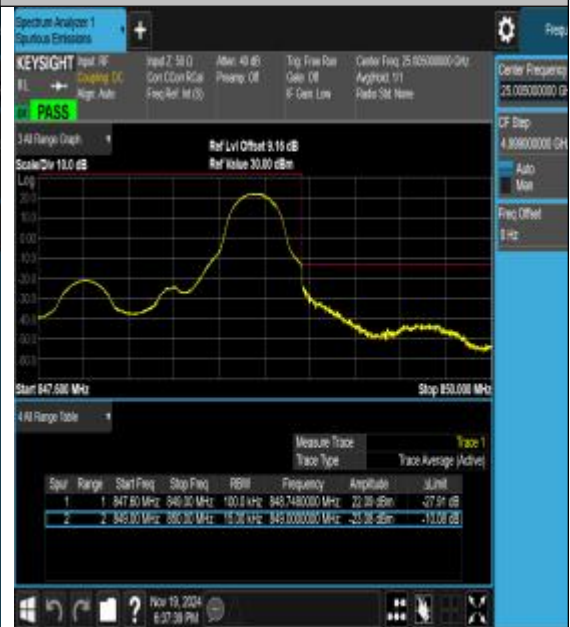
Band26_1.4MHz_16QAM_27033_1RB#5
