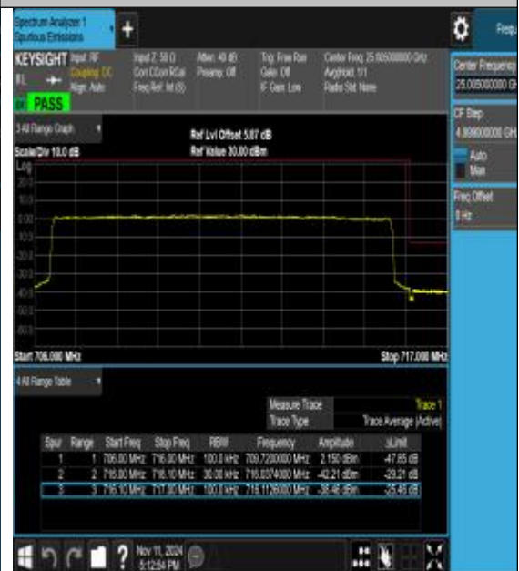
Band12_10MHz_16QAM_23130_50RB#0
