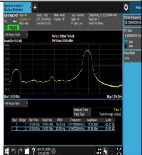
Band25_3MHz_16QAM_26675_1RB#14
