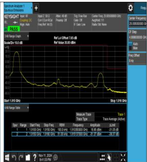
Band25_5MHz_16QAM_26665_1RB#0
