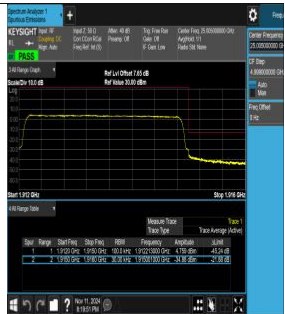
Band25_3MHz_16QAM_26675_15RB#0
