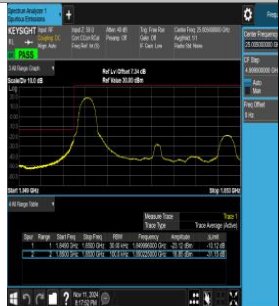
Band25_3MHz_16QAM_26055_1RB#0
