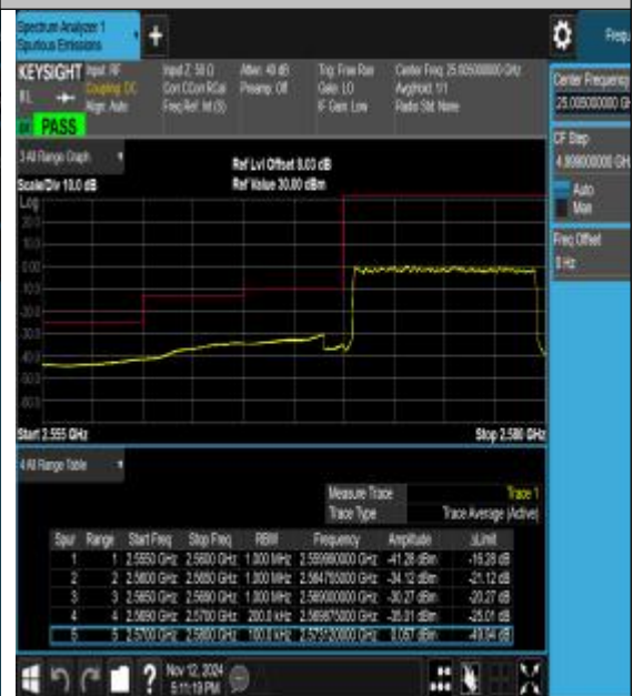
Band38_10MHz_16QAM_37800_50RB#0
