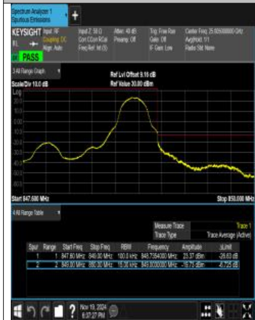
Band26_1.4MHz_QPSK_27033_1RB#5
