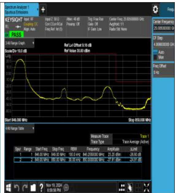
Band26_3MHz_16QAM_27025_1RB#0
