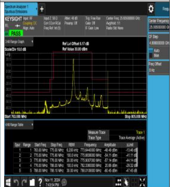
Band13_5MHz_16QAM_23255_1RB#0
