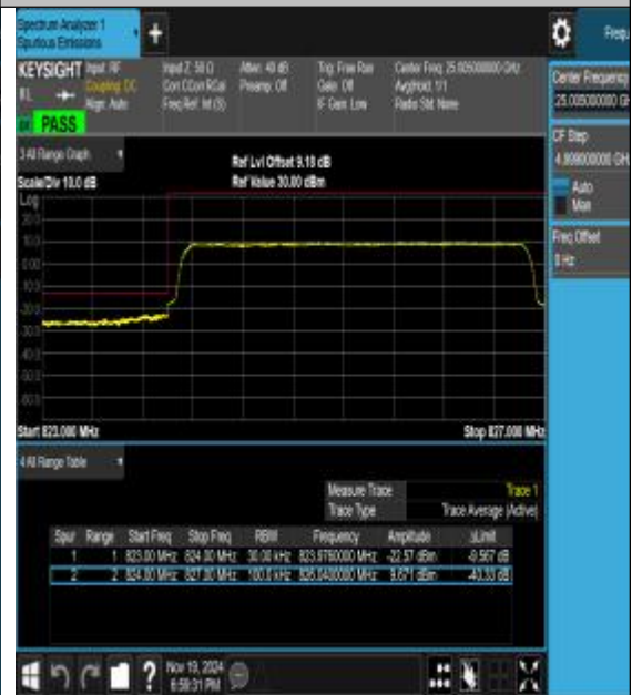
Band26_3MHz_16QAM_26805_15RB#0
