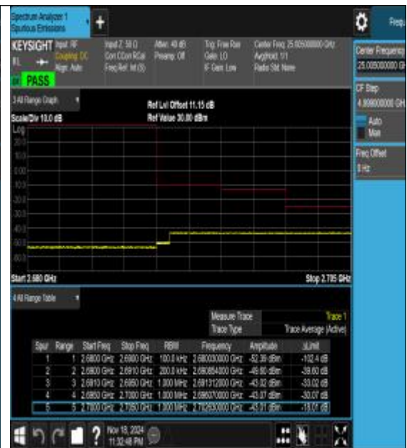
Band41_10MHz_16QAM_41540_50RB#0
