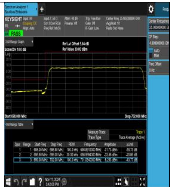
Band12_3MHz_16QAM_23025_15RB#0
