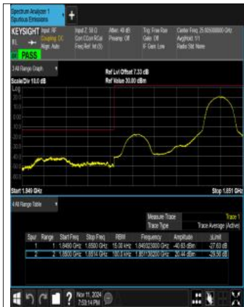
Band25_1.4MHz_QPSK_26047_1RB#5
