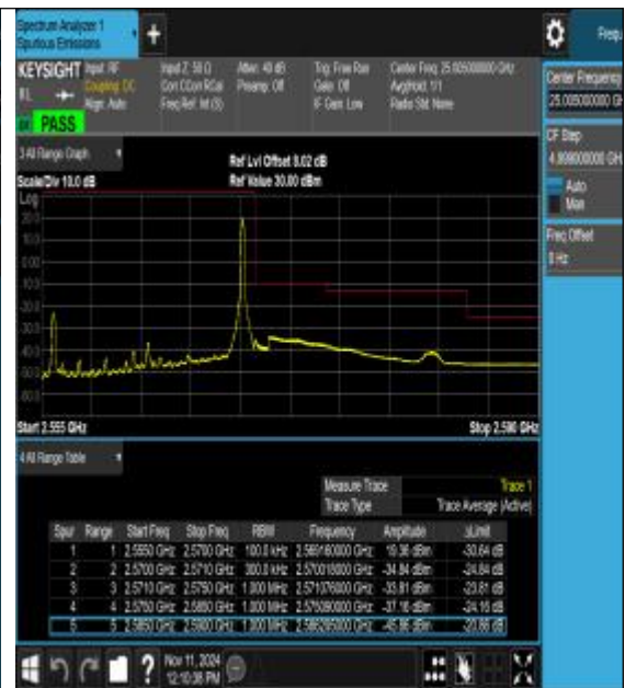
Band7_15MHz_16QAM_21375_1RB#74
