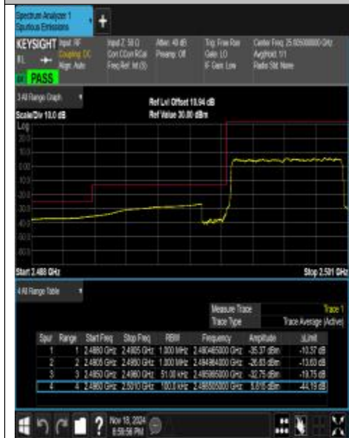
Band41_5MHz_QPSK_39675_25RB#0
