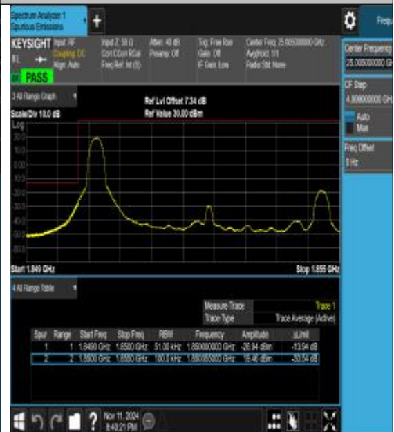
Band25_5MHz_16QAM_26065_1RB#0
