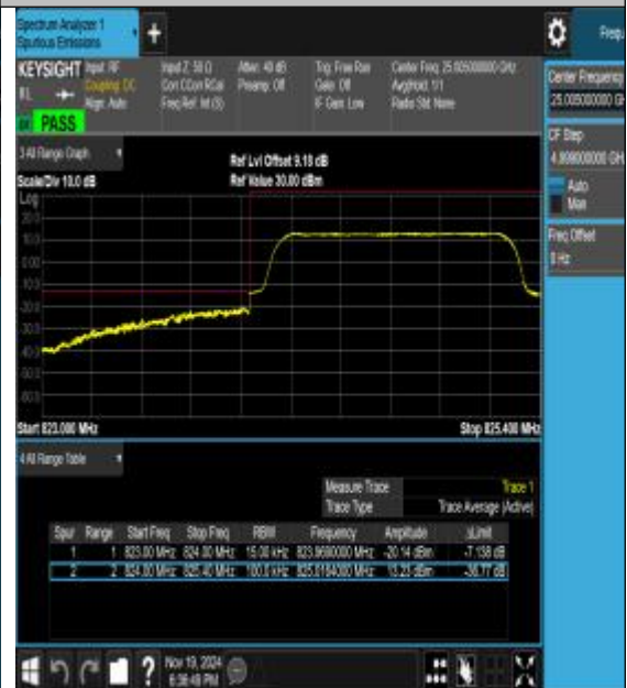
Band26_1.4MHz_16QAM_26797_6RB#0
