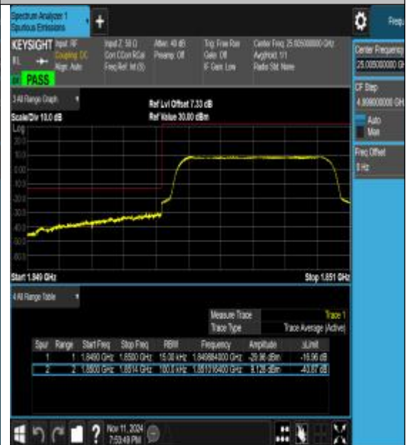
Band25_1.4MHz_16QAM_26047_6RB#0
