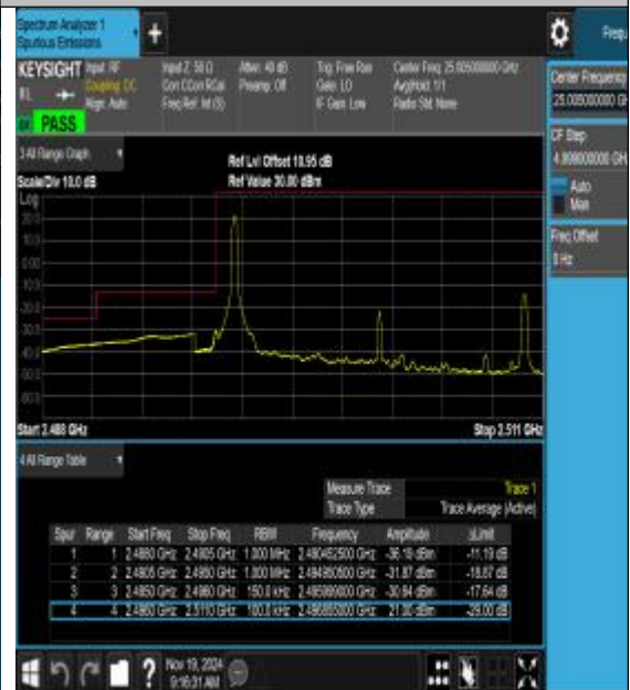
Band41_15MHz_16QAM_39725_1RB#0
