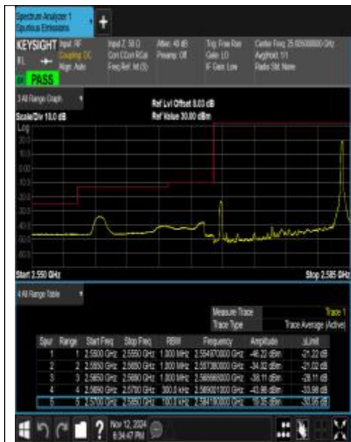
Band38_15MHz_QPSK_37825_1RB#74
