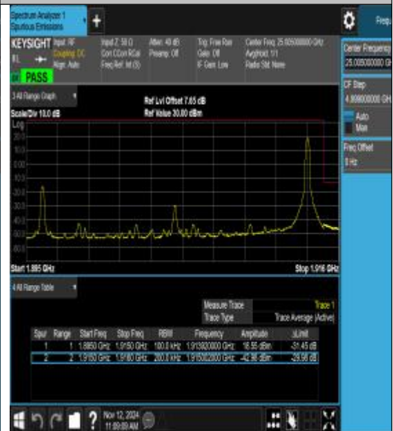
Band25_20MHz_16QAM_26590_1RB#99
