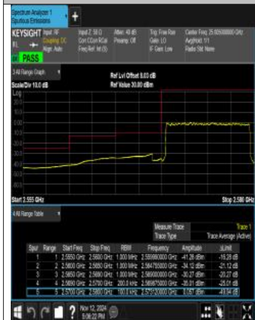
Band38_10MHz_QPSK_37800_50RB#0
