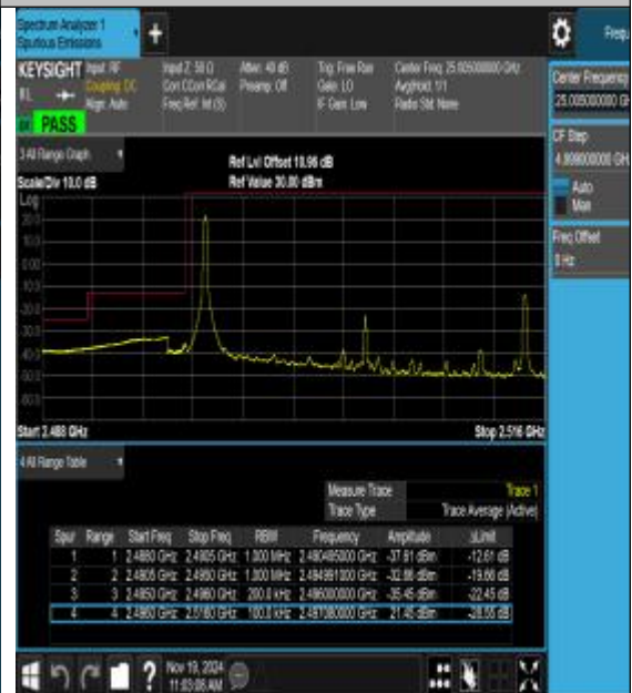
Band41_20MHz_16QAM_39750_1RB#0
