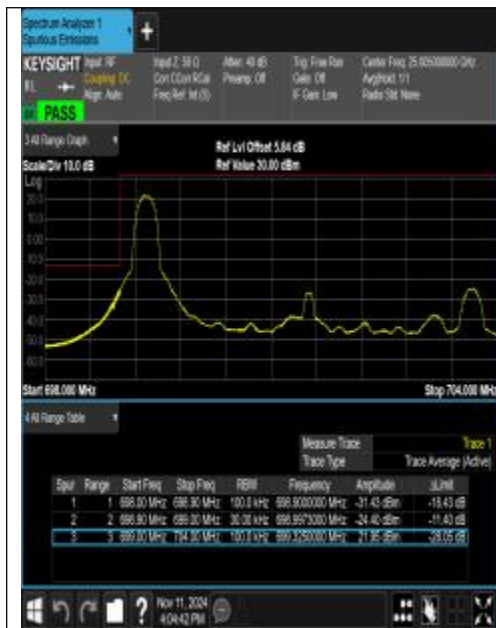
Band12_5MHz_QPSK_23035_1RB#0
