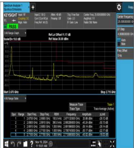
Band41_20MHz_16QAM_41490_1RB#0
