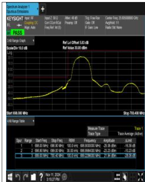
Band12_1.4MHz_QPSK_23017_1RB#0
