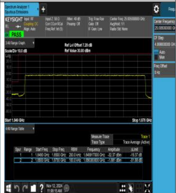
Band25_20MHz_16QAM_26140_100RB#0
