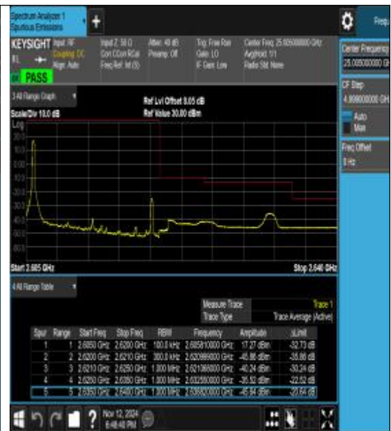
Band38_15MHz_16QAM_38175_1RB#0
