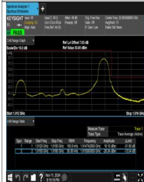
Band25_3MHz_QPSK_26675_1RB#14
