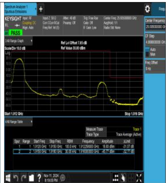
Band25_3MHz_16QAM_26675_1RB#0
