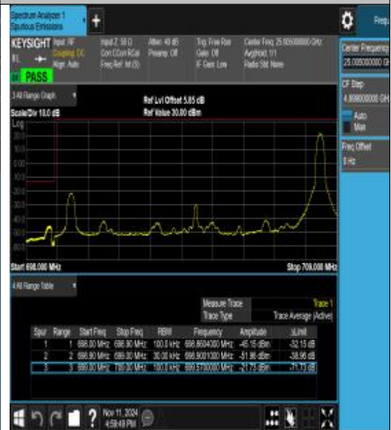
Band12_10MHz_16QAM_23060_1RB#49
