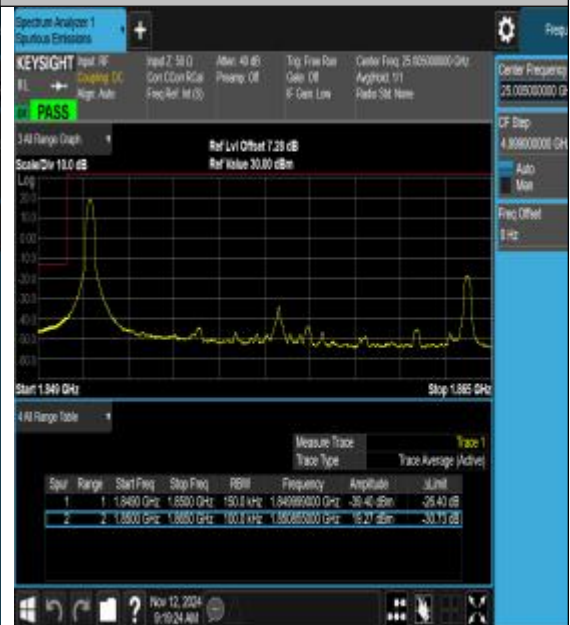
Band25_15MHz_16QAM_26115_1RB#0
