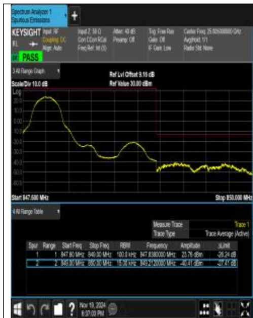
Band26_1.4MHz_QPSK_27033_1RB#0
