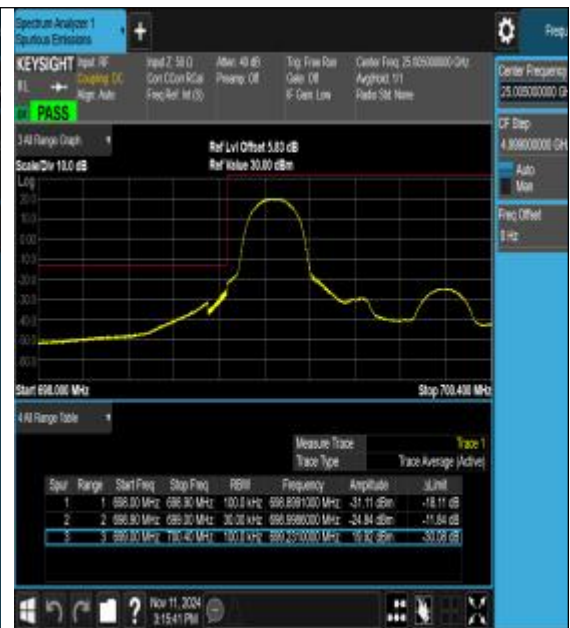
Band12_1.4MHz_16QAM_23017_1RB#0
