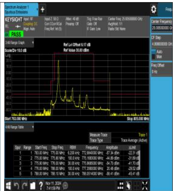
Band13_5MHz_16QAM_23205_1RB#0
