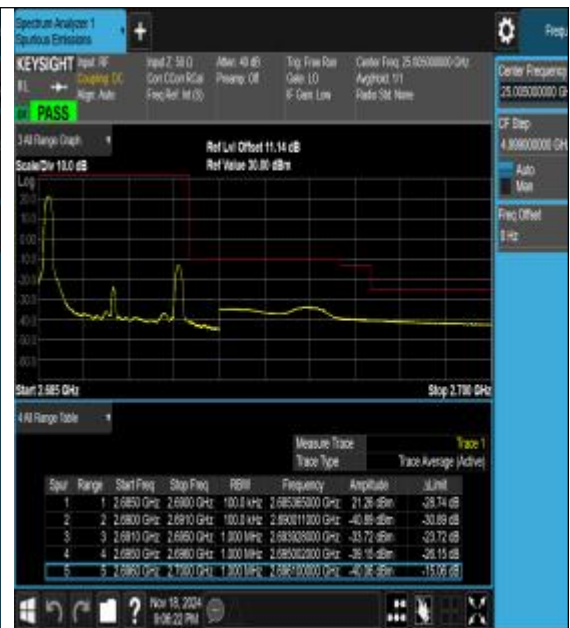
Band41_5MHz_16QAM_41565_1RB#0
