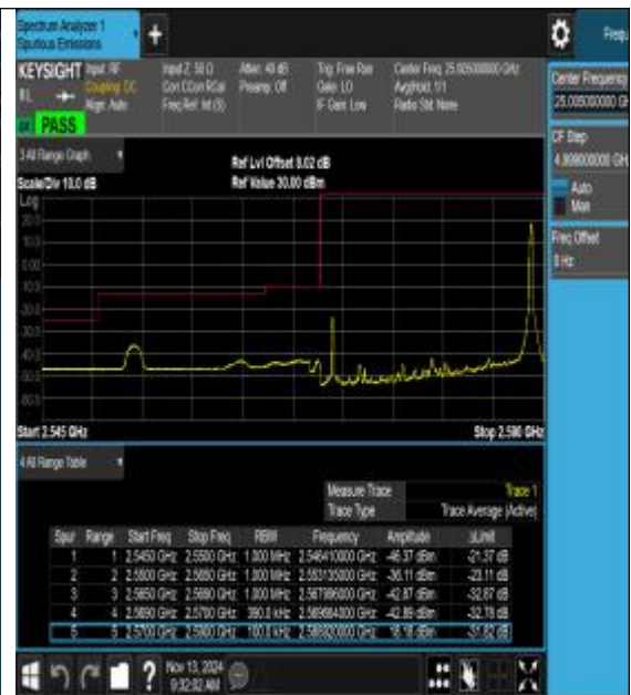
Band38_20MHz_16QAM_37850_1RB#99
