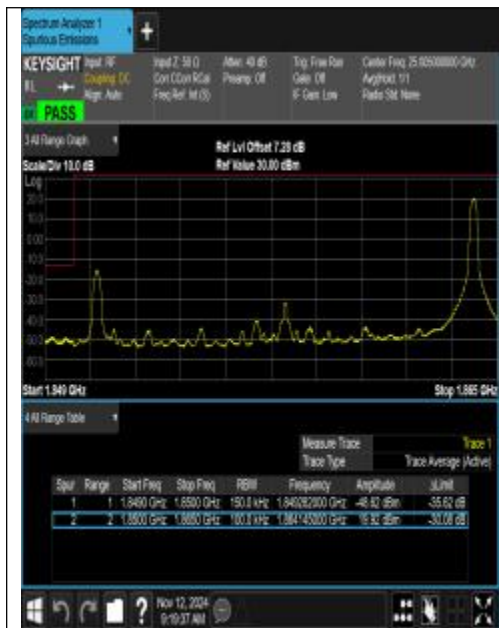
Band25_15MHz_QPSK_26115_1RB#74
