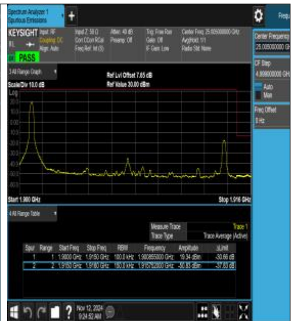
Band25_15MHz_16QAM_26615_1RB#0
