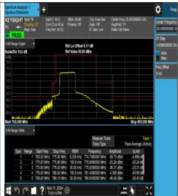
Band13_5MHz_16QAM_23205_25RB#0
