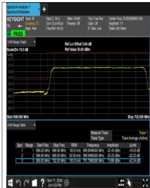
Band12_3MHz_QPSK_23025_15RB#0
