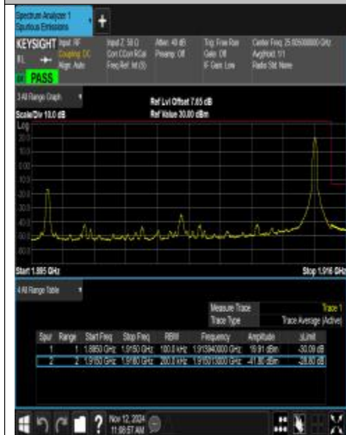
Band25_20MHz_QPSK_26590_1RB#99
