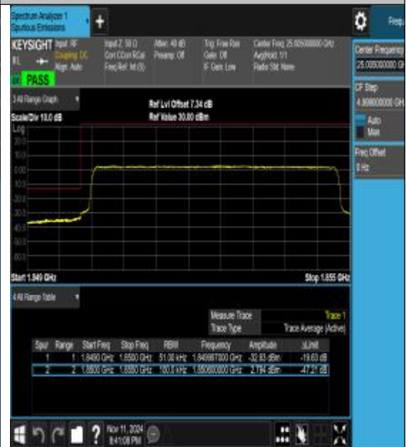
Band25_5MHz_16QAM_26065_25RB#0
