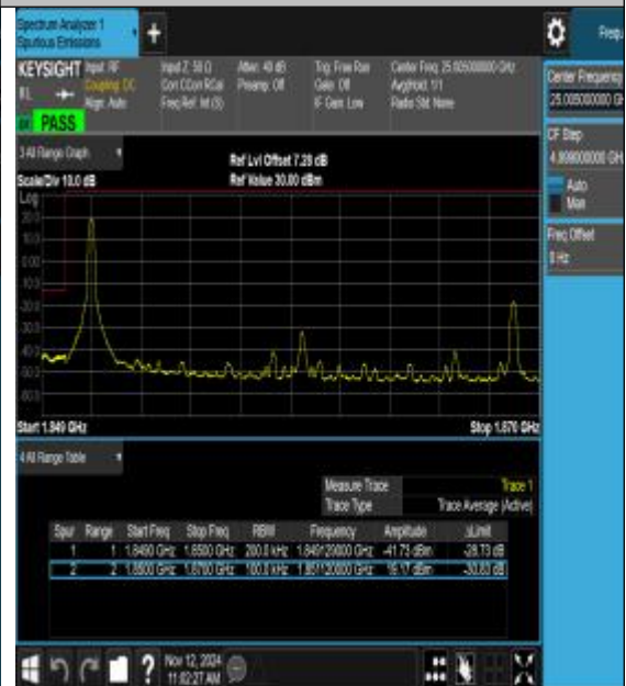
Band25_20MHz_16QAM_26140_1RB#0
