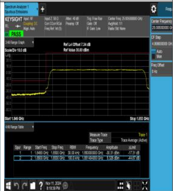
Band25_3MHz_16QAM_26055_15RB#0
