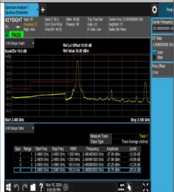
Band41_10MHz_16QAM_39700_1RB#0
