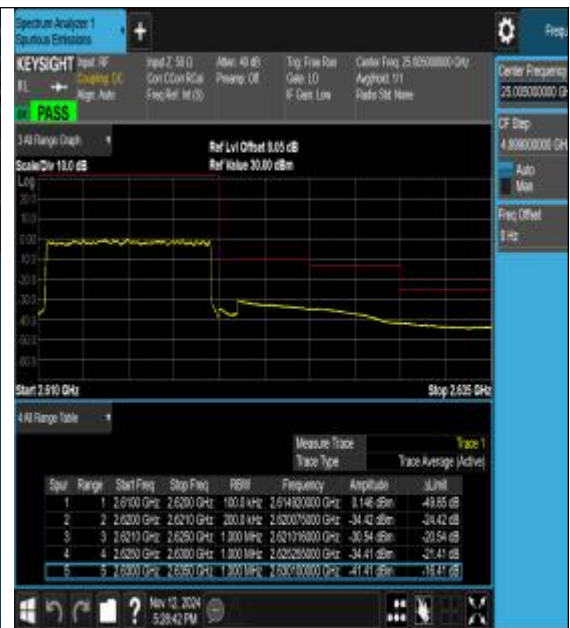
Band38_10MHz_16QAM_38200_50RB#0
