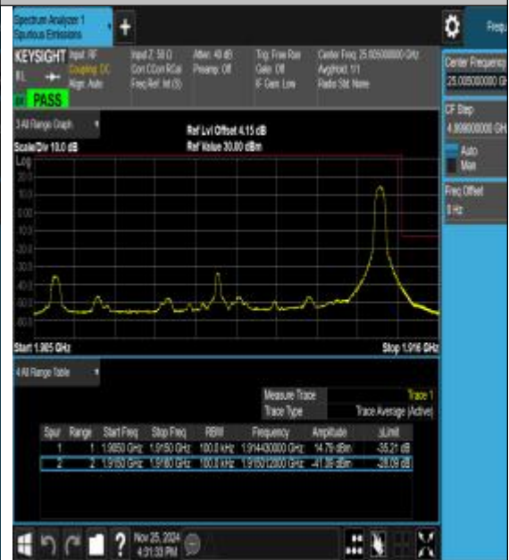
Band25_10MHz_16QAM_26640_1RB#49
