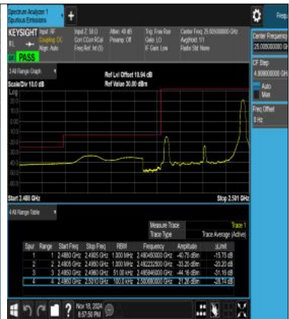
Band41_5MHz_16QAM_39675_1RB#24
