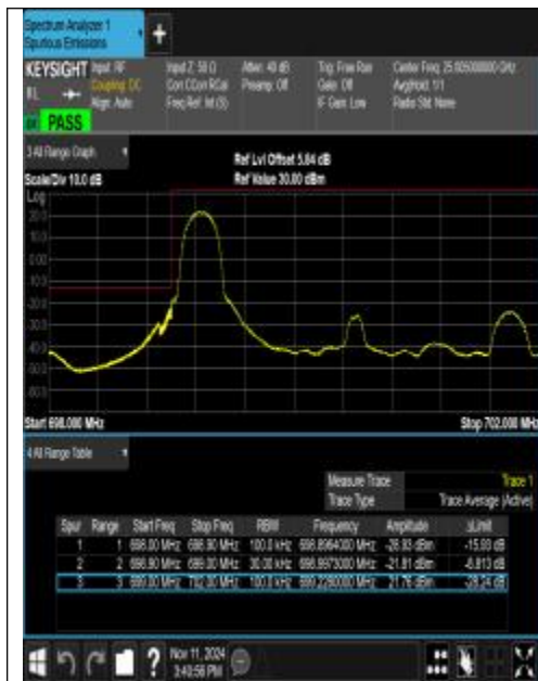
Band12_3MHz_QPSK_23025_1RB#0
