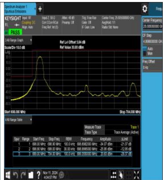
Band12_5MHz_16QAM_23035_1RB#0
