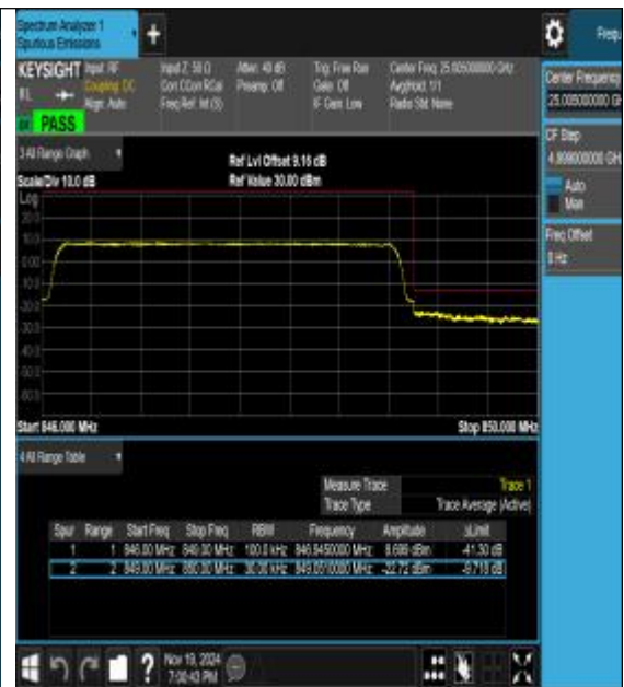
Band26_3MHz_16QAM_27025_15RB#0
