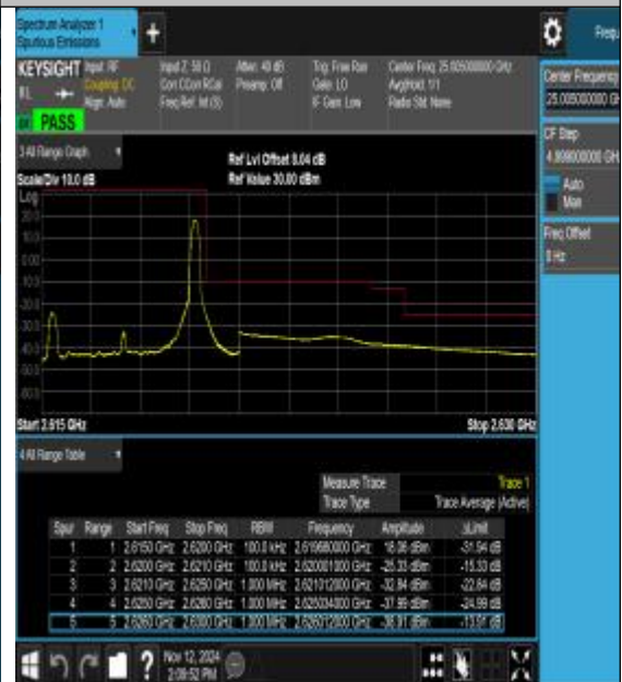
Band38_5MHz_16QAM_38225_1RB#24
