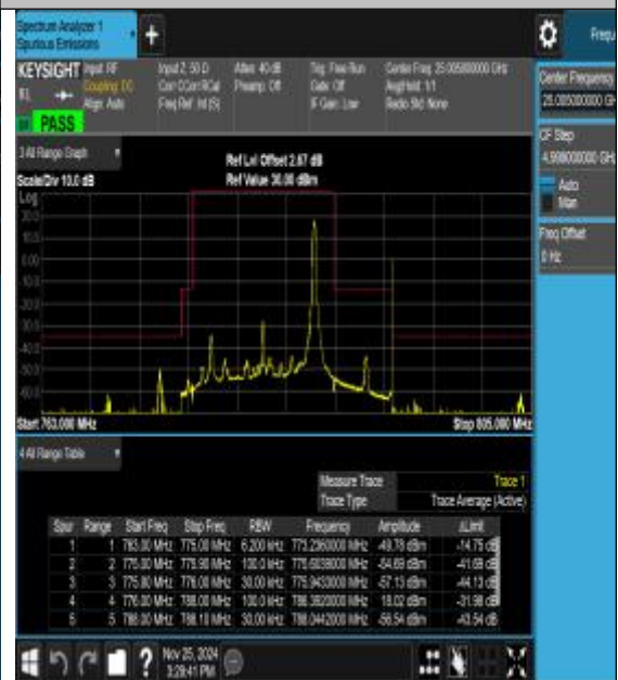
Band13_10MHz_16QAM_23230_1RB#49
