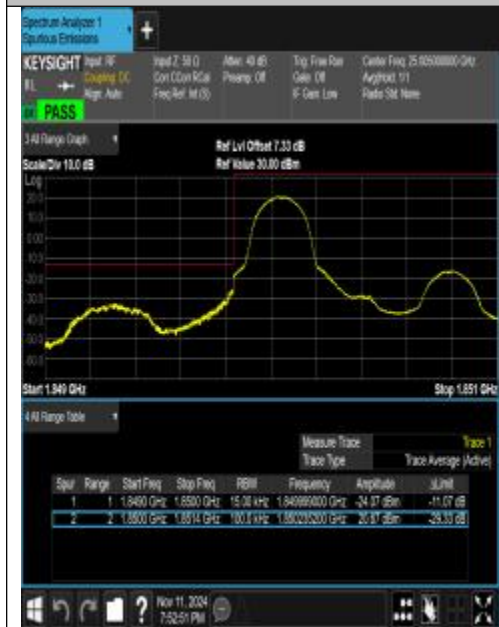
Band25_1.4MHz_QPSK_26047_1RB#0
