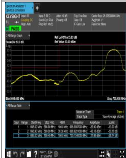
Band12_1.4MHz_QPSK_23017_1RB#5
