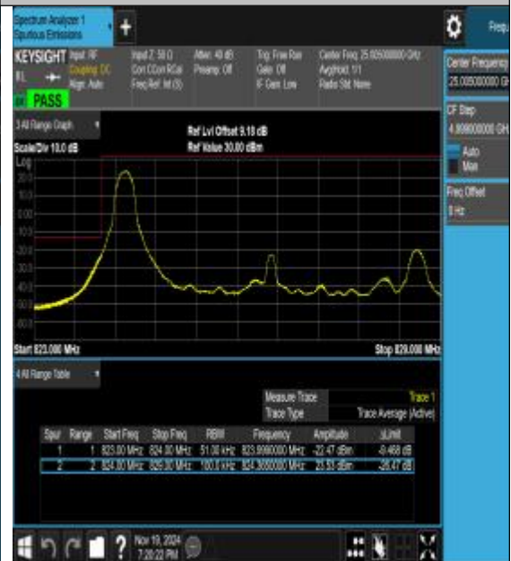
Band26_5MHz_16QAM_26815_1RB#0
