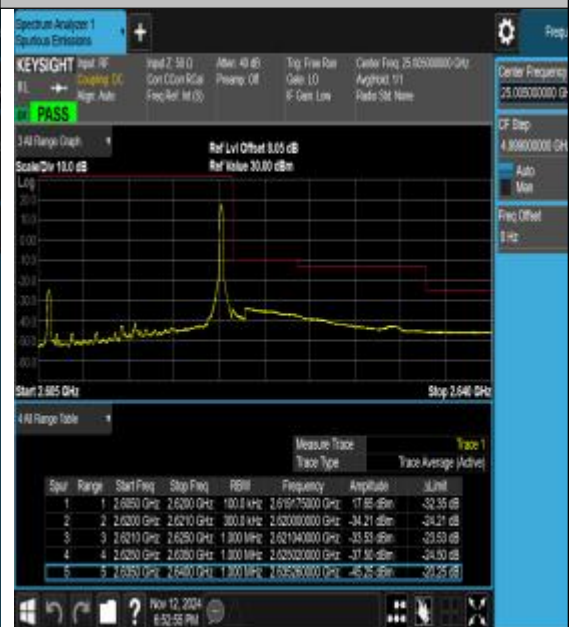
Band38_15MHz_16QAM_38175_1RB#74
