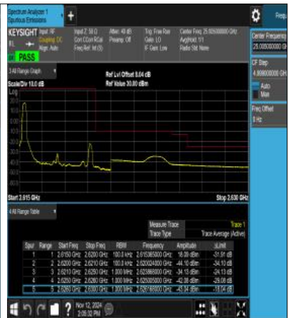
Band38_5MHz_16QAM_38225_1RB#0
