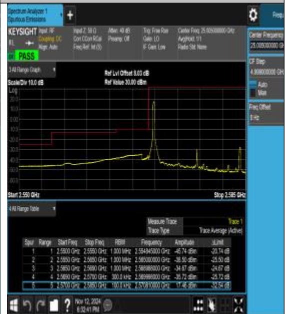
Band38_15MHz_16QAM_37825_1RB#0
