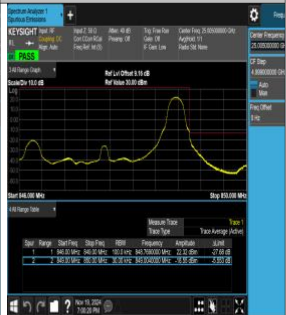
Band26_3MHz_16QAM_27025_1RB#14
