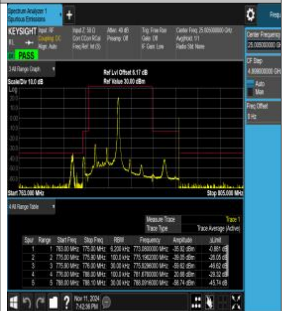
Band13_5MHz_16QAM_23205_1RB#24
