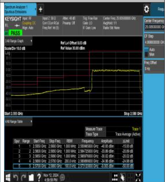
Band38_10MHz_16QAM_37800_1RB#0
