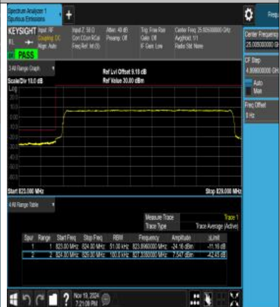
Band26_5MHz_16QAM_26815_25RB#0
