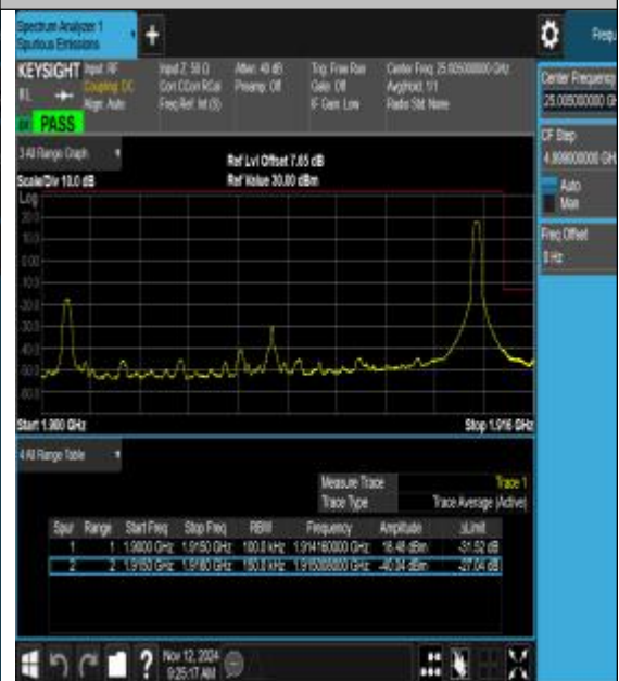
Band25_15MHz_16QAM_26615_1RB#74
