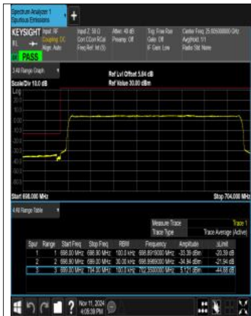
Band12_5MHz_QPSK_23035_25RB#0
