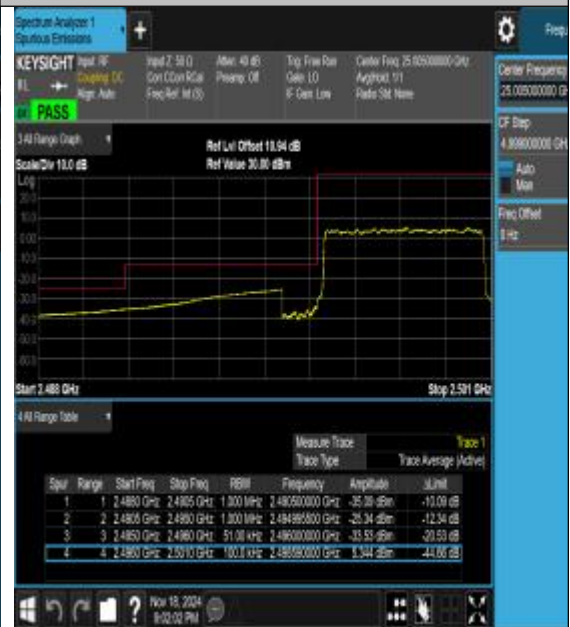
Band41_5MHz_16QAM_39675_25RB#0
