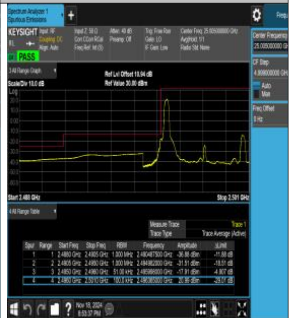
Band41_5MHz_16QAM_39675_1RB#0
