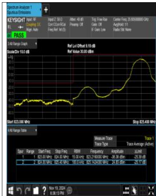
Band26_1.4MHz_QPSK_26797_1RB#5
