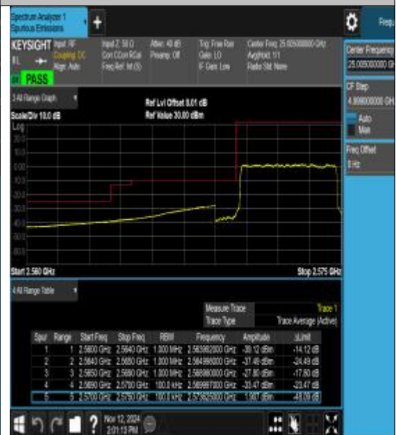
Band38_5MHz_16QAM_37775_25RB#0
