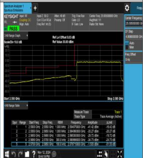
Band38_15MHz_16QAM_37825_75RB#0
