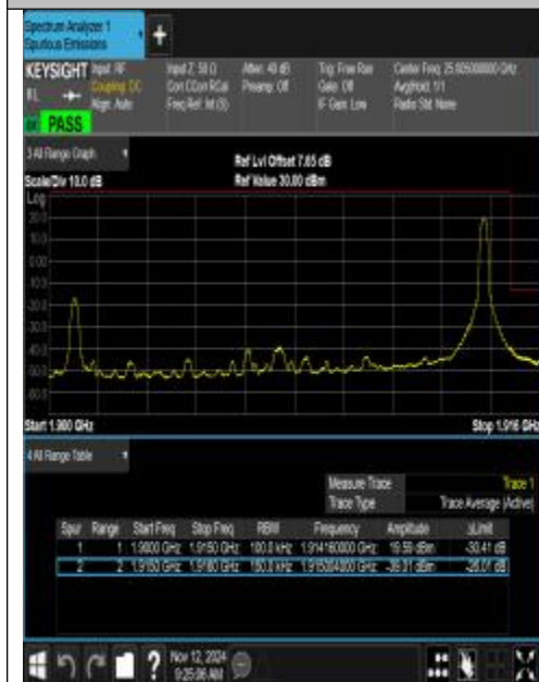
Band25_15MHz_QPSK_26615_1RB#74
