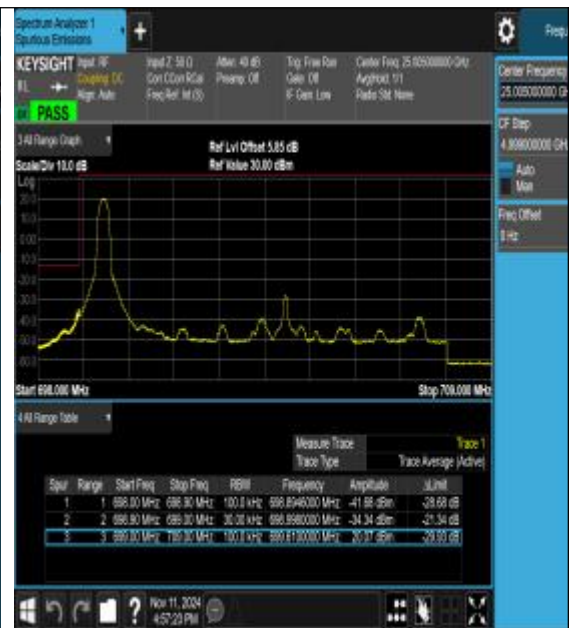
Band12_10MHz_16QAM_23060_1RB#0
