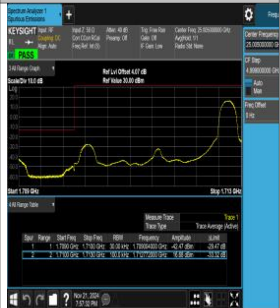
Band66_3MHz_16QAM_131987_1RB#14
