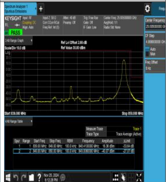
Band26_10MHz_16QAM_26990_1RB#49
