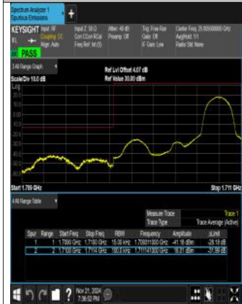
Band66_1.4MHz_QPSK_131979_1RB#5
