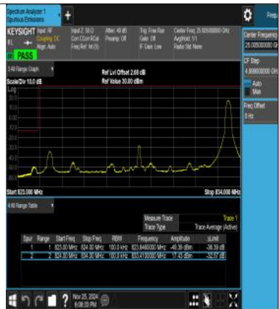
Band26_10MHz_16QAM_26840_1RB#49
