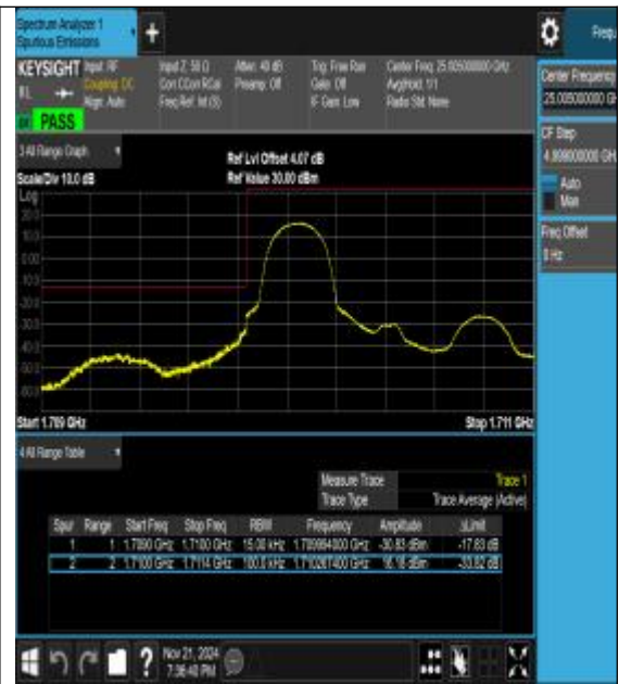
Band66_1.4MHz_16QAM_131979_1RB#0
