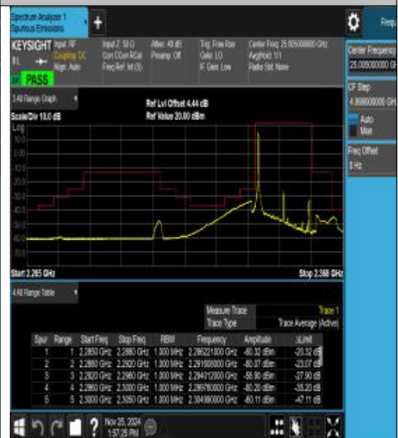
Band40_15MHz_16QAM_39175_1RB#0
