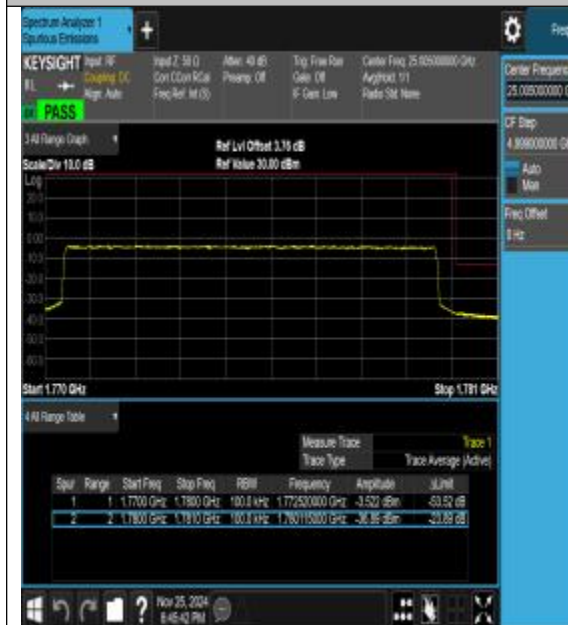
Band66_10MHz_QPSK_132622_50RB#0
