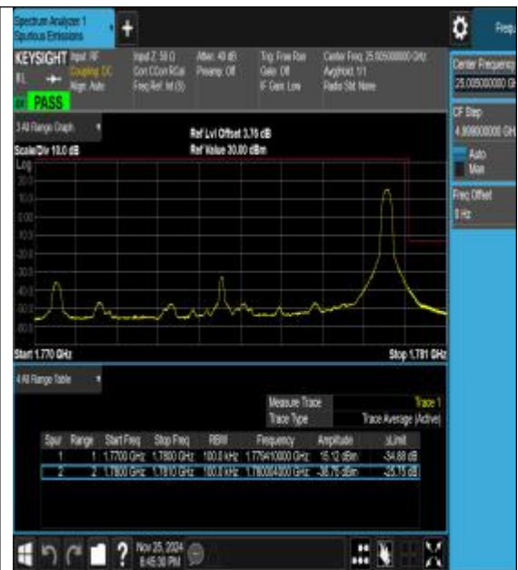
Band66_10MHz_16QAM_132622_1RB#49
