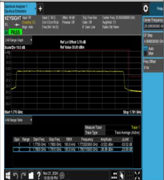
Band66_10MHz_16QAM_132622_50RB#0
