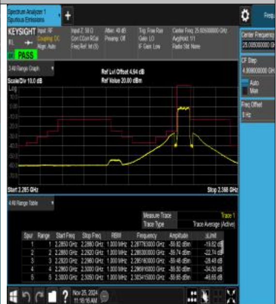
Band40_5MHz_16QAM_39125_25RB#0
