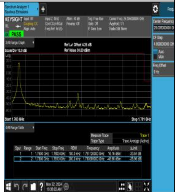
Band66_20MHz_16QAM_132572_1RB#0
