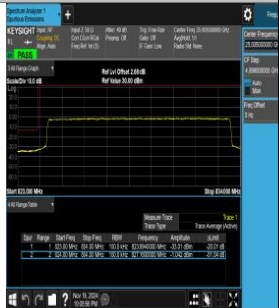
Band26_10MHz_16QAM_26840_50RB#0
