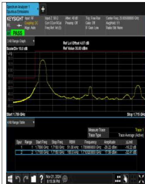
Band66_5MHz_QPSK_131997_1RB#0
