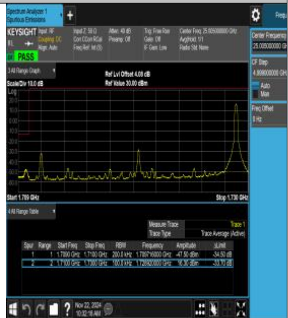
Band66_20MHz_16QAM_132072_1RB#99
