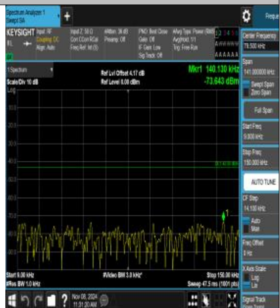
Band2_3MHz_16QAM_18615_1RB#0_0.009~0.15 0.009~0.15
