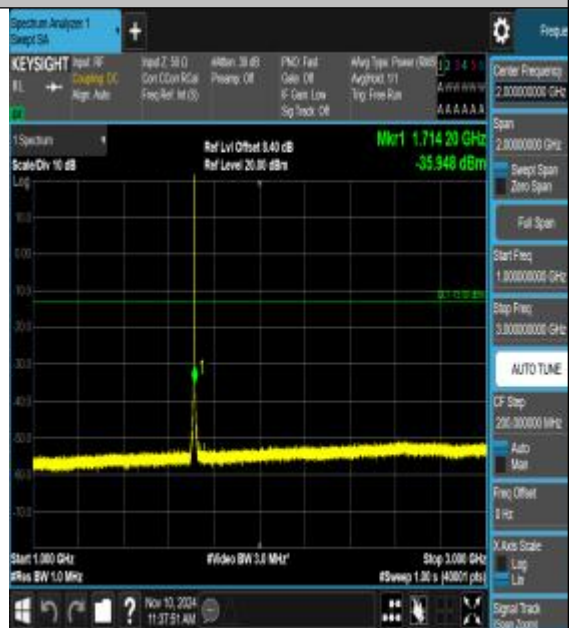
Band4_1.4MHz_QPSK_19957_1RB#0_1000~300 0_1000~3000
