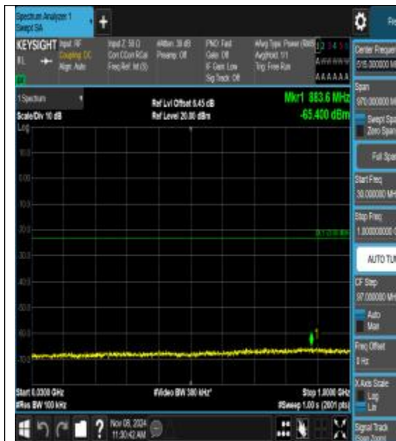
Band2_3MHz_QPSK_18615_1RB#0_30~1000_3 0~1000
