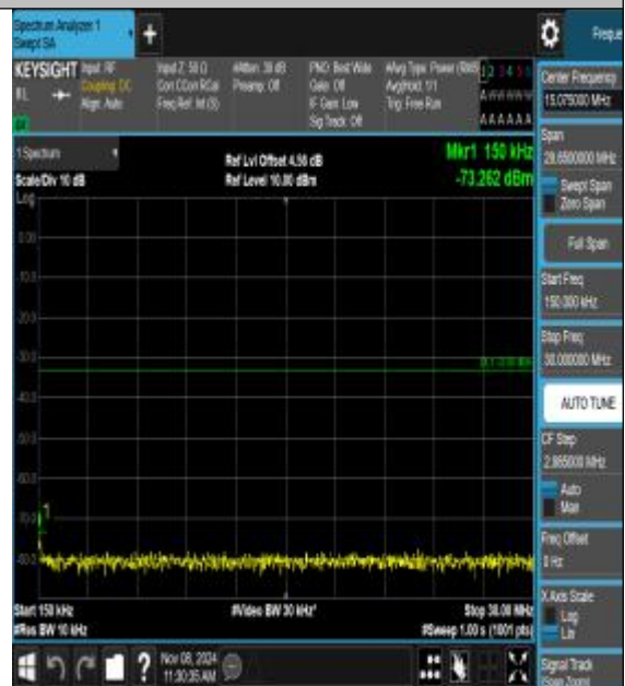
Band2_3MHz_QPSK_18615_1RB#0_0.15~30_0.15~30_5~30
