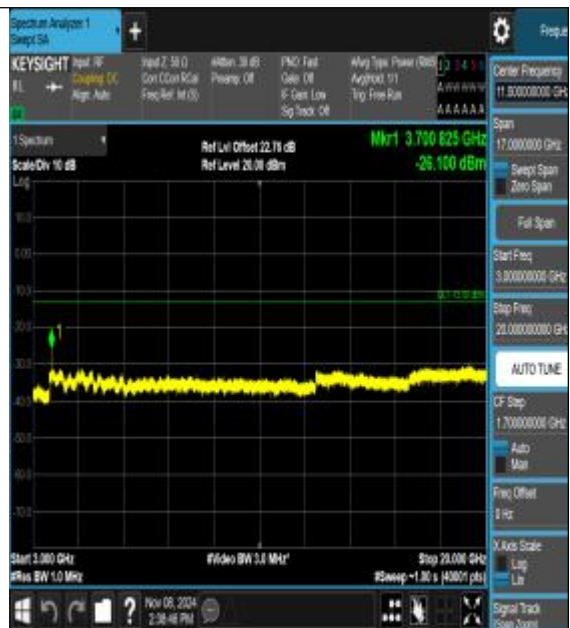
Band2_5MHz_16QAM_18625_1RB#0_3000~20000_0_3000~20000
