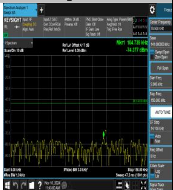
Band4_1.4MHz_16QAM_20175_1RB#0_0.009~0.15_15_0.009~0.15
