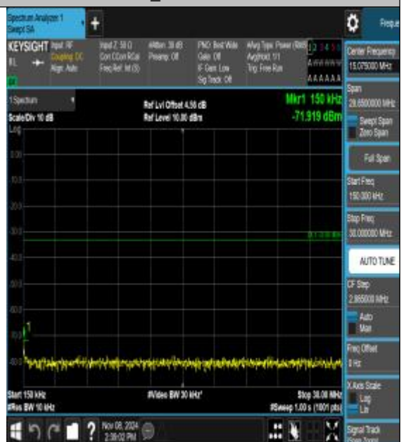
Band2_5MHz_QPSK_18900_1RB#0_0.15~30_0.15~30_5~30
