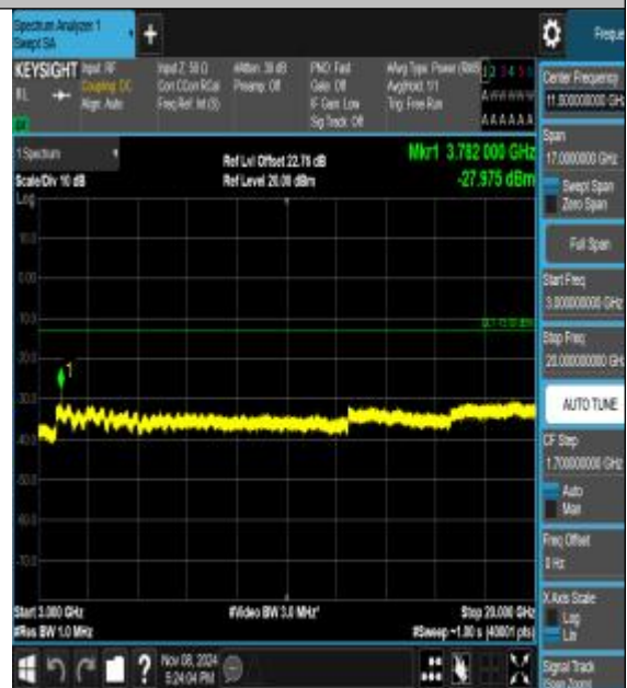
Band2_20MHz_16QAM_19100_1RB#0_3000~20000_3000~20000
