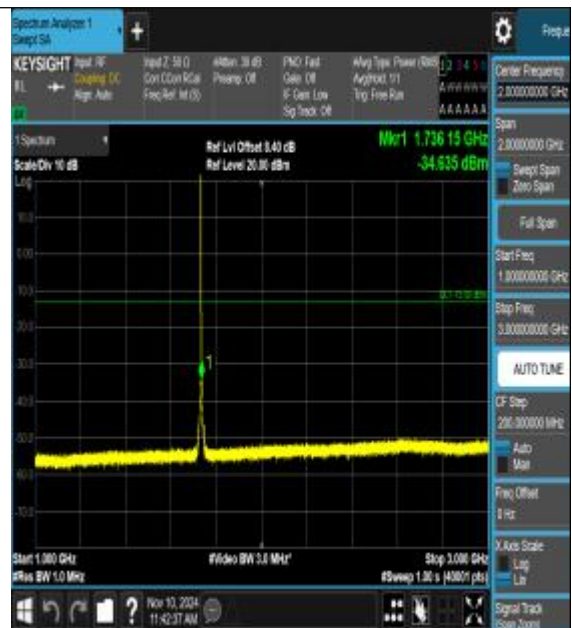
Band4_1.4MHz_QPSK_20175_1RB#0_1000~3000_0_1000~3000
