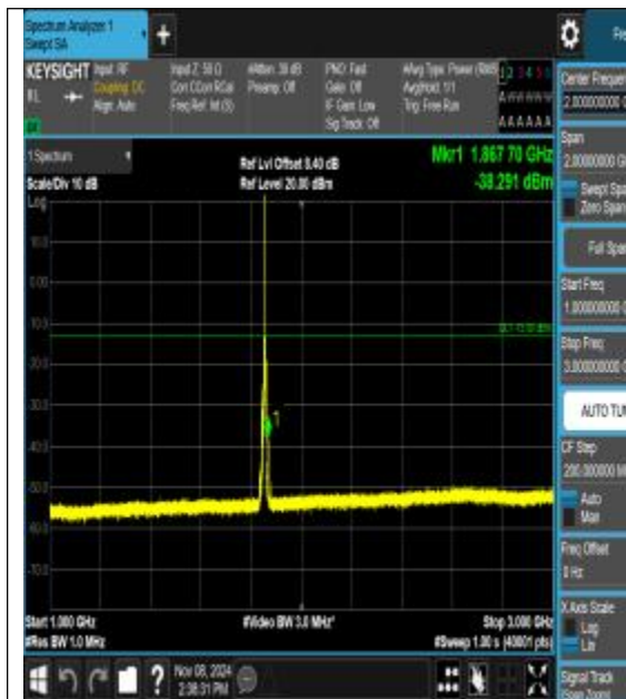
Band2_5MHz_16QAM_18625_1RB#0_1000~3000_1000~3000
