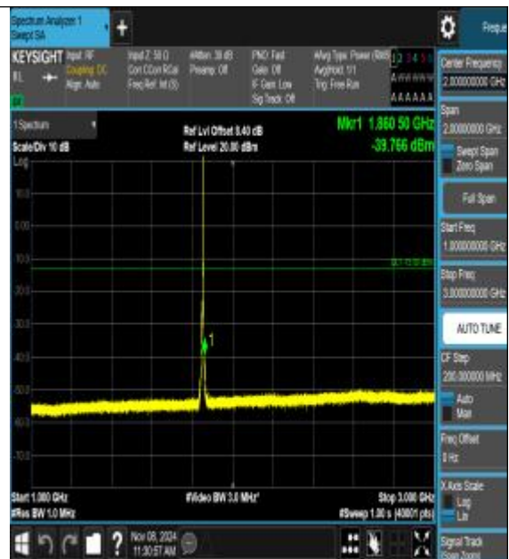
Band2_3MHz_QPSK_18615_1RB#0_1000~3000_1000~3000
