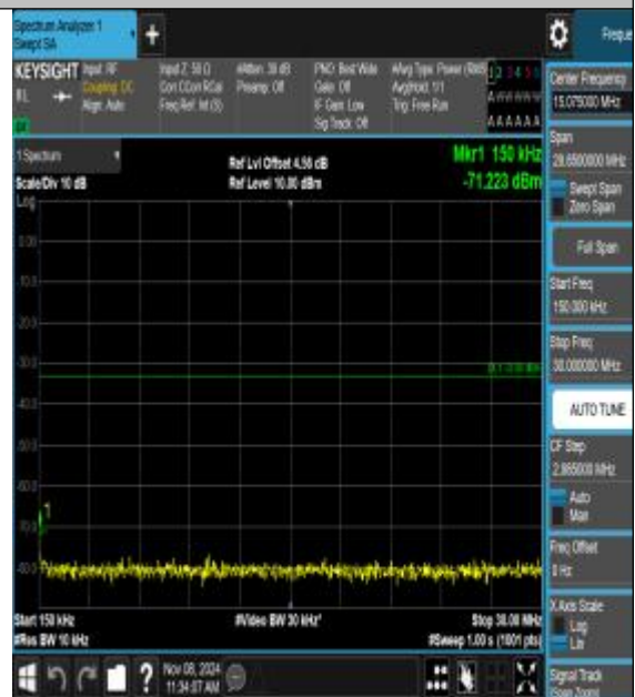
Band2_3MHz_QPSK_19185_1RB#0_0.15~30_0.15~30_5~30
