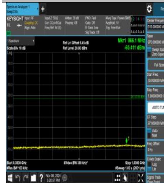
Band2_20MHz_QPSK_18900_1RB#0_30~1000_ 30~1000
