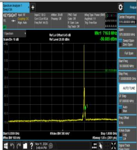
Band12_3MHz_16QAM_23095_1RB#0_30~1000_30~1000
