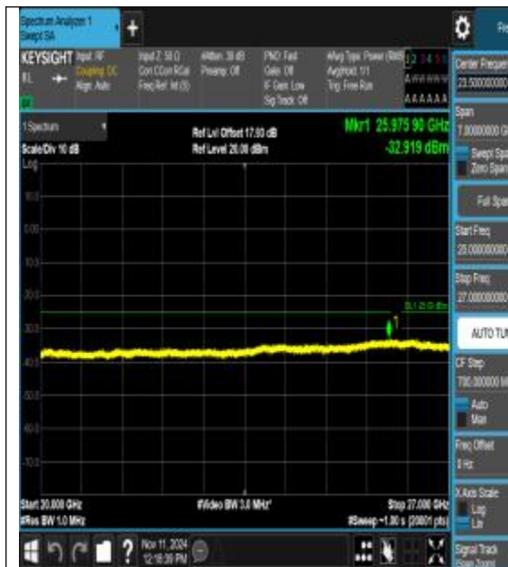
Band7_15MHz_QPSK_21375_1RB#0_20000~27000_000_20000~27000
