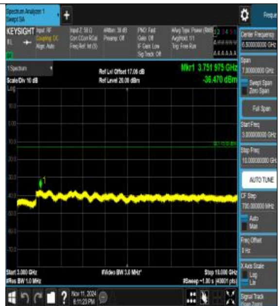
Band13_5MHz_16QAM_23205_1RB#0_3000~10000_3000~10000
