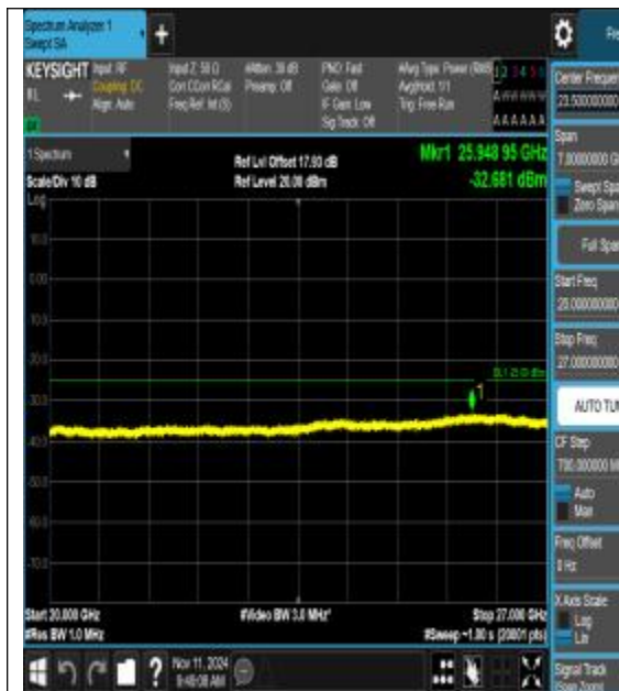
Band7_5MHz_QPSK_20775_1RB#0_20000~27000_20000~27000
