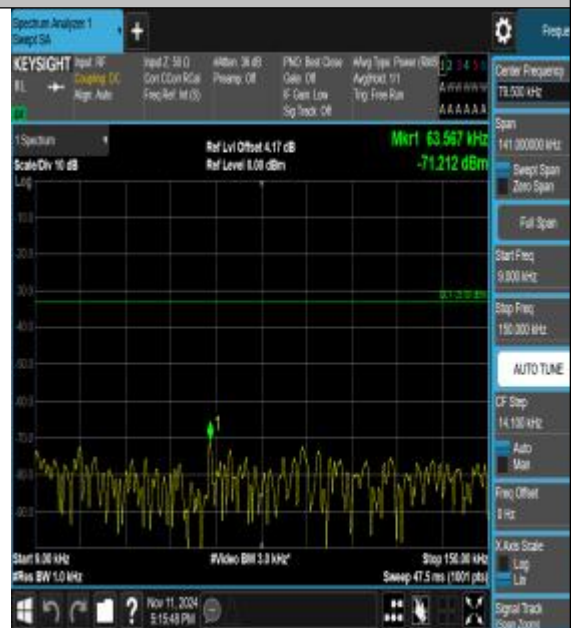
Band12_10MHz_16QAM_23060_1RB#0_0.009~0.15_0.009~0.15
