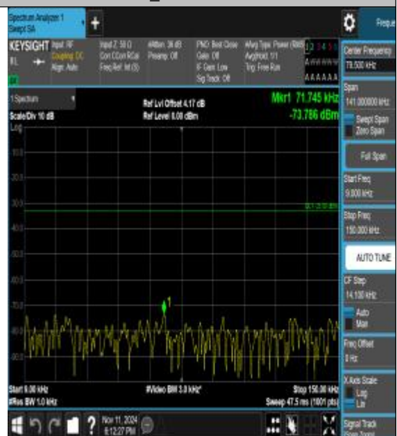
Band13_5MHz_16QAM_23230_1RB#0_0.009~0.15_5_0.009~0.15
