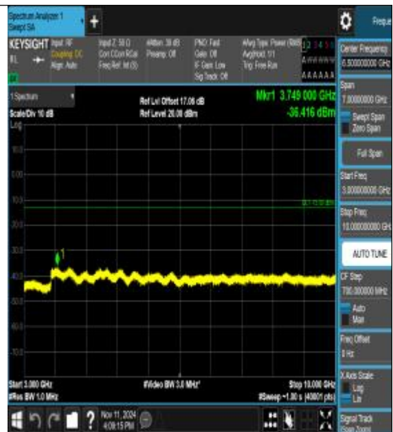
Band12_5MHz_16QAM_23035_1RB#0_3000~10000_3000~10000
