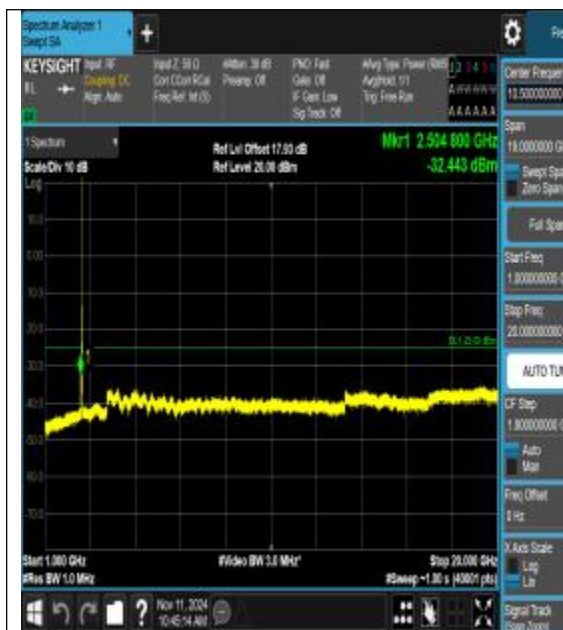
Band7_10MHz_16QAM_21100_1RB#0_1000~20000
