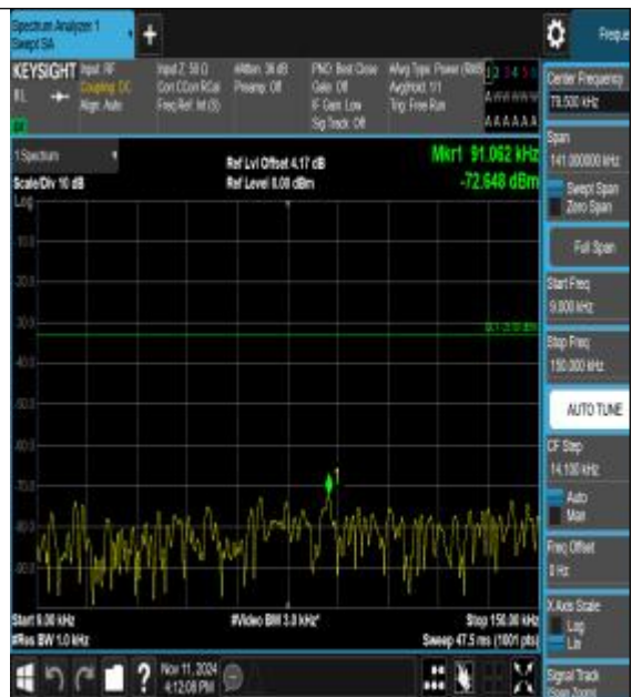
Band12_5MHz_16QAM_23155_1RB#0_0.009~0.15
