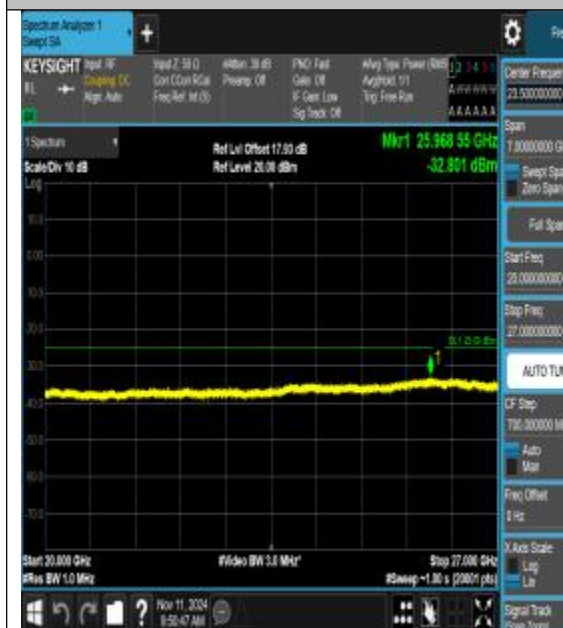
Band7_5MHz_QPSK_21100_1RB#0_20000~27000 00 20000~27000
