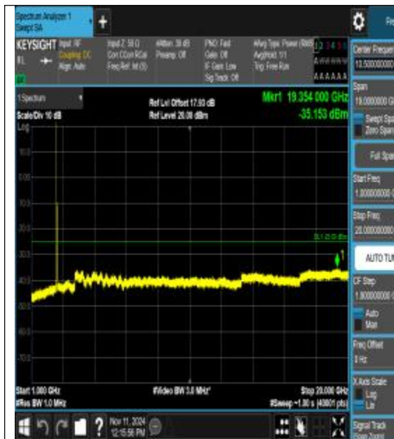
Band7_15MHz_16QAM_20825_1RB#0_1000~20000_000_1000~20000
