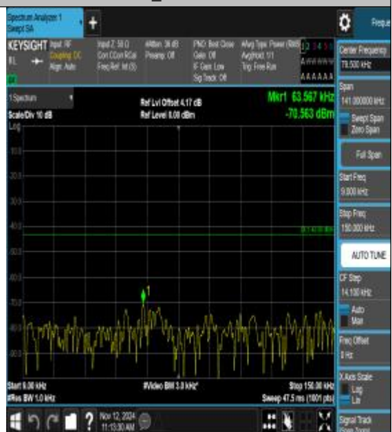
Band38_10MHz_16QAM_37800_1RB#0_0.009~0.15_15_0.009~0.15
