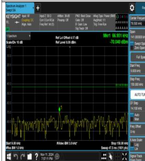
Band25_1.4MHz_QPSK_26365_1RB#0_0.009~0.15_15_0.009~0.15
