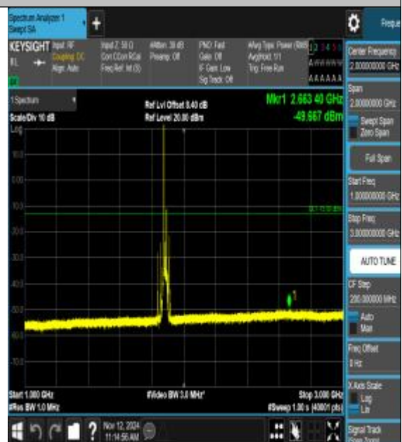
Band25_20MHz_QPSK_26365_1RB#0_1000~300 0_1000~3000
