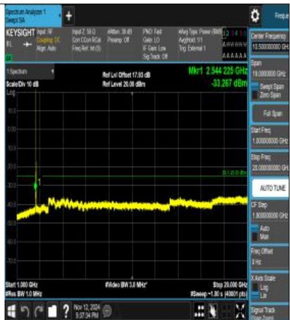
Band38_10MHz_QPSK_37800_1RB#0_1000~20000_00_1000~20000
