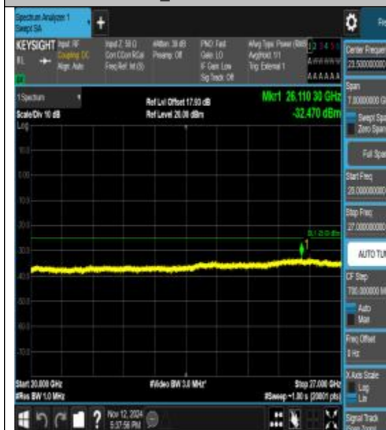
Band38_10MHz_QPSK_37800_1RB#0_20000~27000_7000_20000~27000
