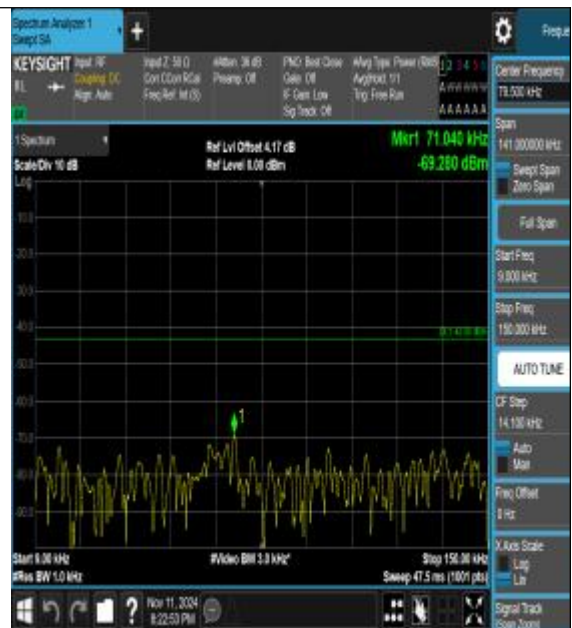
Band25_3MHz_16QAM_26365_1RB#0_0.009~0.15_5_0.009~0.15
