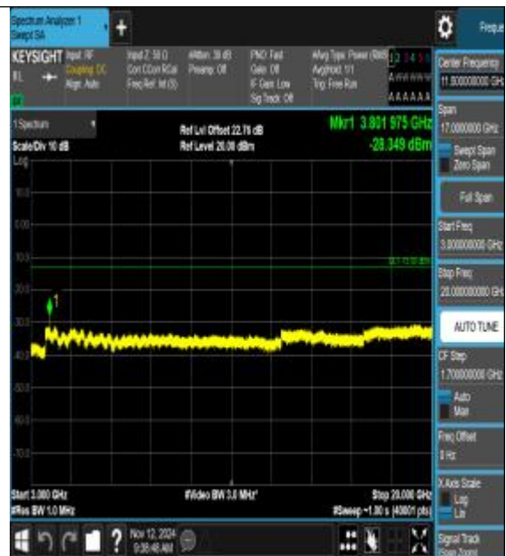
Band25_15MHz_16QAM_26615_1RB#0_3000~20000_3000~20000
