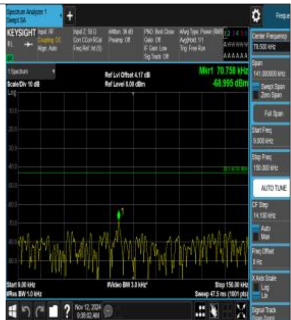
Band25_15MHz_16QAM_26615_1RB#0_0.009~0.15_0.009~0.15
