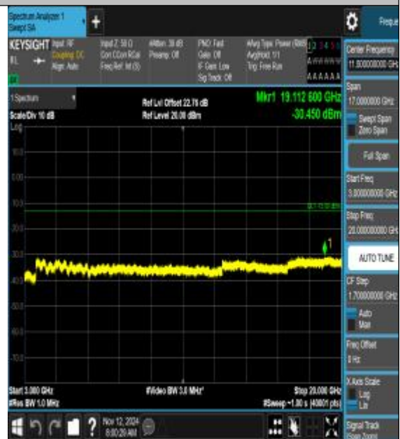
Band25_10MHz_16QAM_26090_1RB#0_3000~20 000_3000~20000
