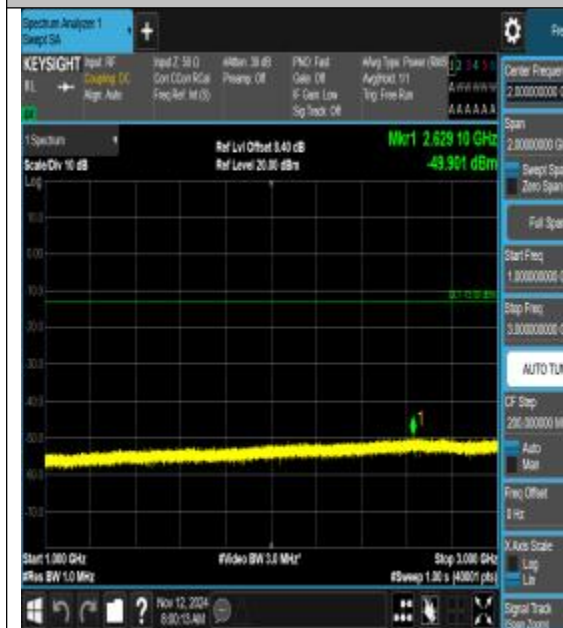
Band25_10MHz_16QAM_26090_1RB#0_1000~3 000_1000~3000
