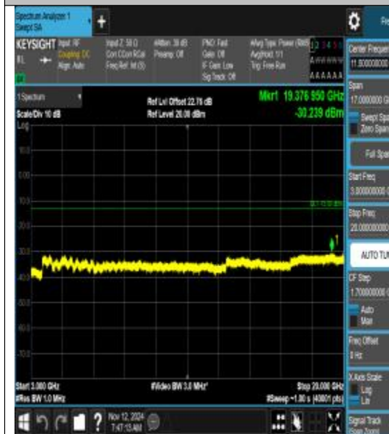
Band25_10MHz_QPSK_26090_1RB#0_3000~20000_000_3000~20000
