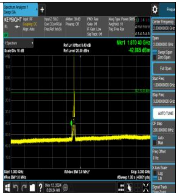
Band25_10MHz_QPSK_26640_1RB#0_1000~300 0_1000~3000
