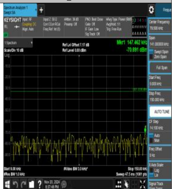
Band41_10MHz_16QAM_39700_1RB#0_0.009~0.15_15_0.009~0.15
