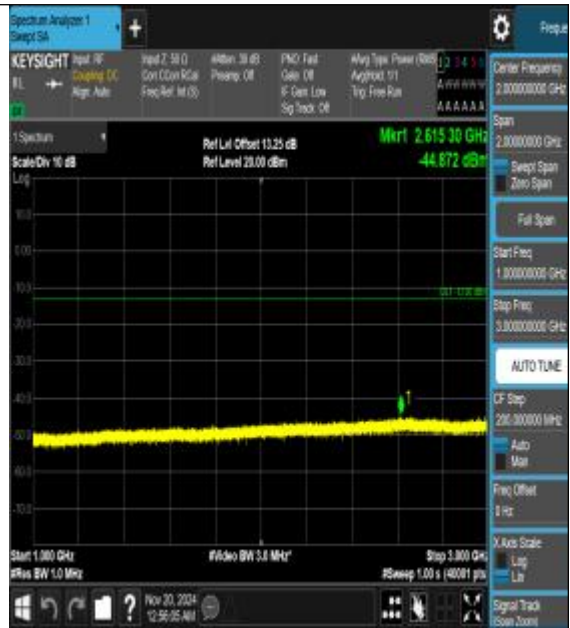
Band26_10MHz_QPSK_26990_1RB#0_1000~3000_0_1000~3000
