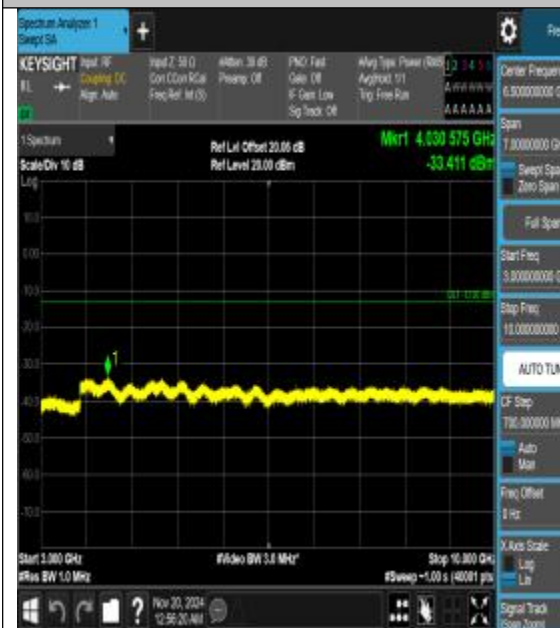
Band26_10MHz_QPSK_26990_1RB#0_3000~10000_000_3000~10000
