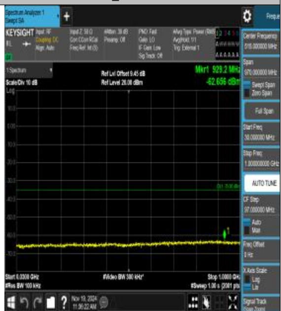
Band41_20MHz_16QAM_40620_1RB#0_30~1000_30~1000
