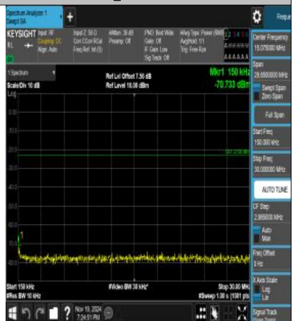
Band26_5MHz_QPSK_26915_1RB#0_0.15~30_0.15~30_15~30
