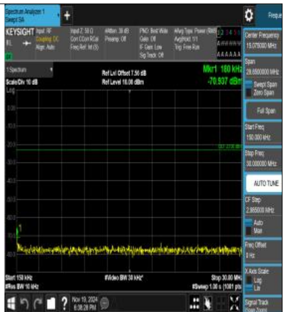
Band26_1.4MHz_QPSK_26797_1RB#0_0.15~30_0.15~30
