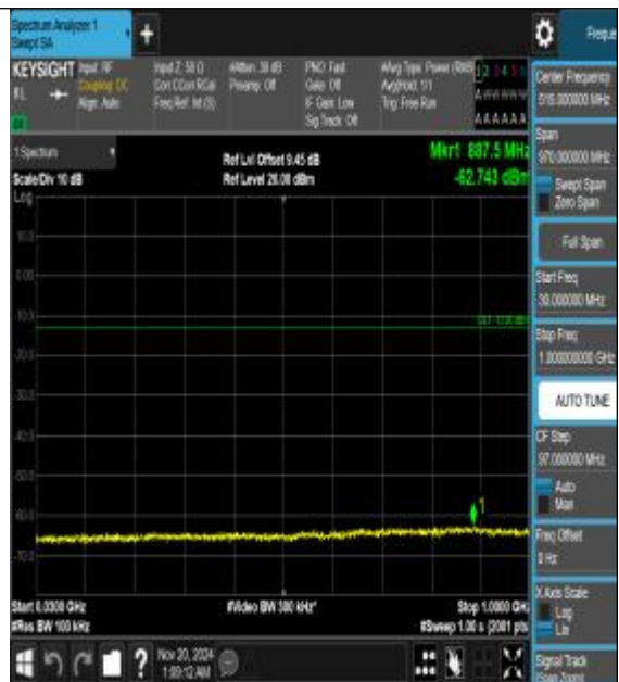
Band26_10MHz_16QAM_26990_1RB#0_30~1000 _30~1000
