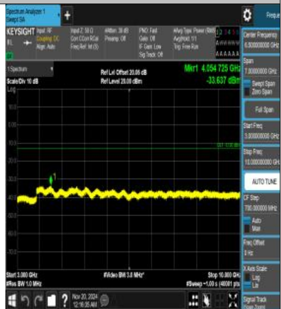
Band26_10MHz_16QAM_26840_1RB#0_3000~10 000_3000~10000
