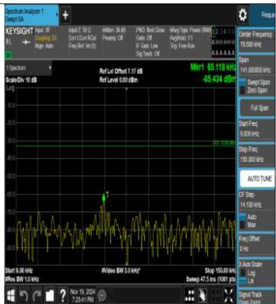
Band26_5MHz_16QAM_26815_1RB#0_0.009~0.15_5_0.009~0.15
