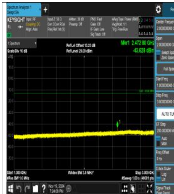
Band26_5MHz_16QAM_26815_1RB#0_1000~3000_1000~3000
