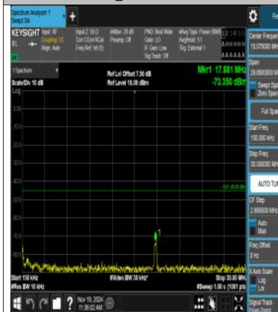
Band41_20MHz_16QAM_40620_1RB#0_0.15~30_0.15~30
