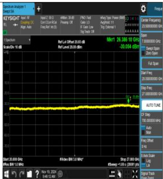
Band41_15MHz_16QAM_39725_1RB#0_20000~27000
