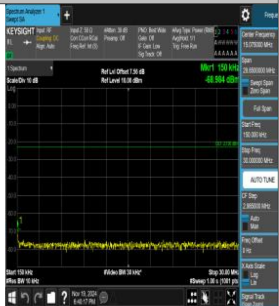
Band26_1.4MHz_QPSK_26915_1RB#0_0.15~30_0.15~30
