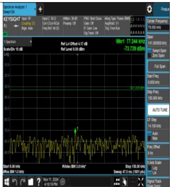
Band41_20MHz_16QAM_40620_1RB#0_0.009~0.15_0.009~0.15
