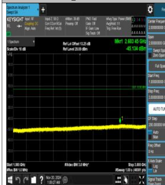
Band26_10MHz_16QAM_26990_1RB#0_1000~3 000_1000~3000
