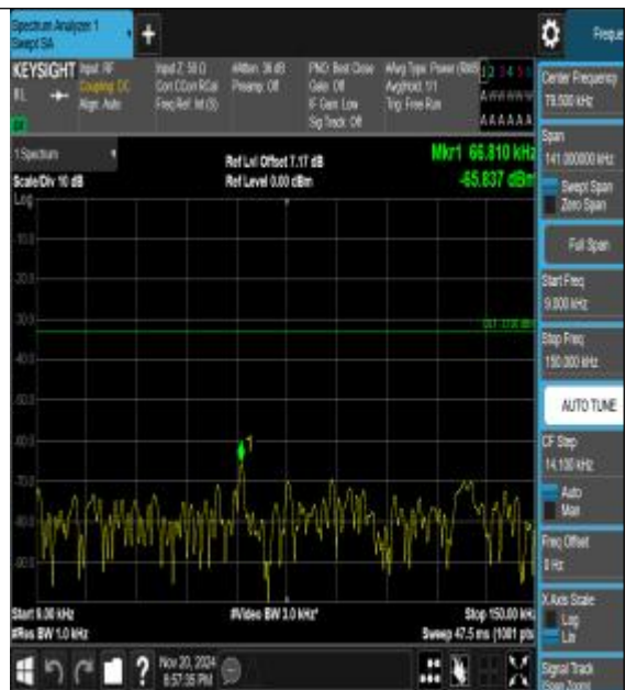
Band41_15MHz_16QAM_39725_1RB#0_0.009~0.15_0.009~0.15
