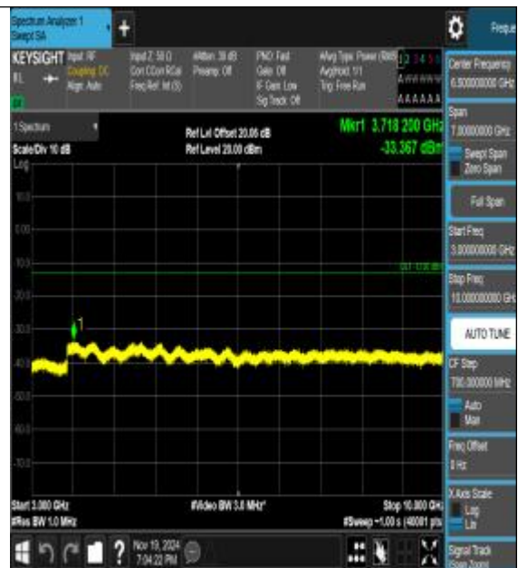
Band26_3MHz_16QAM_26915_1RB#0_3000~10000_3000~10000
