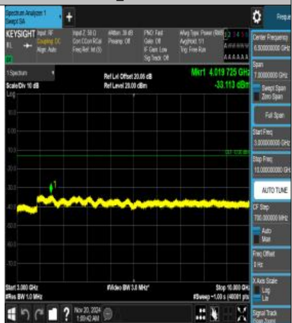
Band26_10MHz_16QAM_26990_1RB#0_3000~10 000_3000~10000
