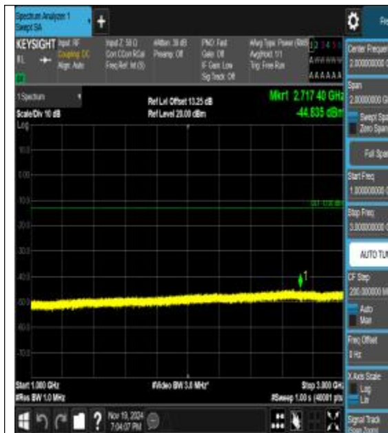
Band26_3MHz_16QAM_26915_1RB#0_1000~3000_1000~3000
