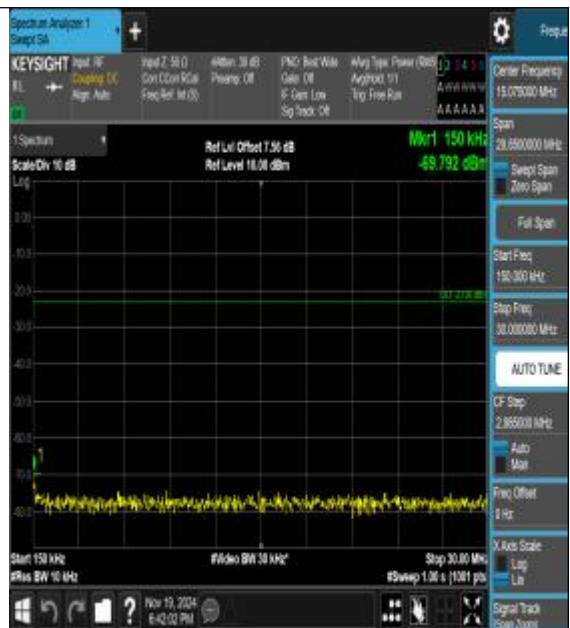
Band26_1.4MHz_QPSK_27033_1RB#0_0.15~30_0.15~30
