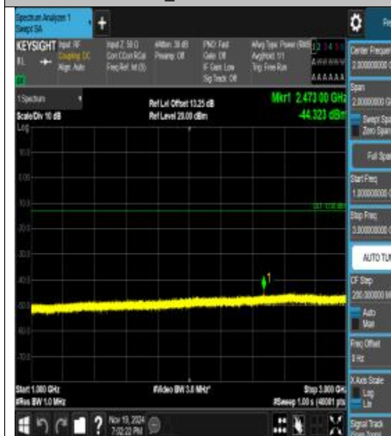
Band26_3MHz_16QAM_26805_1RB#0_1000~3000_1000~3000
