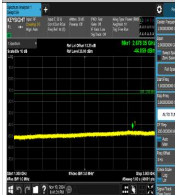
Band26_1.4MHz_16QAM_26915_1RB#0_1000~ 3000_1000~3000
