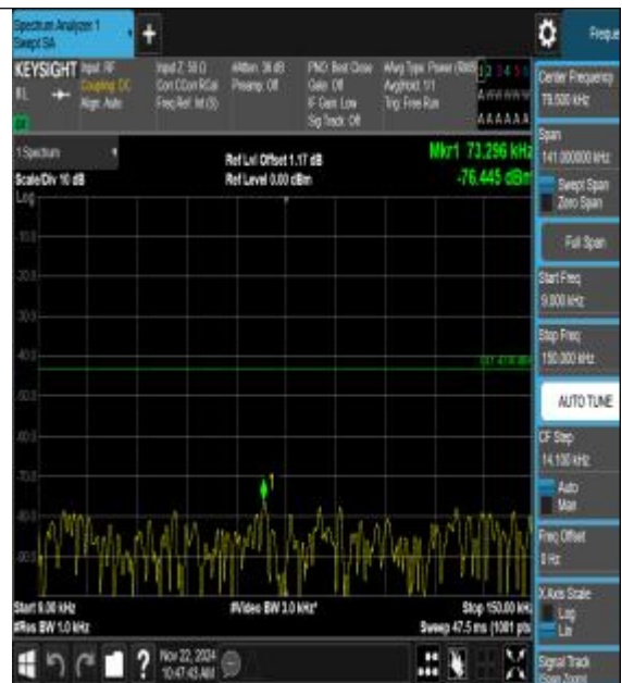
Band66_20MHz_16QAM_132572_1RB#0_0.009~0.15
