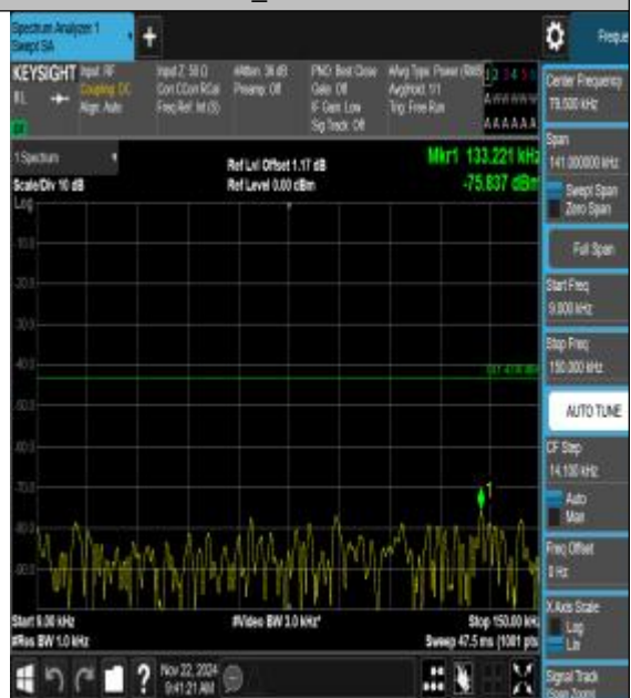
Band66_15MHz_16QAM_132597_1RB#0_0.009~ 0.15 0.009~0.15
