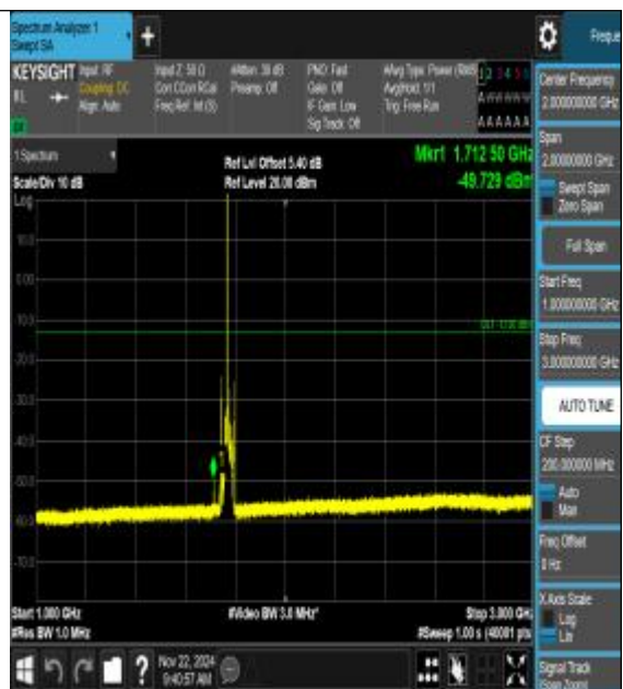
Band66_15MHz_QPSK_132597_1RB#0_1000~3000
