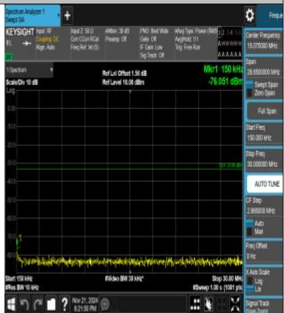
Band66_5MHz_QPSK_132647_1RB#0_0.15~30_0.15~30
