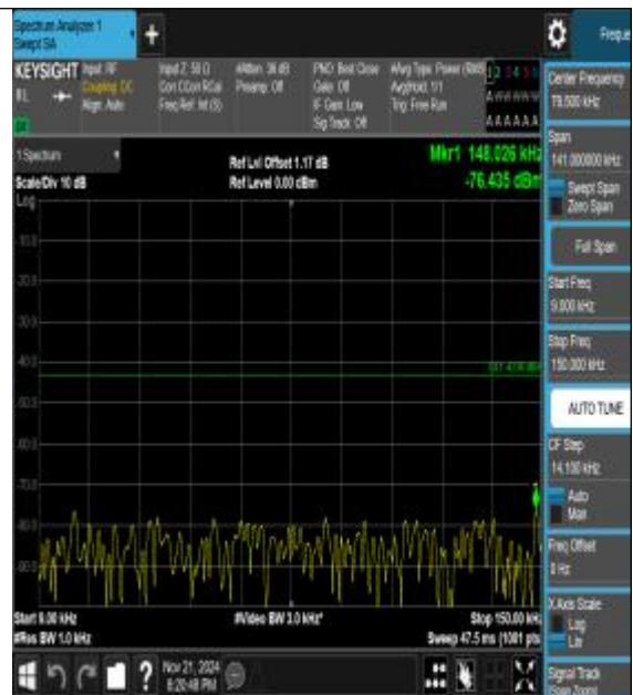
Band66_5MHz_16QAM_132322_1RB#0_0.009~0.15_15_0.009~0.15
