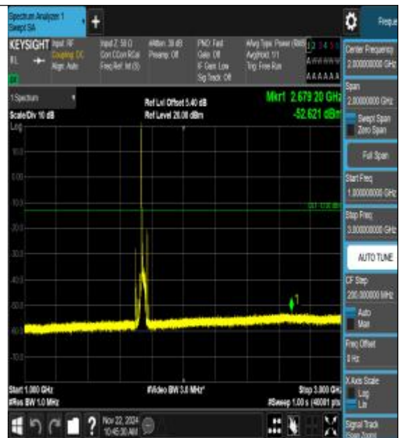
Band66_20MHz_QPSK_132322_1RB#0_1000~30 00_1000~3000
