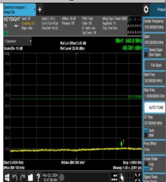
Band66_20MHz_16QAM_132572_1RB#0_30~1000
