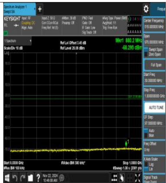
Band66_20MHz_16QAM_132322_1RB#0_30~1000_30~1000
