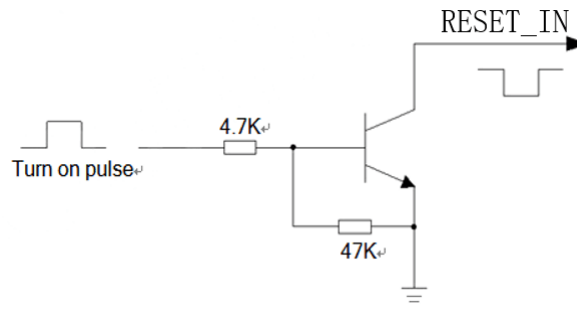
Chart9 Hardware Reset Reference Circuit
