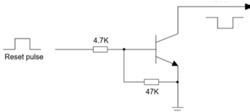
Chart5 Open set driver reference power-up circuit
