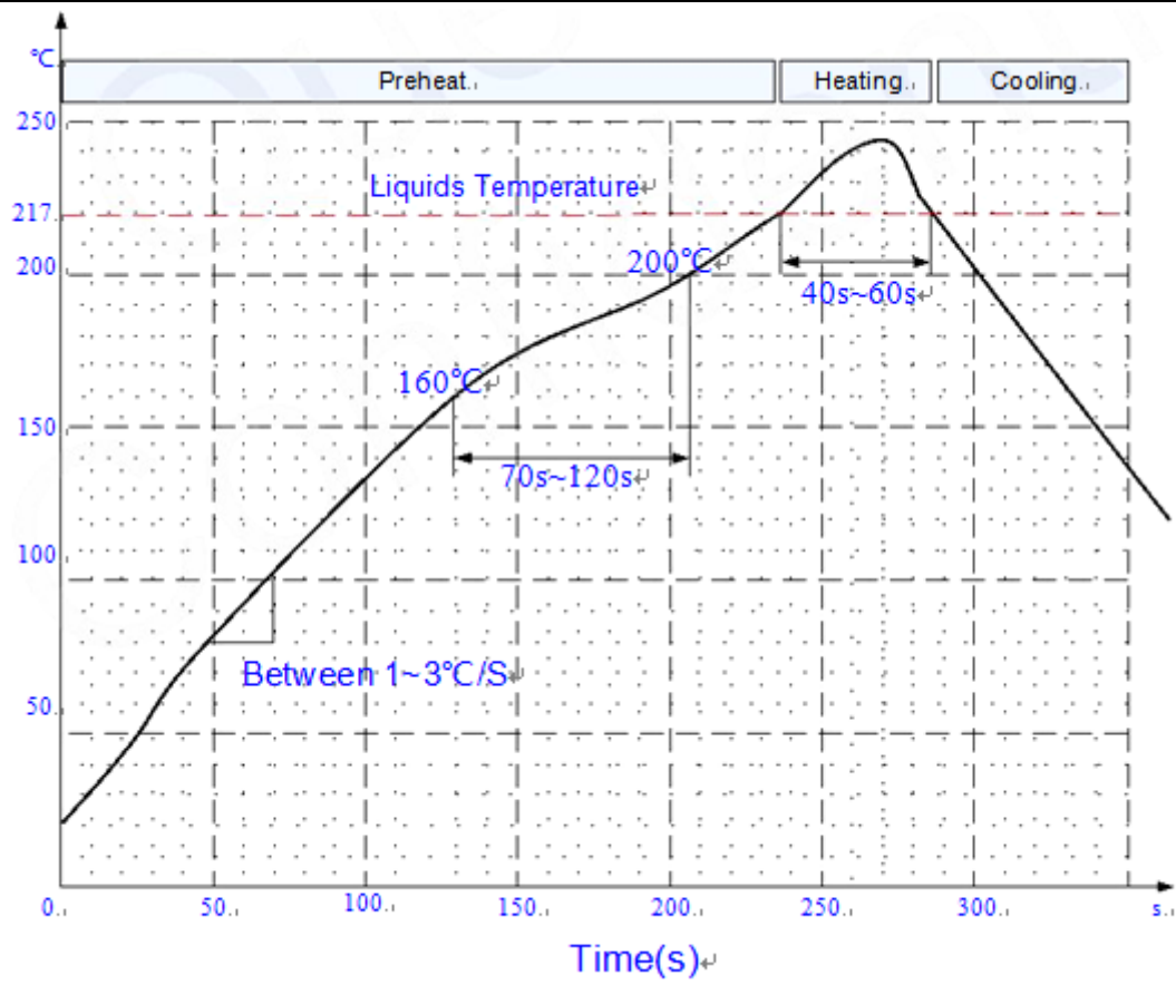
Chart22 Furnace Temperature Curve
