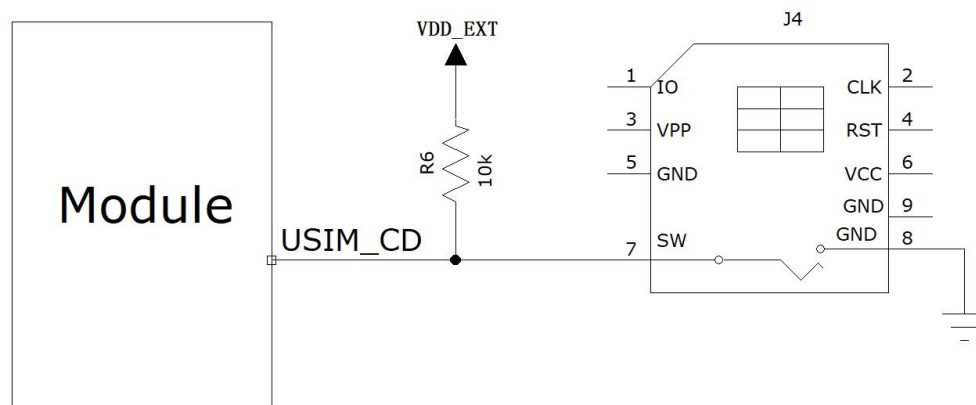
Diagram16 Reference Circuit Diagram for SIM Card Holder Using Band Detection PIN
