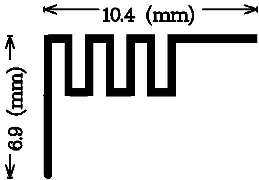
Antenna Photo & Length (mm)
