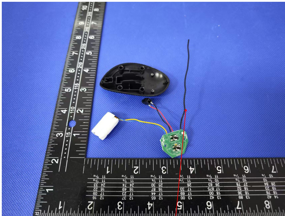
Internal antenna
