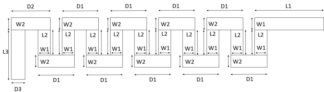
Antenna Dimensions
