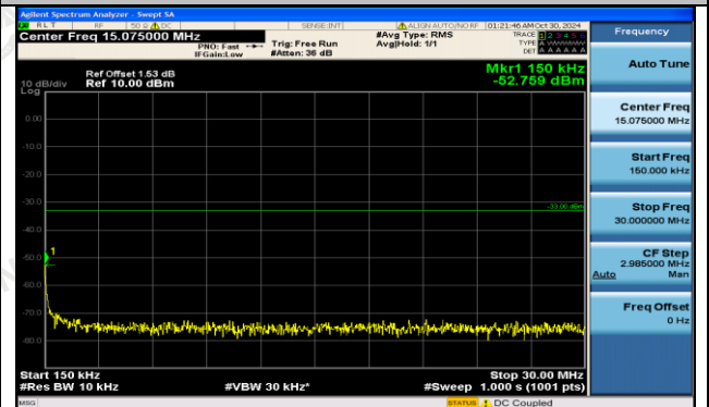
Band2-9400-0.15~30MHz-PASS
