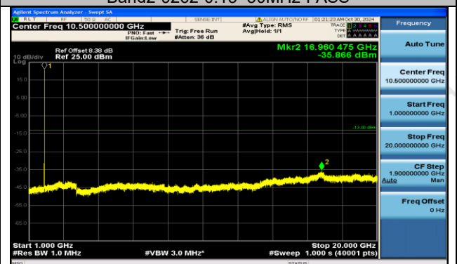
Band2-9262-1000~20000MHz-PASS
