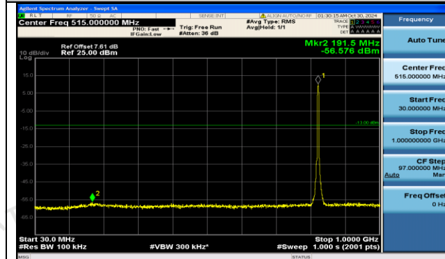
Band5-4132-30~1000MHz-PASS
