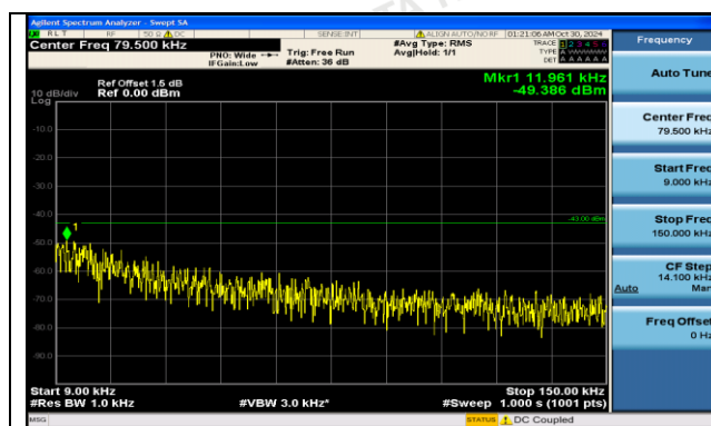
Band2-9262-0.009~0.15MHz-PASS
