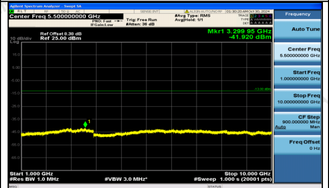
Band5-4132-1000~10000MHz-PASS
