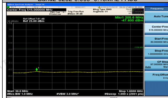
Band2-9262-30~1000MHz-PASS
