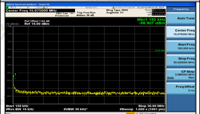
Band5-4182-0.15~30MHz-PASS
