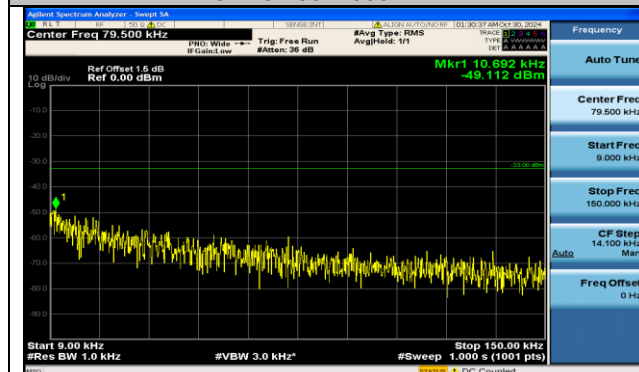
Band5-4182-0.009~0.15MHz-PASS
