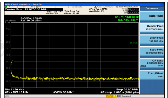
Band5-4132-0.15~30MHz-PASS
