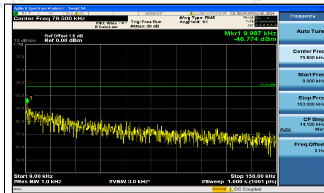
Band5-4132-0.009~0.15MHz-PASS
