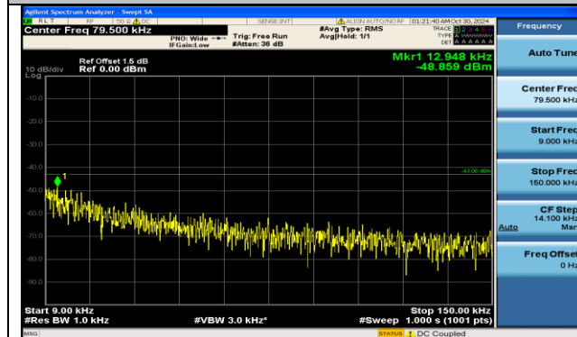
Band2-9400-0.009~0.15MHz-PASS
