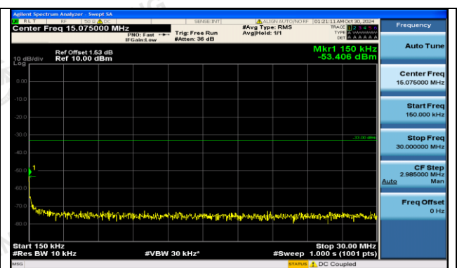
Band2-9262-0.15~30MHz-PASS
