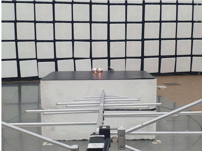
[Rear view of Radiated Emission (Below 1GHz)]
