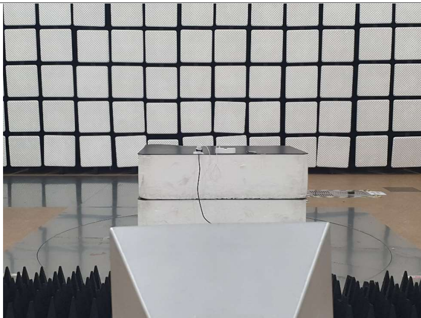
[Rear view of Radiated Emission (Above 1GHz)]
