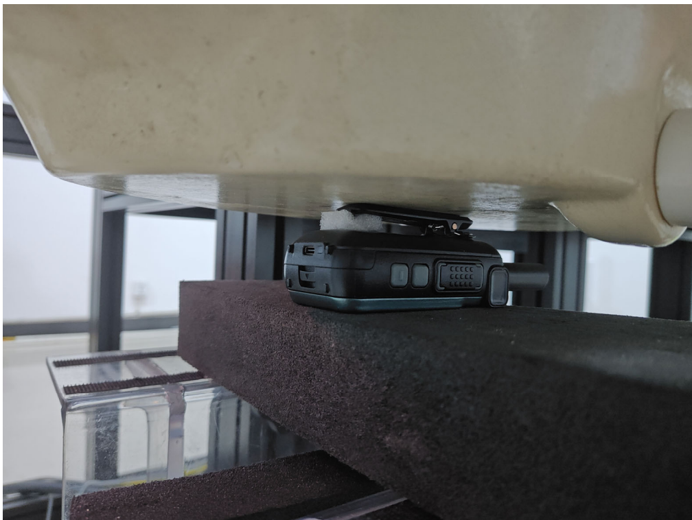
WWAN Body Back with Belt Clip (0mm)
