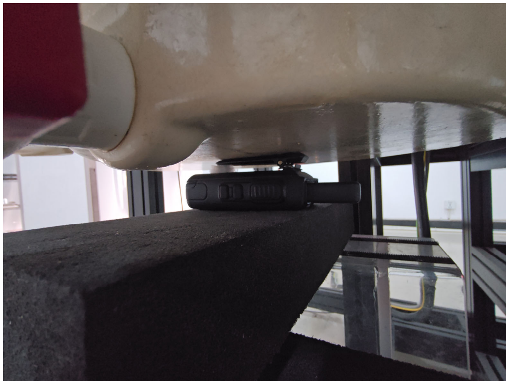
WWAN Body Back with Belt Clip (0mm) —BLT-X115
