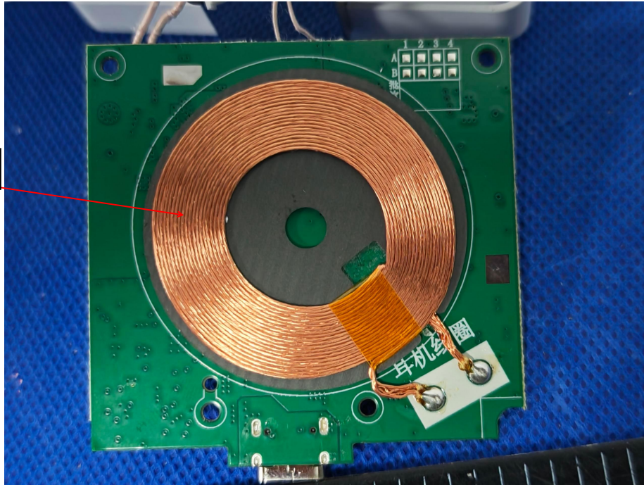
Earphone coil
