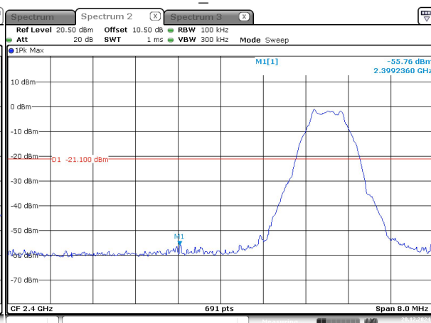
1M_Low -2
