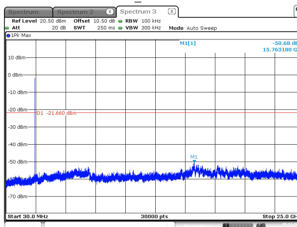
1M_Middle -2
