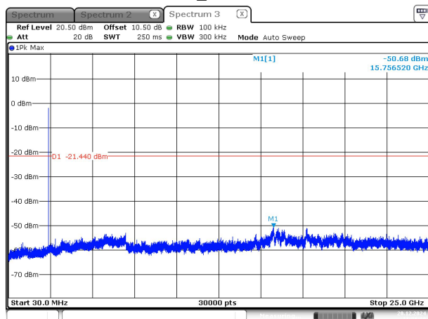
2M_Low -3
