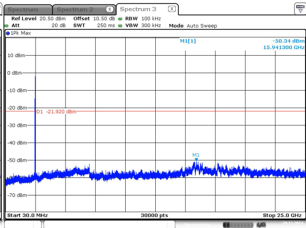
1M_High -3
