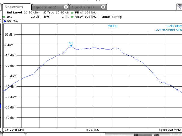
1M_High -1
