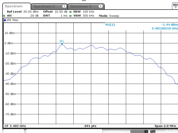
2M_Low -1
