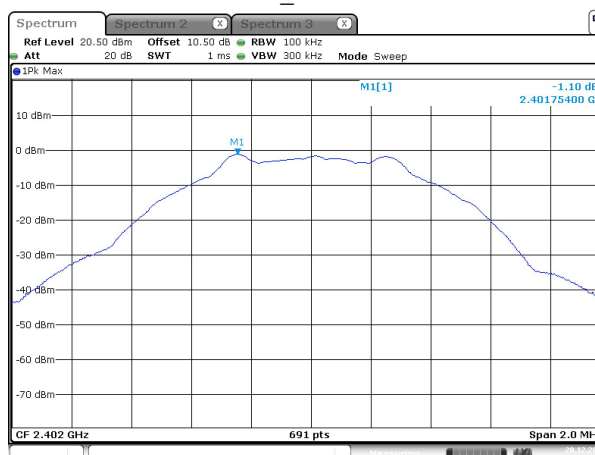
1M_Low -1
