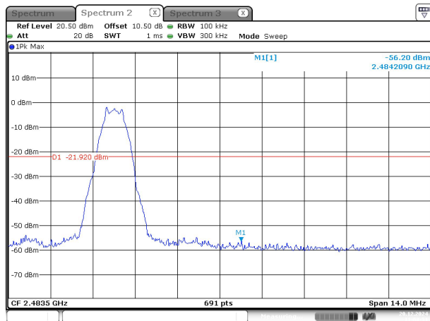
1M_High -2
