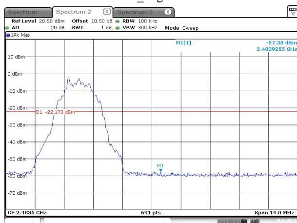
2M_High -2
