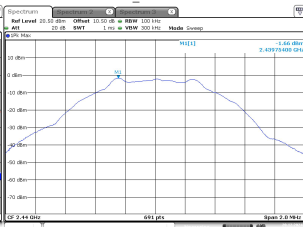
1M_Middle -1
