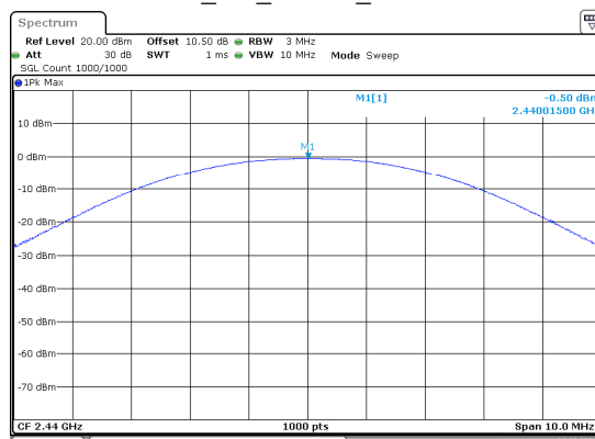
BLE_1M_Middle_Channel
