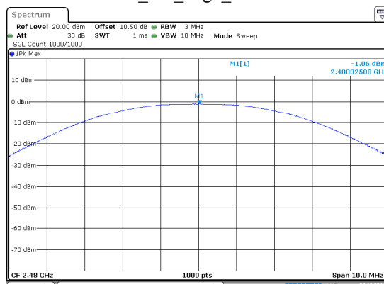
BLE_2M_High_Channel
