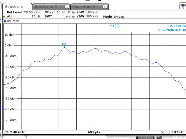
2M_High -1
