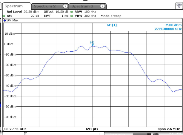
2DH1_Middle -1
