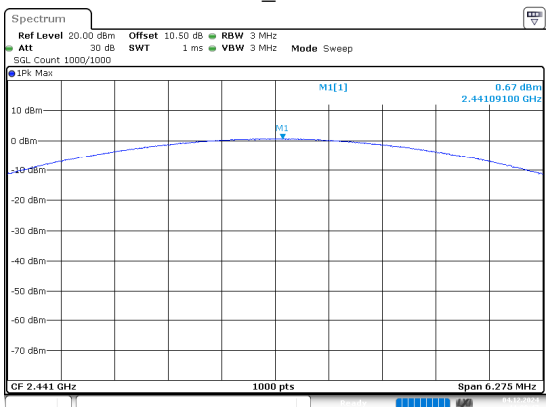
3DH1_Middle
