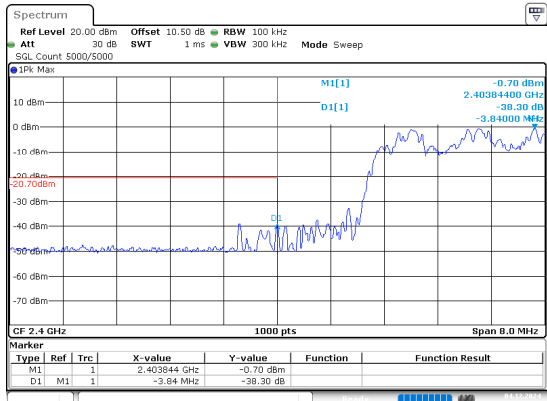
3DH1_Hopping_Lower
