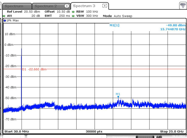
2DH1_High -3
