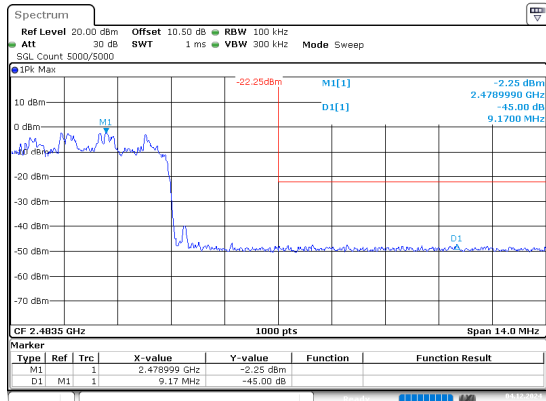
3DH1_Hopping_Upper
