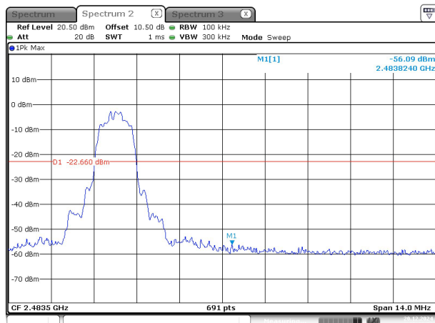
2DH1_High -2
