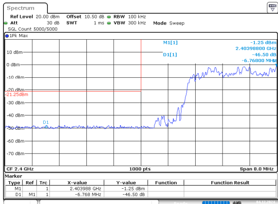
2DH1_Hopping_Lower
