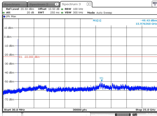
2DH1_Middle -2
