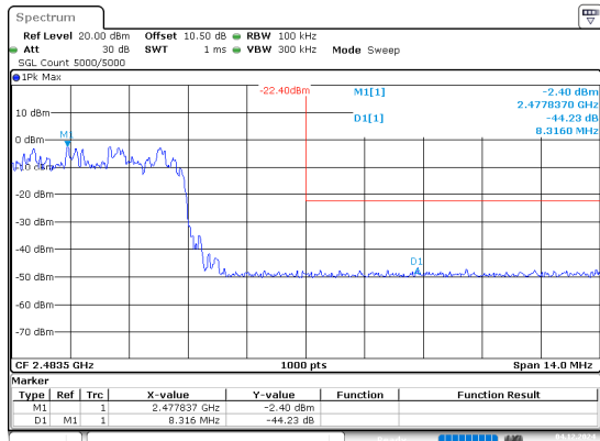
2DH1_Hopping_Upper
