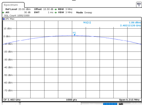
3DH1_Low
