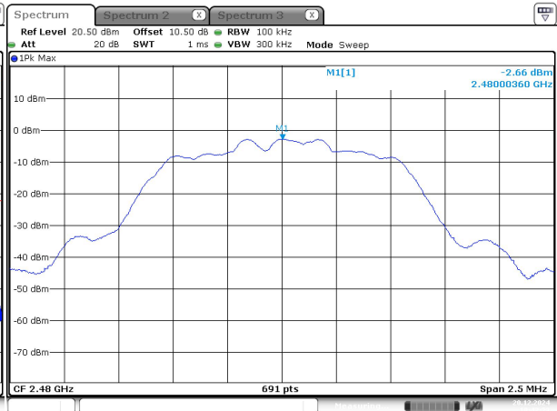
2DH1_High -1
