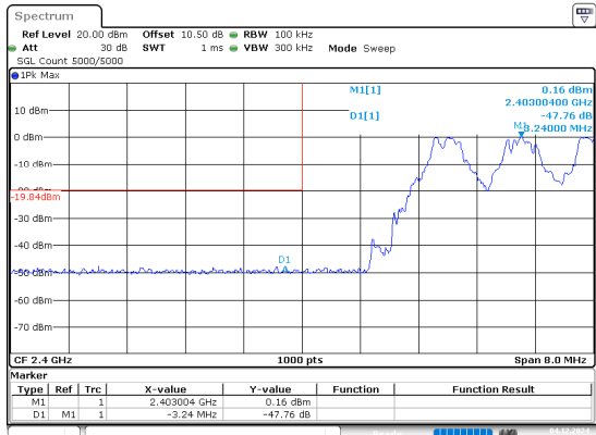
DH1_Hopping_Lower
