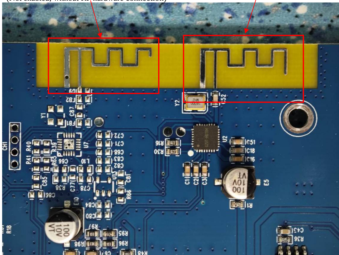
Reserved Antenna (Not enabled, without RF hardware connection)
