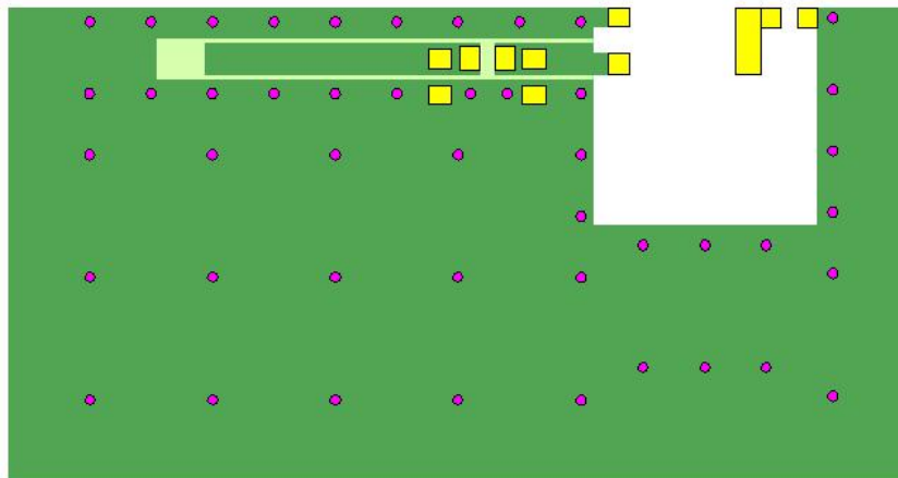
Piercing reference diagram
