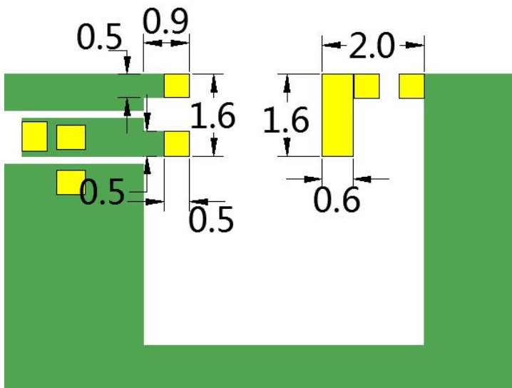
Piercing reference diagram
