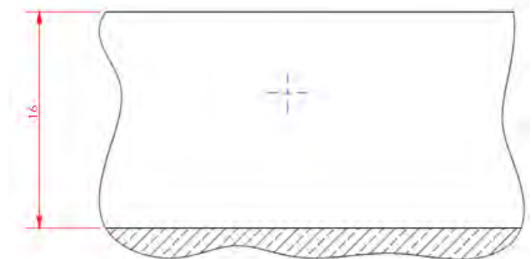
GROUND CLEARANCE BOTTOM VIEW
