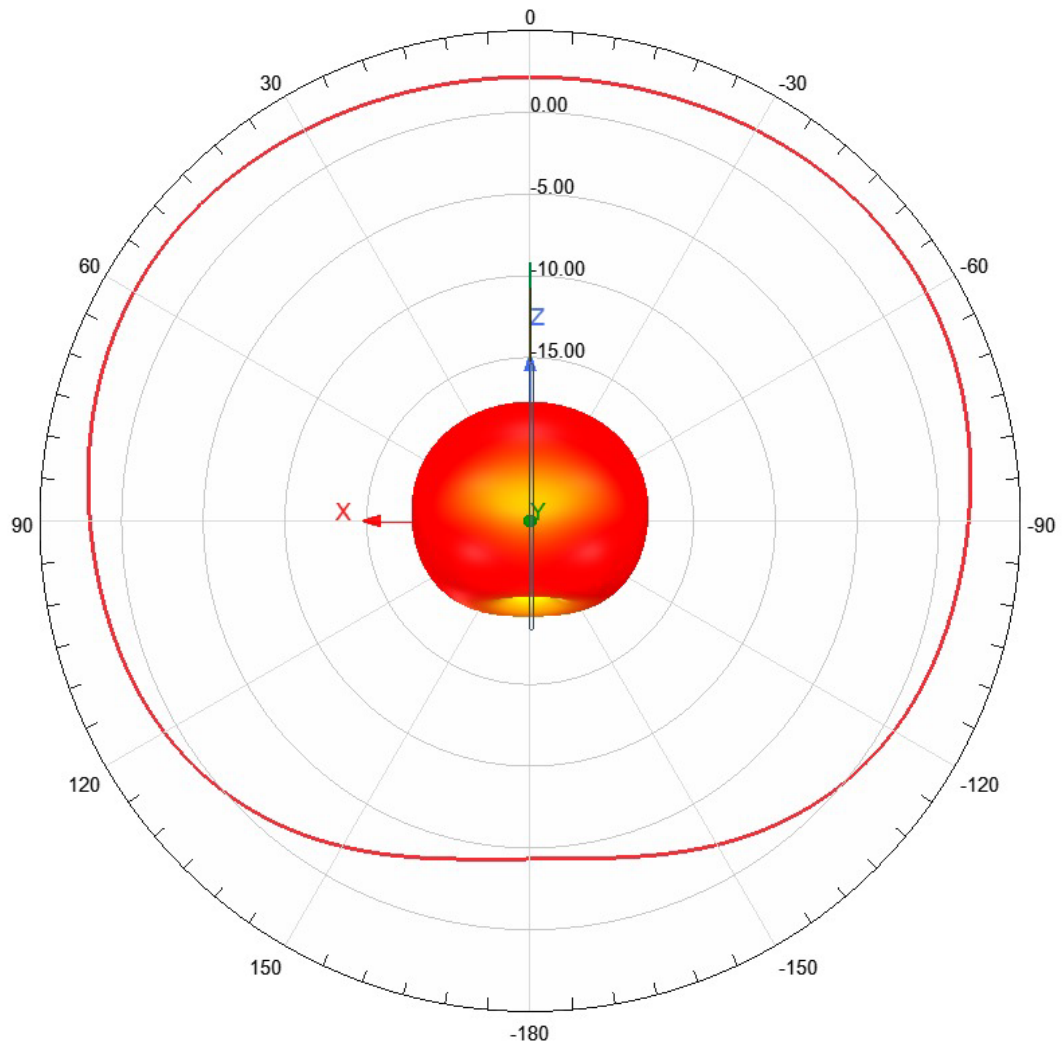
Figure 2- Elevation cut (ZX plane)
