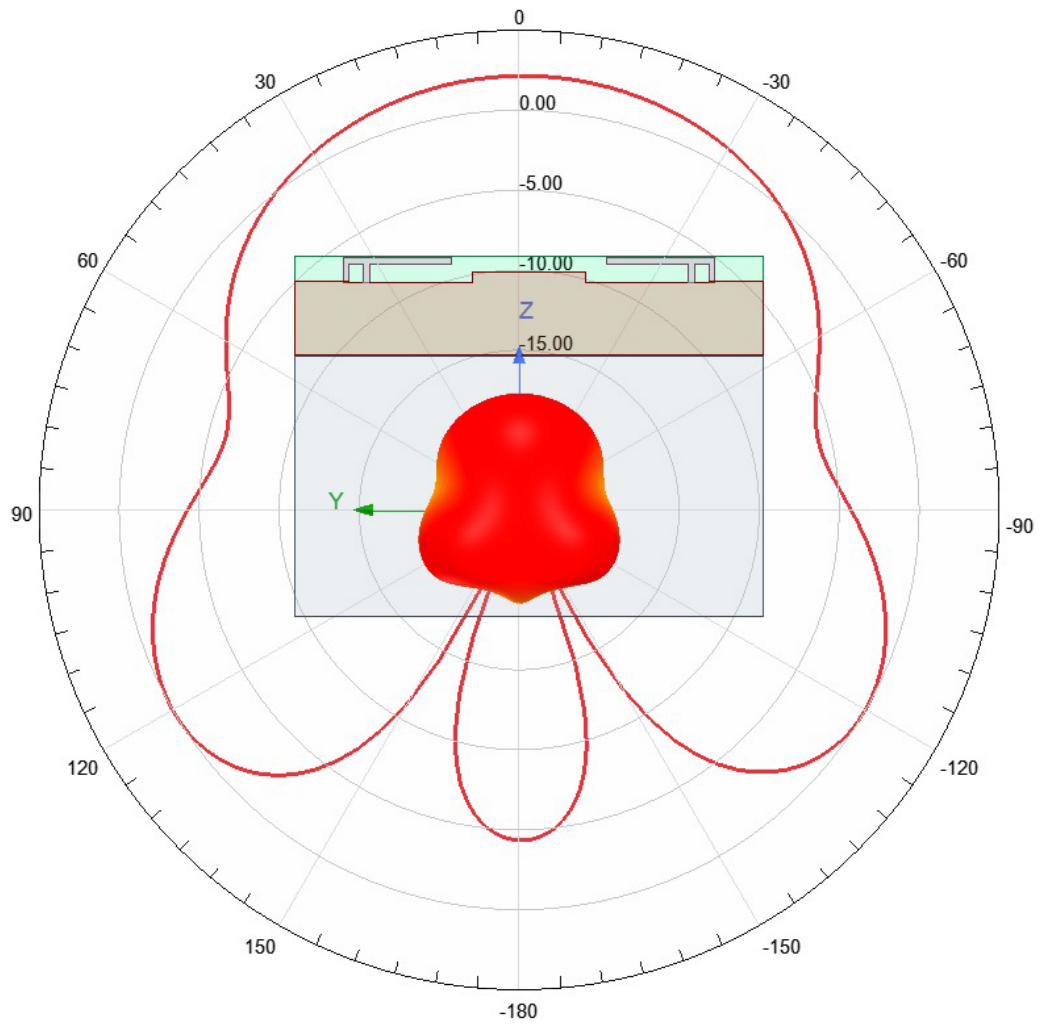
Figure 3- Elevation cut (ZY plane)
