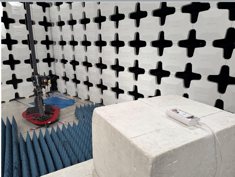
18 GHz – 26 GHz
