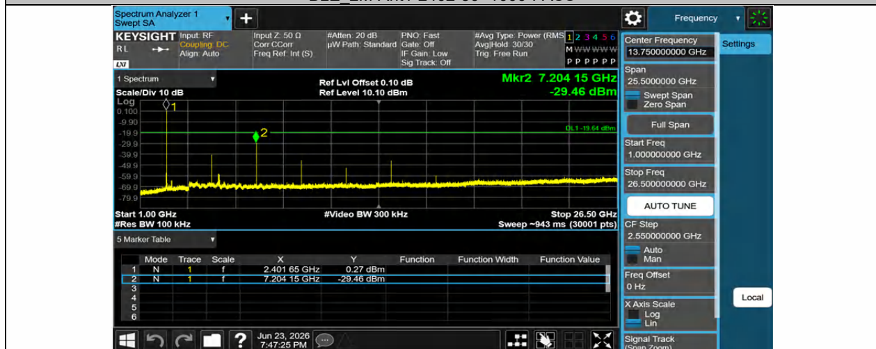
BLE_2M-Ant1-2402-1000~26500-PASS
