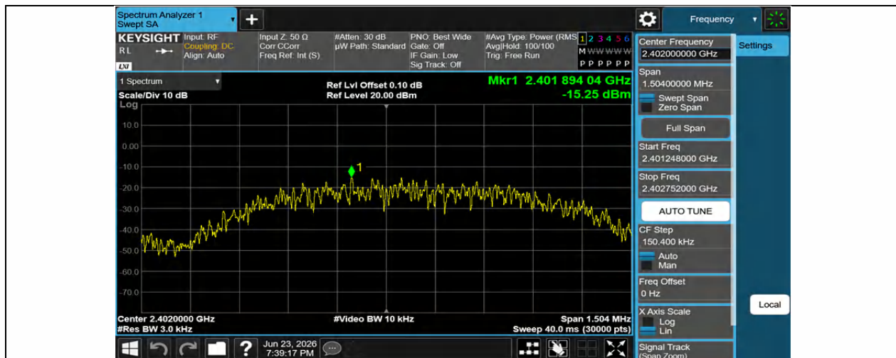
BLE_1M-Ant1-2402-PASS
