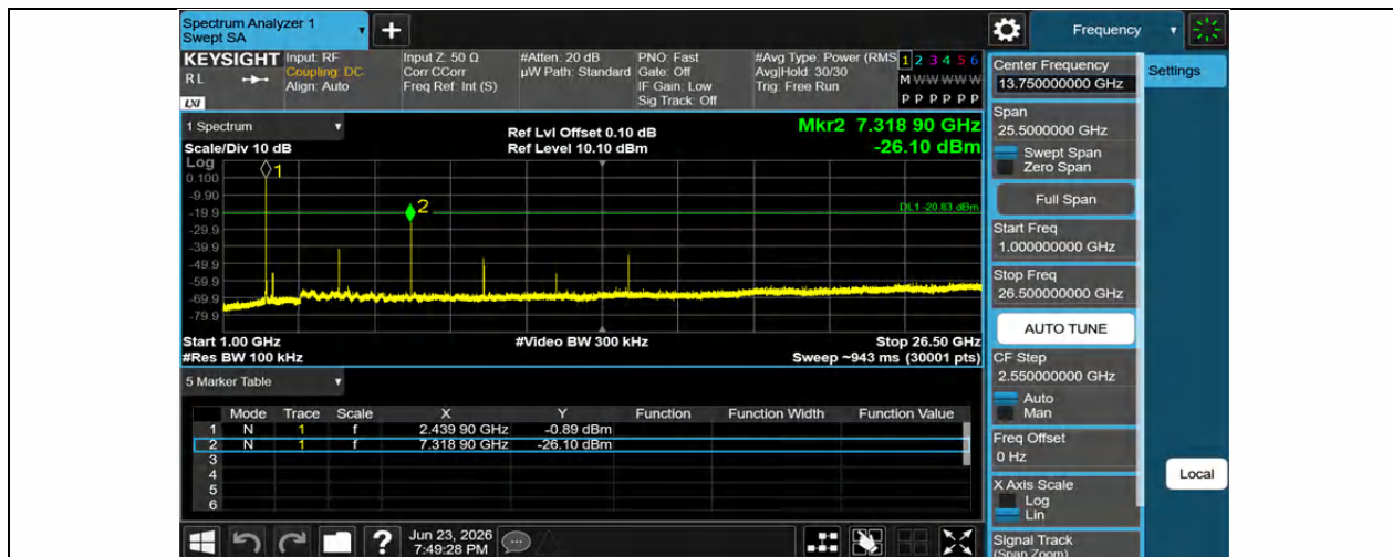
BLE_2M-Ant1-2440-1000~26500-PASS
