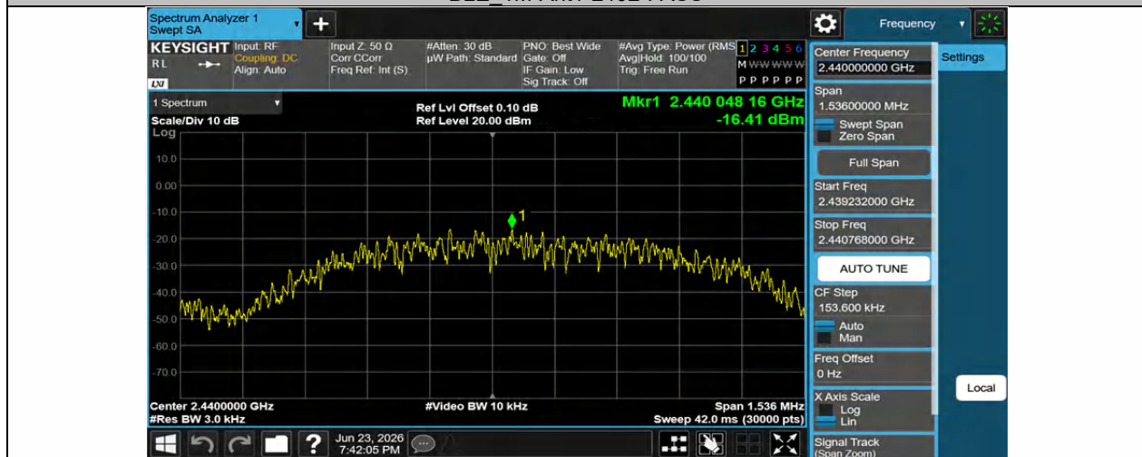
BLE_1M-Ant1-2440-PASS
