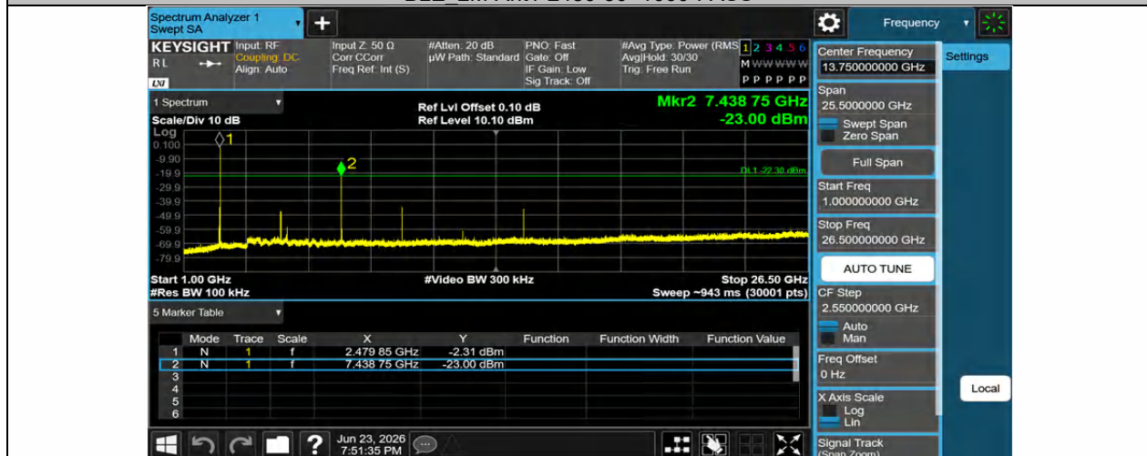
BLE_2M-Ant1-2480-1000~26500-PASS
