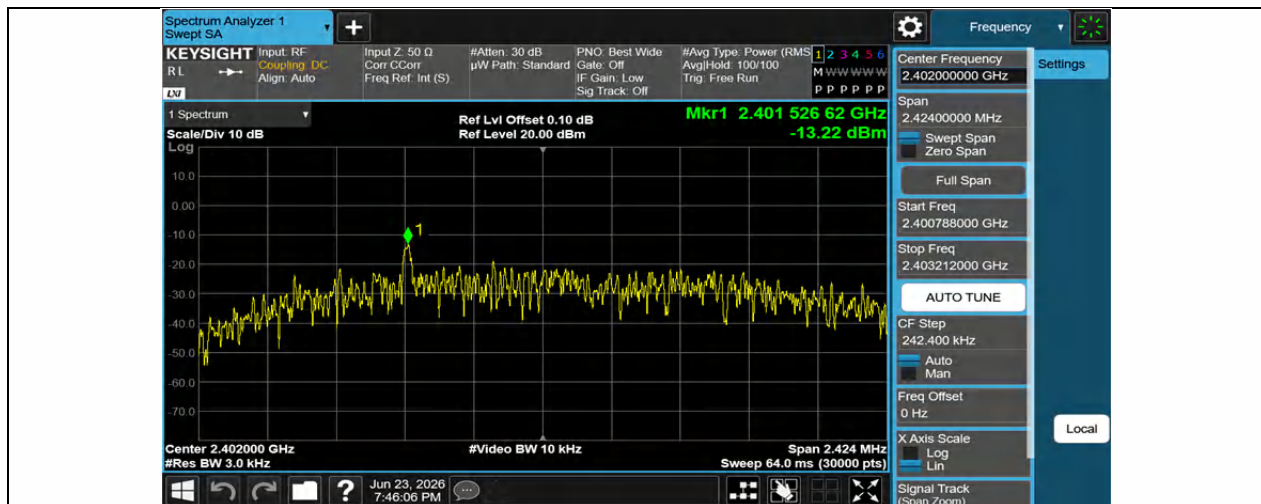
BLE_2M-Ant1-2402-PASS
